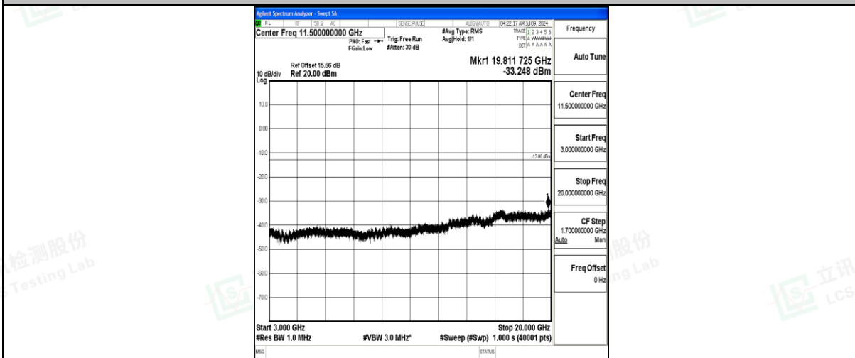
Band25_15MHz_QPSK_26615_1RB#0_3000~20000_3000~20000
