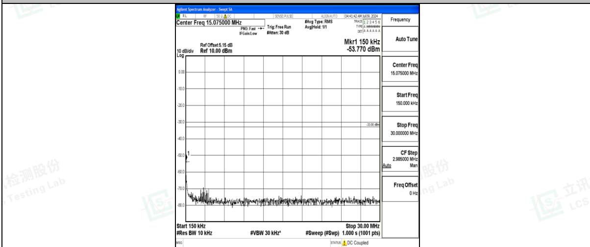
Band25_20MHz_QPSK_26590_1RB#0_0.15~30_0.15~30
