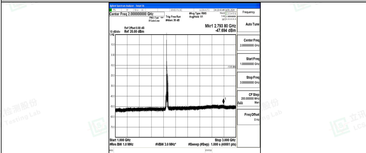
Band25_15MHz_QPSK_26115_1RB#0_1000~3000_1000~3000
