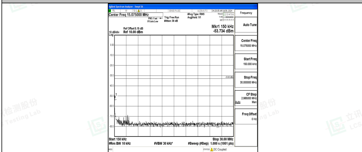
Band25_15MHz_16QAM_26115_1RB#0_0.15~30_0.15~30
