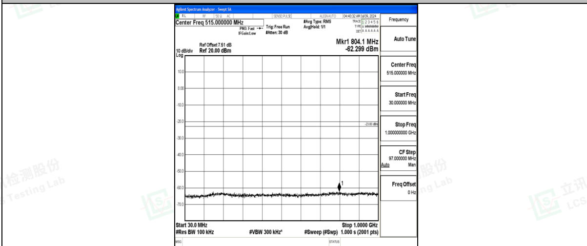
Band25_20MHz_QPSK_26365_1RB#0_30~1000_30~1000
