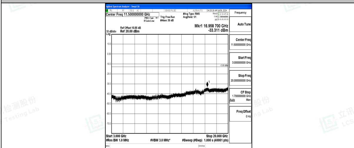
Band25_15MHz_16QAM_26115_1RB#0_3000~20000_3000~20000
