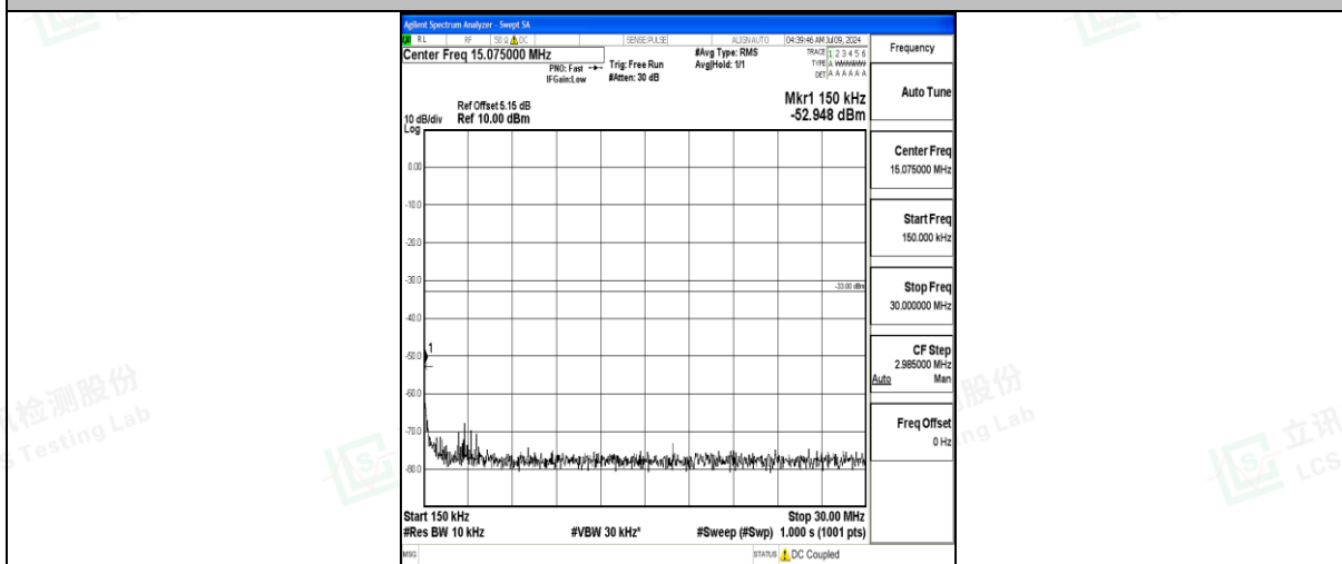
Band25_20MHz_16QAM_26140_1RB#0_0.15~30_0.15~30
