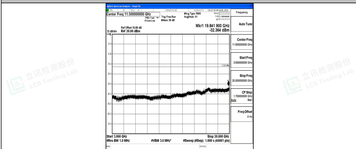
Band25_15MHz_16QAM_26365_1RB#0_3000~20000_3000~20000
