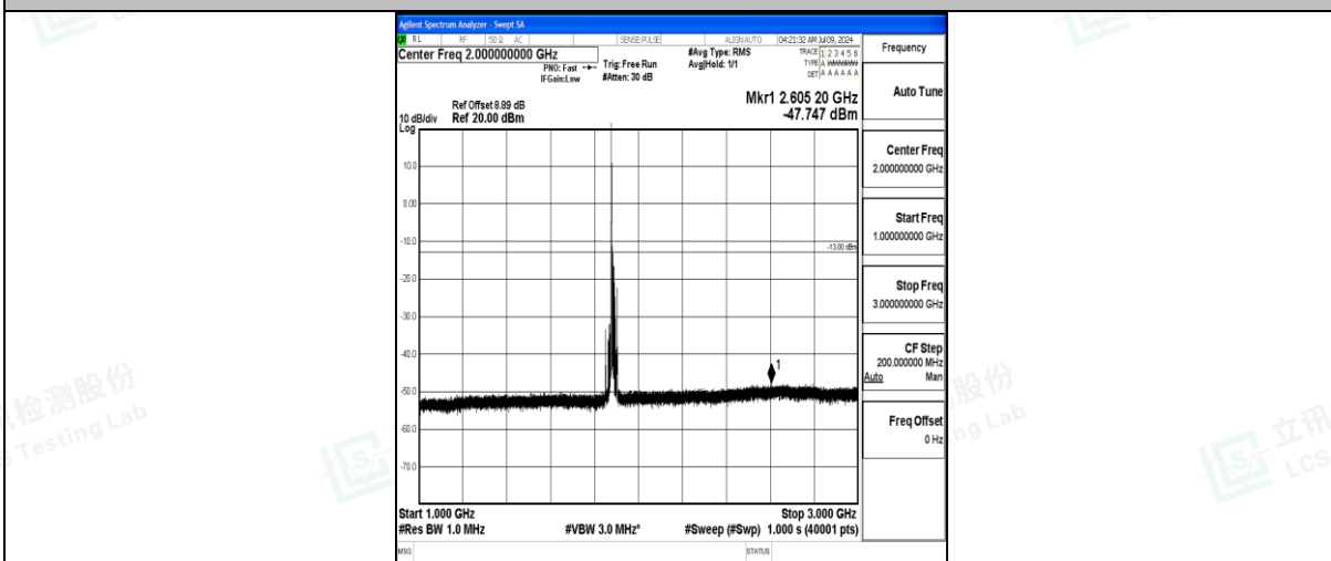
Band25_15MHz_16QAM_26365_1RB#0_1000~3000_1000~3000
