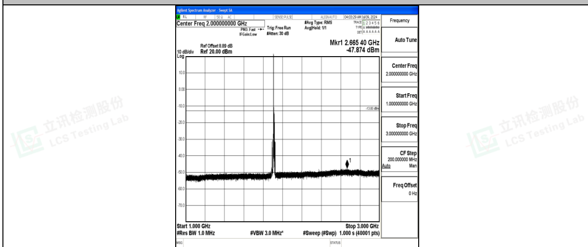
Band25_10MHz_16QAM_26640_1RB#0_1000~3000_1000~3000
