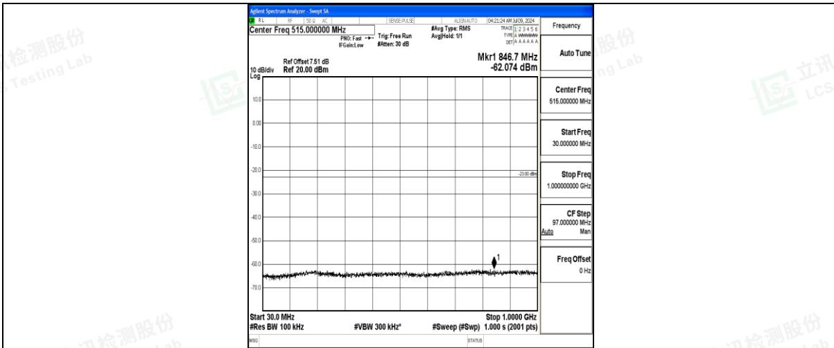
Band25_15MHz_16QAM_26365_1RB#0_30~1000_30~1000
