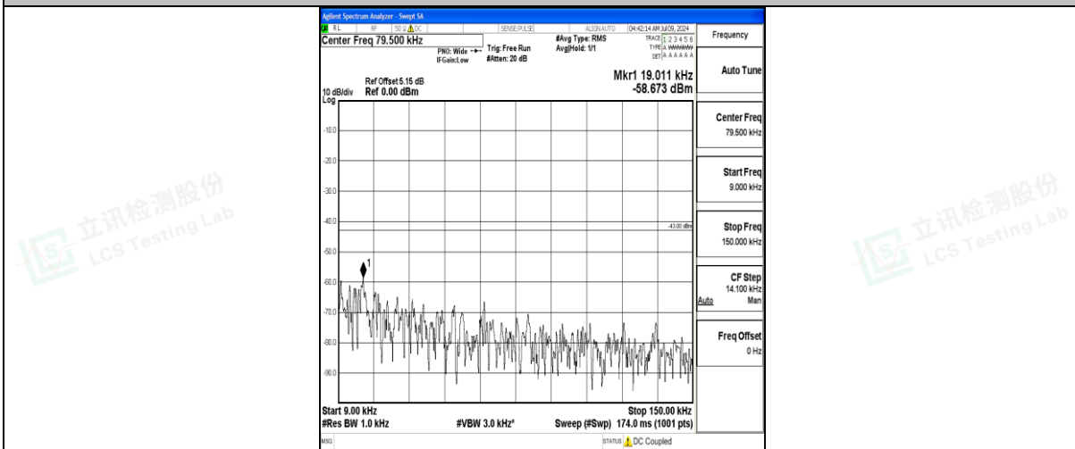
Band25_20MHz_16QAM_26590_1RB#0_0.009~0.15_0.009~0.15
