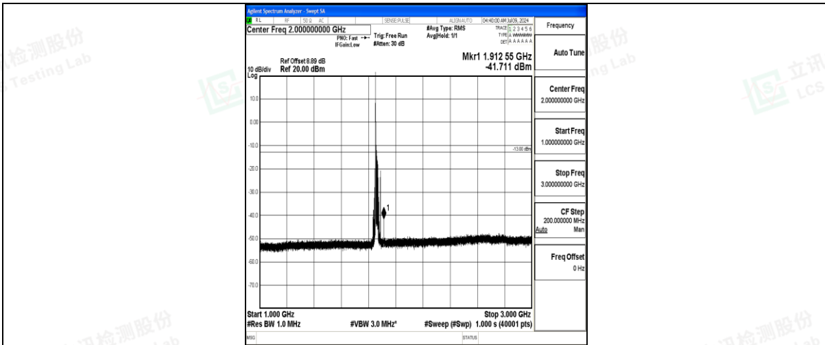
Band25_20MHz_16QAM_26140_1RB#0_1000~3000_1000~3000
