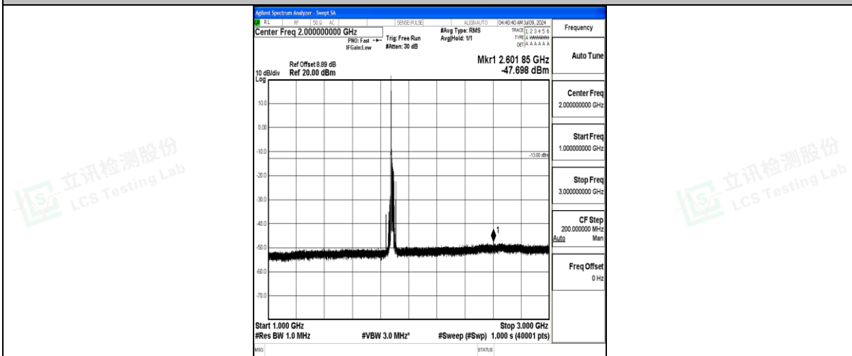
Band25_20MHz_QPSK_26365_1RB#0_1000~3000_1000~3000
