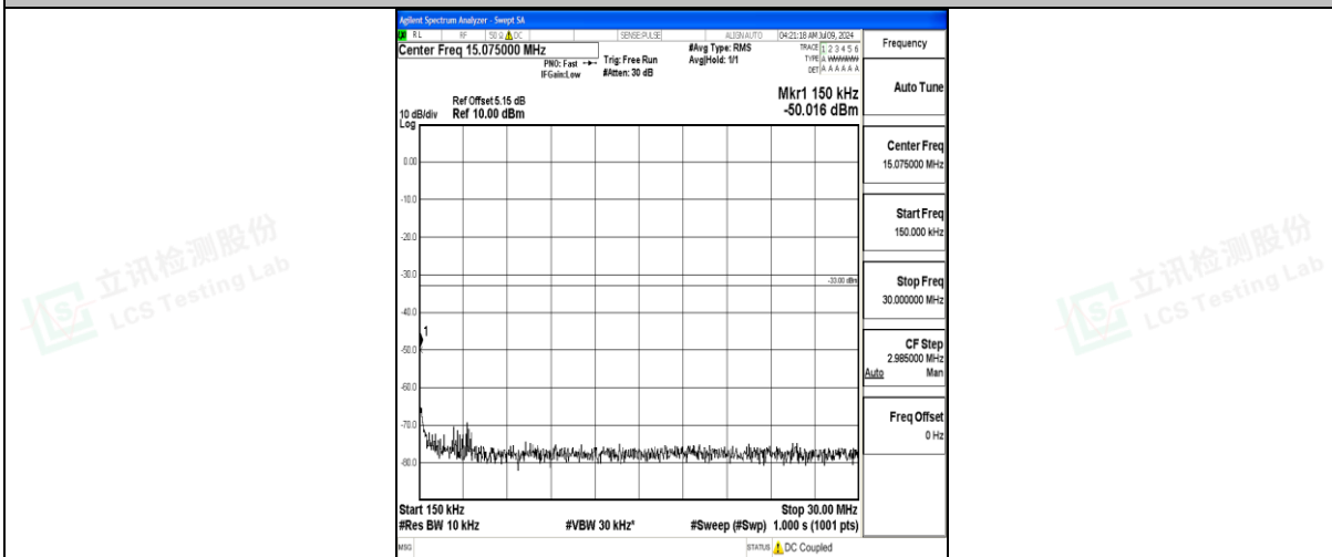
Band25_15MHz_16QAM_26365_1RB#0_0.15~30_0.15~30
