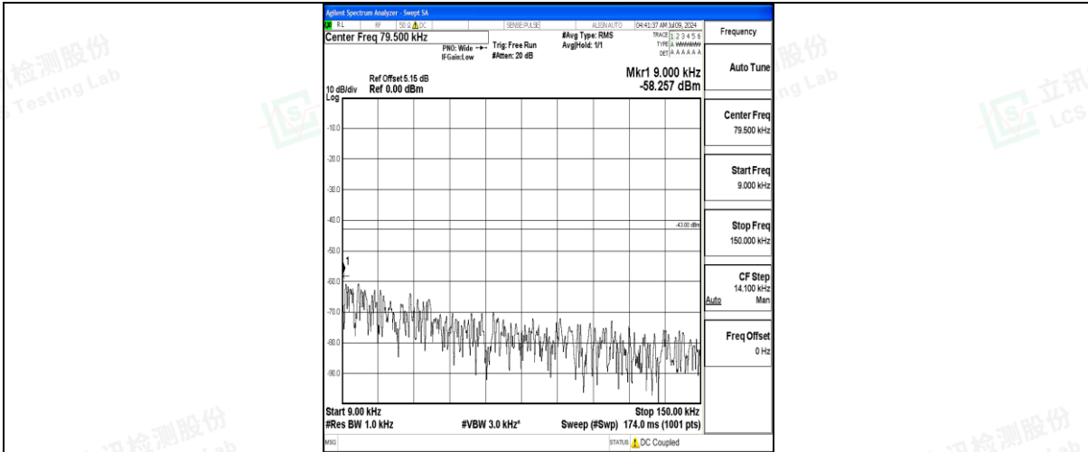
Band25_20MHz_QPSK_26590_1RB#0_0.009~0.15_0.009~0.15
