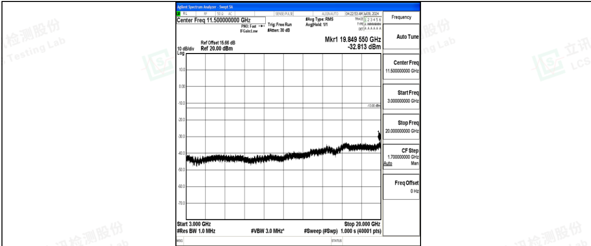
Band25_15MHz_16QAM_26615_1RB#0_3000~20000_3000~20000
