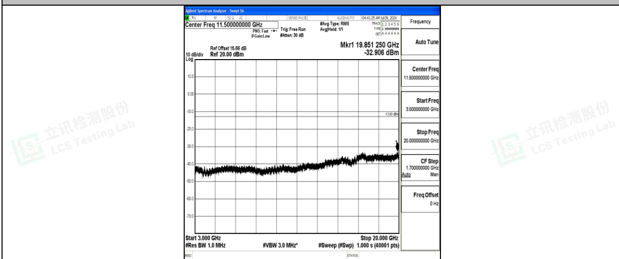
Band25_20MHz_16QAM_26365_1RB#0_3000~20000_3000~20000
