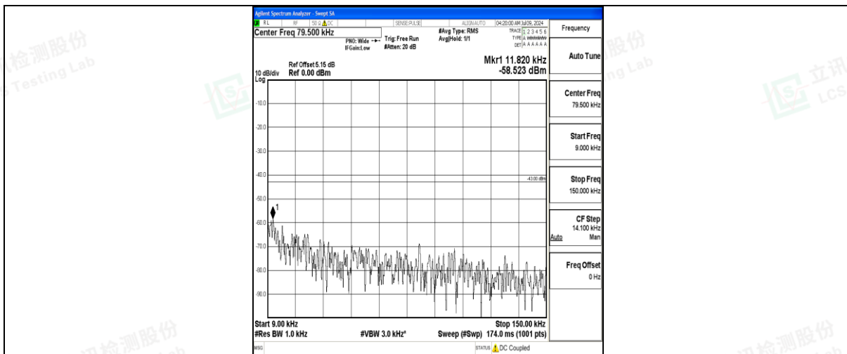
Band25_15MHz_16QAM_26115_1RB#0_0.009~0.15_0.009~0.15
