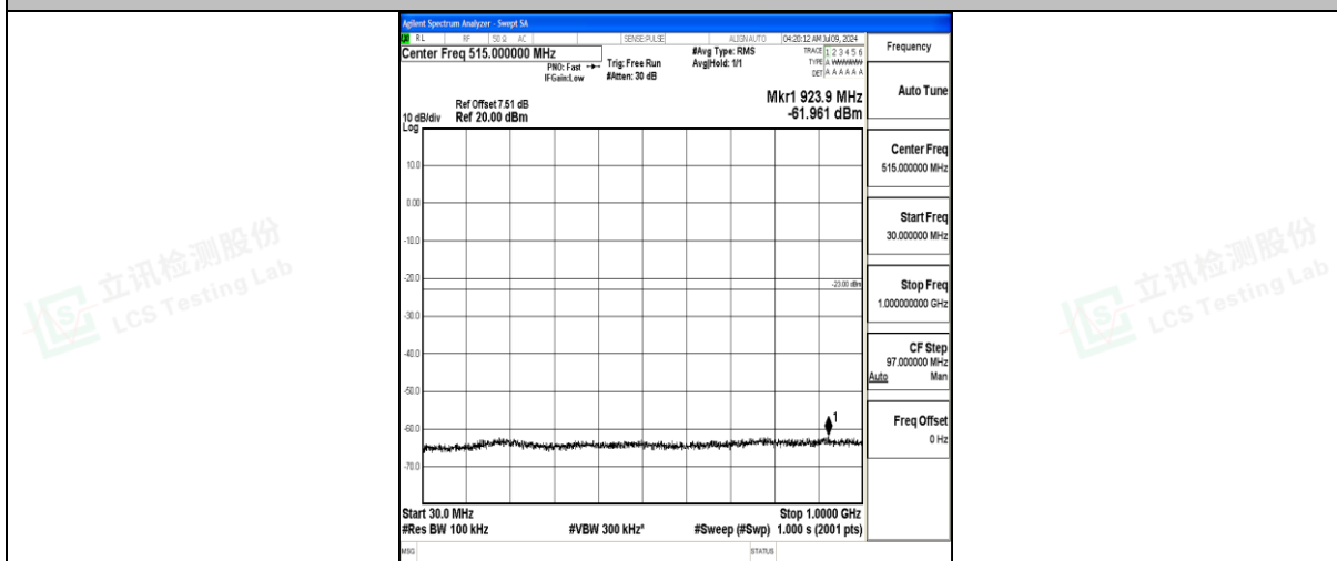
Band25_15MHz_16QAM_26115_1RB#0_30~1000_30~1000
