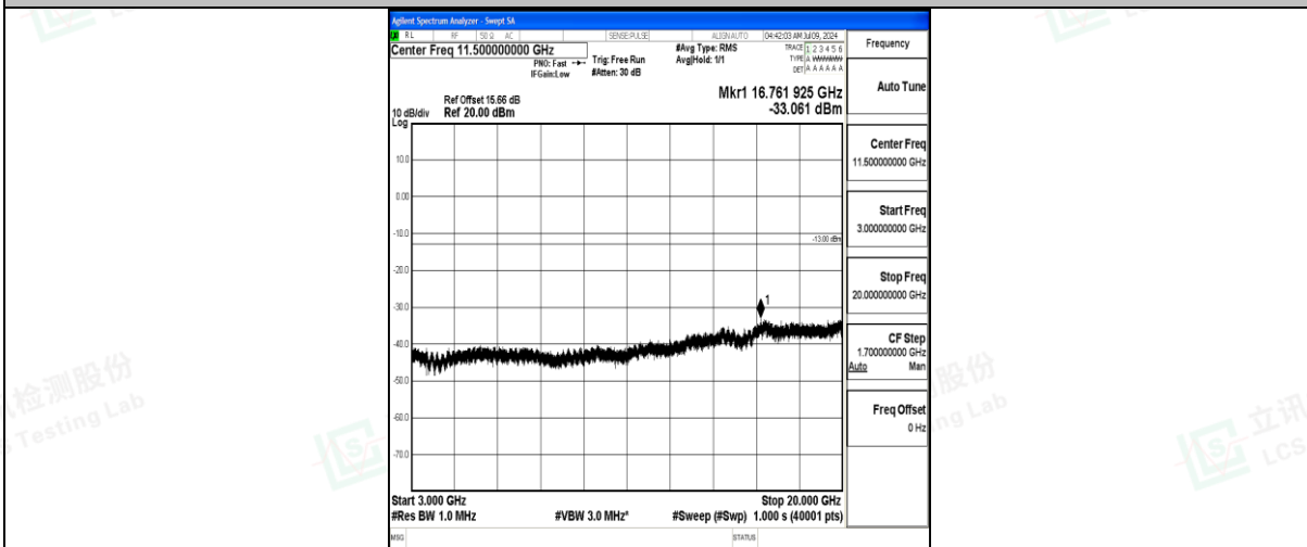
Band25_20MHz_QPSK_26590_1RB#0_3000~20000_3000~20000
