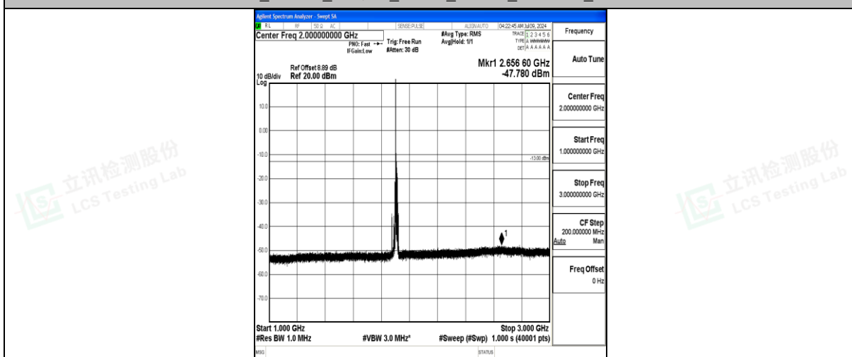
Band25_15MHz_16QAM_26615_1RB#0_1000~3000_1000~3000
