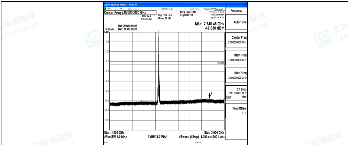
Band25_15MHz_16QAM_26115_1RB#0_1000~3000_1000~3000
