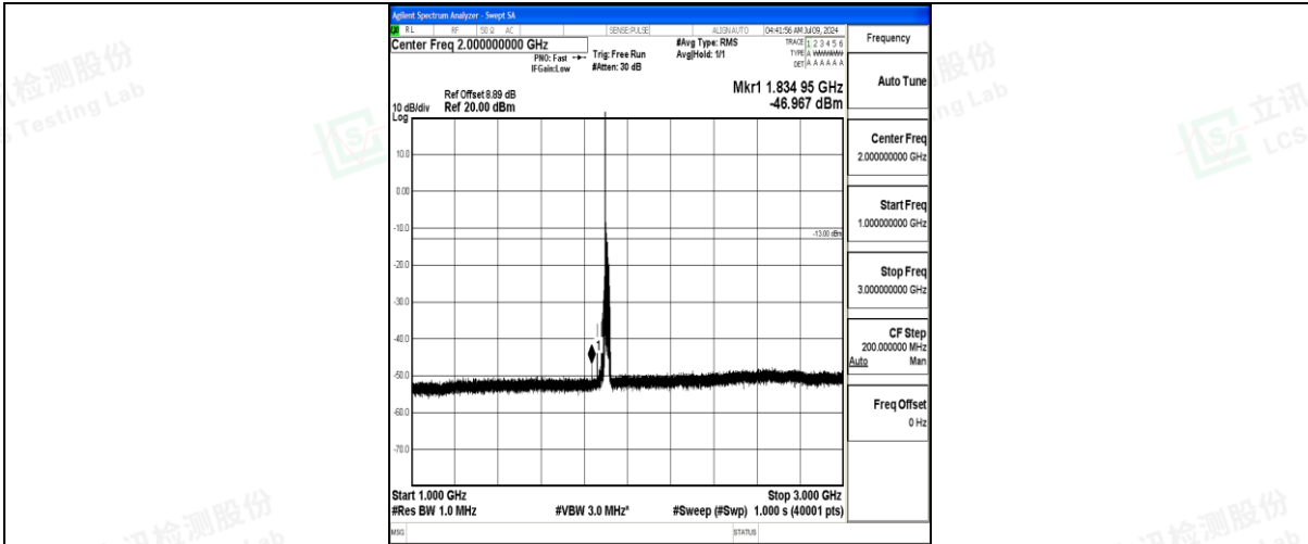
Band25_20MHz_QPSK_26590_1RB#0_1000~3000_1000~3000
