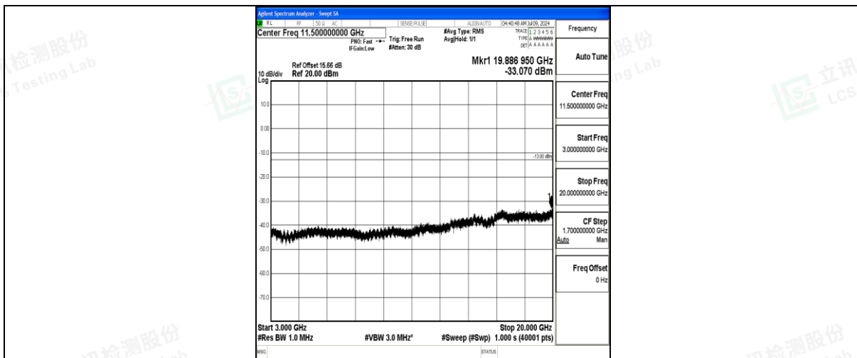
Band25_20MHz_QPSK_26365_1RB#0_3000~20000_3000~20000
