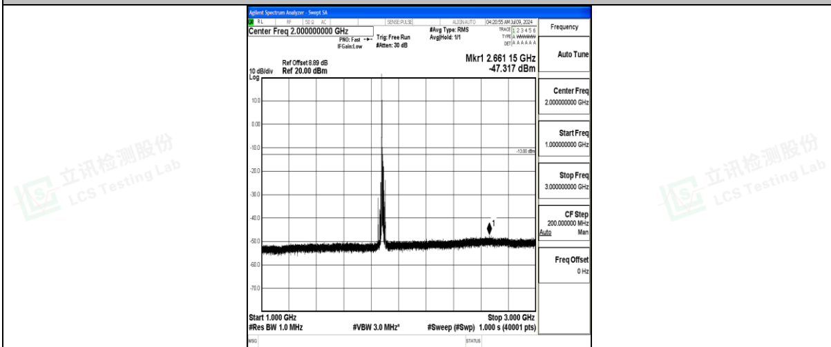
Band25_15MHz_QPSK_26365_1RB#0_1000~3000_1000~3000
