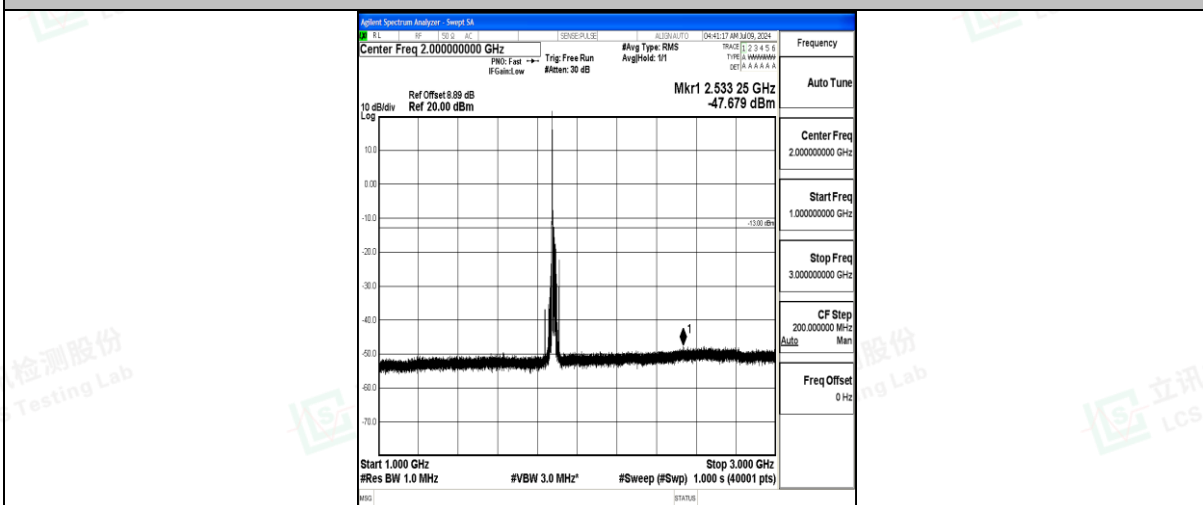
Band25_20MHz_16QAM_26365_1RB#0_1000~3000_1000~3000
