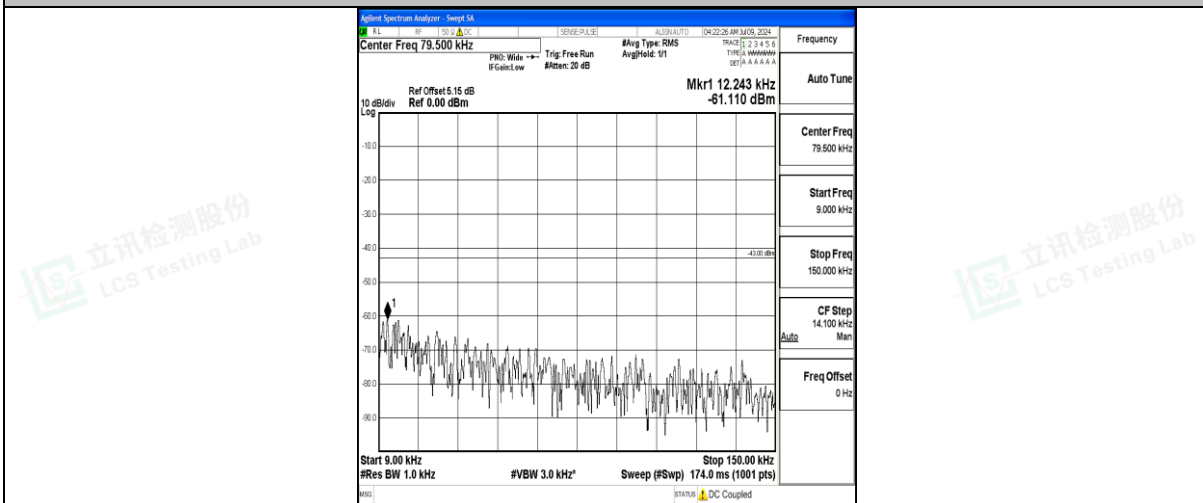
Band25_15MHz_16QAM_26615_1RB#0_0.009~0.15_0.009~0.15
