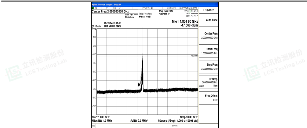
Band25_20MHz_16QAM_26590_1RB#0_1000~3000_1000~3000
