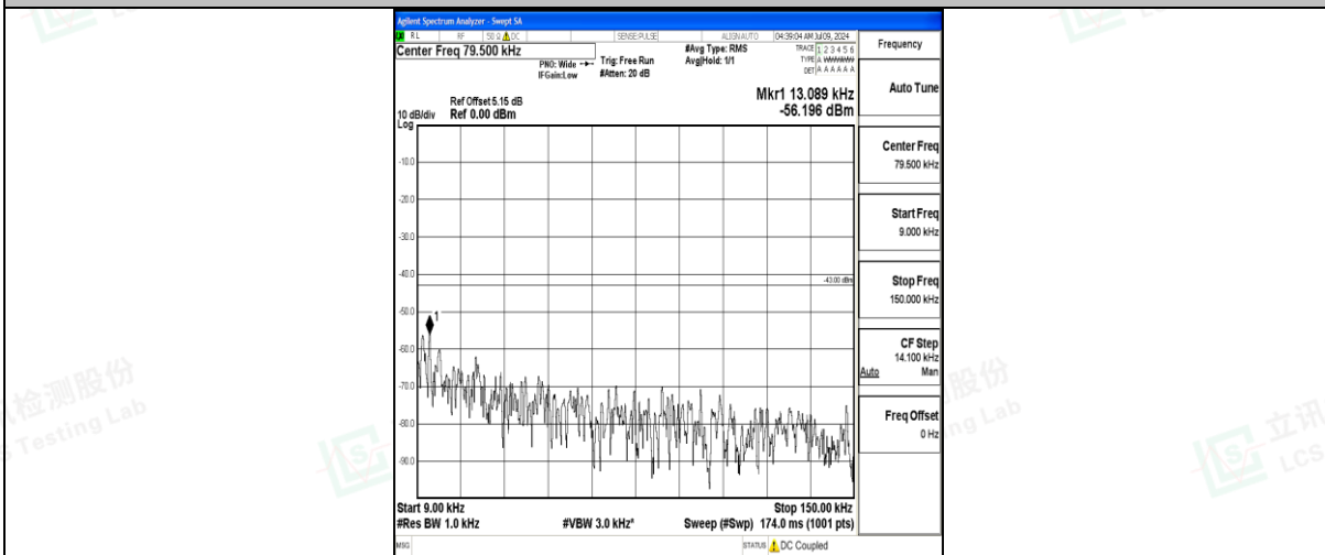
Band25_20MHz_QPSK_26140_1RB#0_0.009~0.15_0.009~0.15
