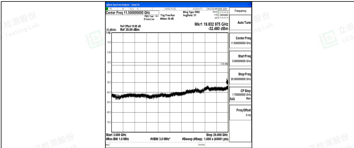
Band25_15MHz_QPSK_26365_1RB#0_3000~20000_3000~20000
