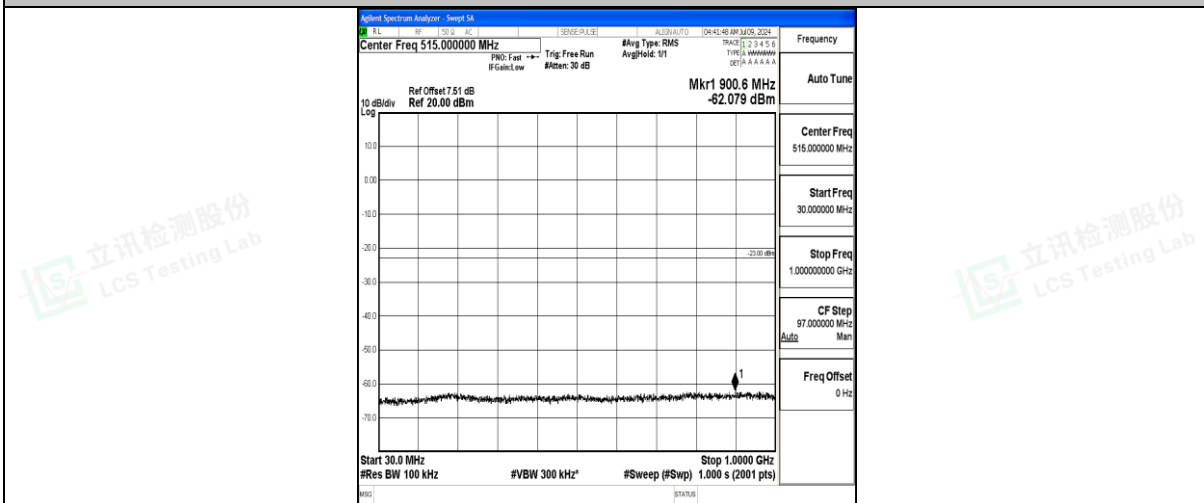
Band25_20MHz_QPSK_26590_1RB#0_30~1000_30~1000
