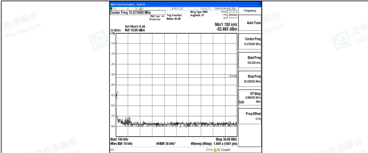
Band25_20MHz_QPSK_26365_1RB#0_0.15~30_0.15~30
