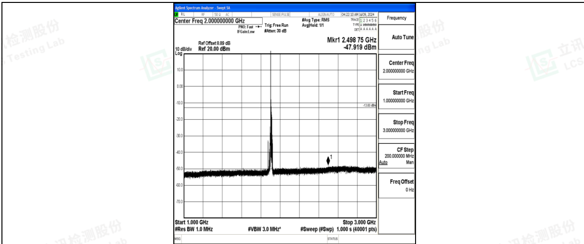
Band25_15MHz_QPSK_26615_1RB#0_1000~3000_1000~3000
