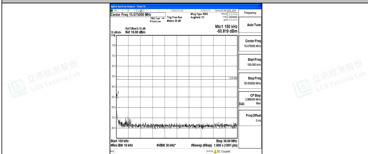
Band25_20MHz_16QAM_26365_1RB#0_0.15~30_0.15~30
