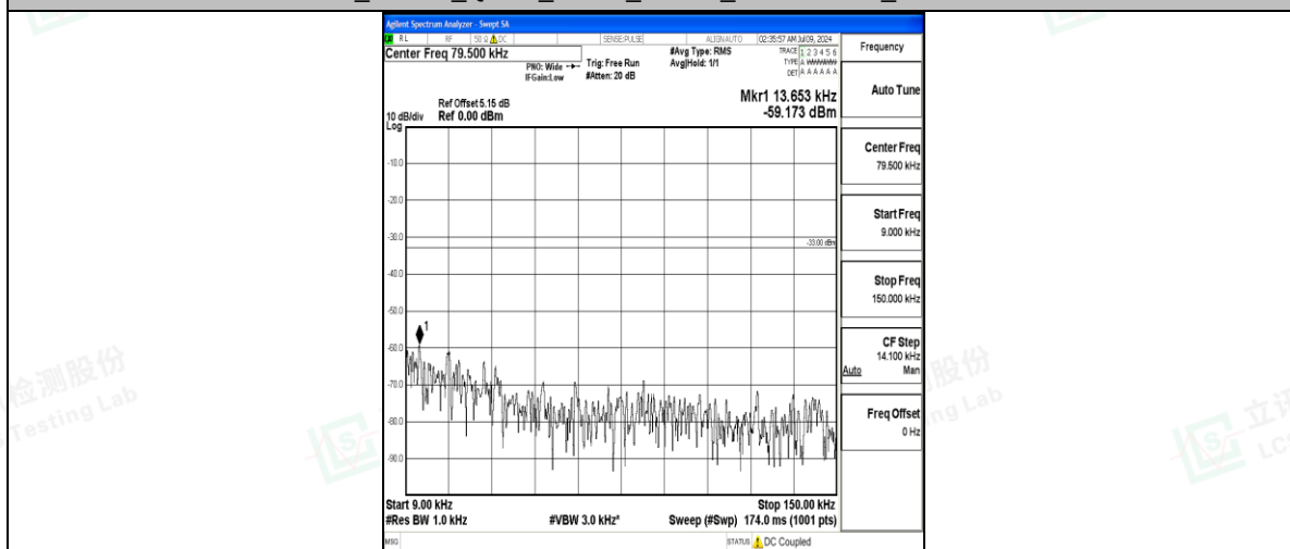
Band17_10MHz_16QAM_23780_1RB#0_0.009~0.15_0.009~0.15
