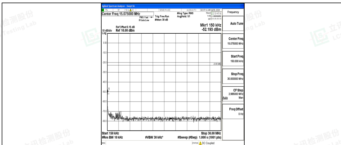
Band17_10MHz_16QAM_23790_1RB#0_0.15~30_0.15~30
