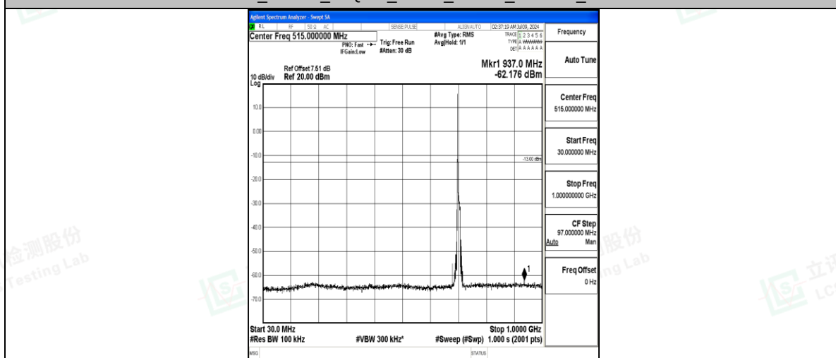
Band17_10MHz_16QAM_23790_1RB#0_30~1000_30~1000
