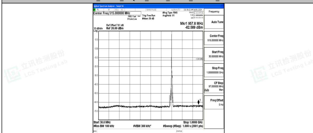
Band17_10MHz_16QAM_23800_1RB#0_30~1000_30~1000
