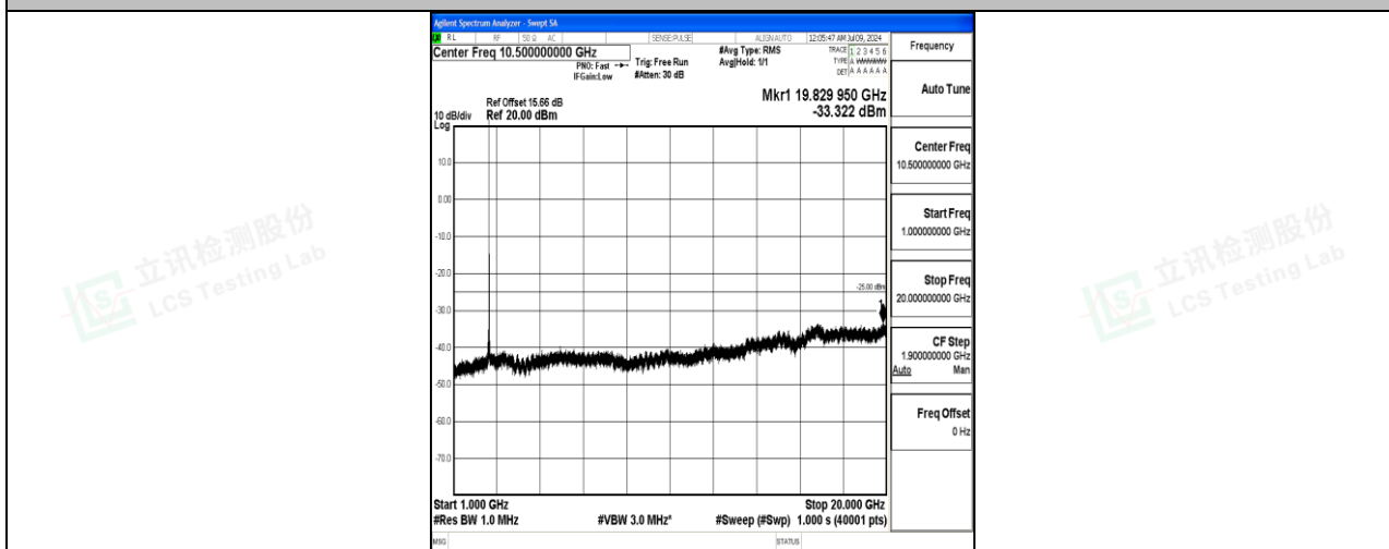
Band7_20MHz_QPSK_21350_1RB#0_1000~20000_1000~20000
