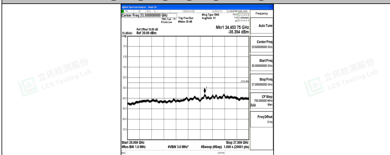
Band7_15MHz_QPSK_21100_1RB#0_20000~27000_20000~27000
