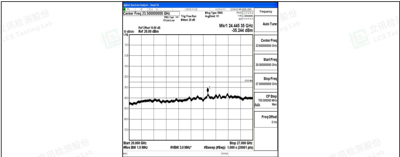
Band7_20MHz_16QAM_20850_1RB#0_20000~27000_20000~27000
