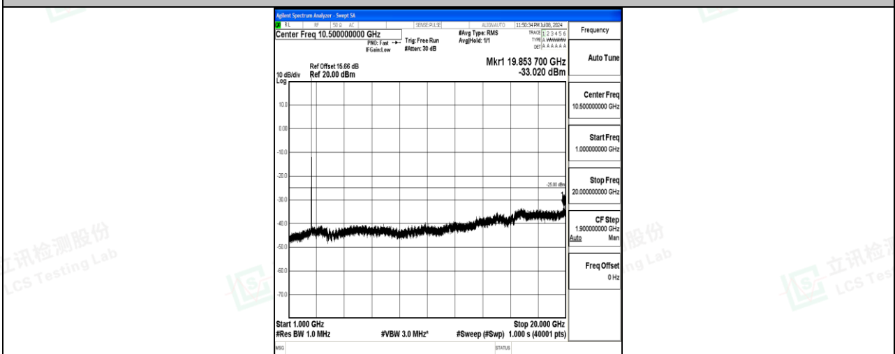
Band7_15MHz_16QAM_21375_1RB#0_1000~20000_1000~20000
