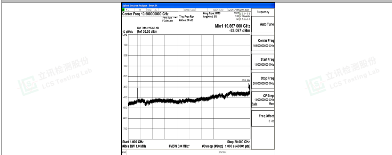
Band7_20MHz_16QAM_20850_1RB#0_1000~20000_1000~20000
