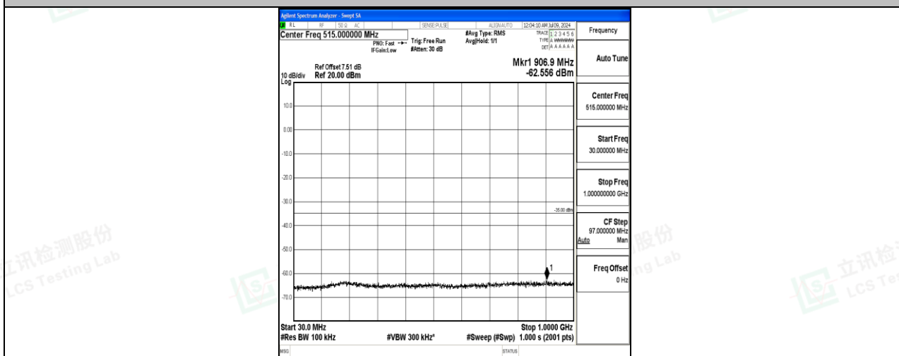
Band7_20MHz_16QAM_20850_1RB#0_30~1000_30~1000
