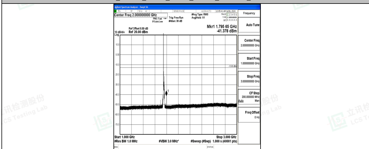
Band4_10MHz_QPSK_20350_1RB#0_1000~3000_1000~3000
