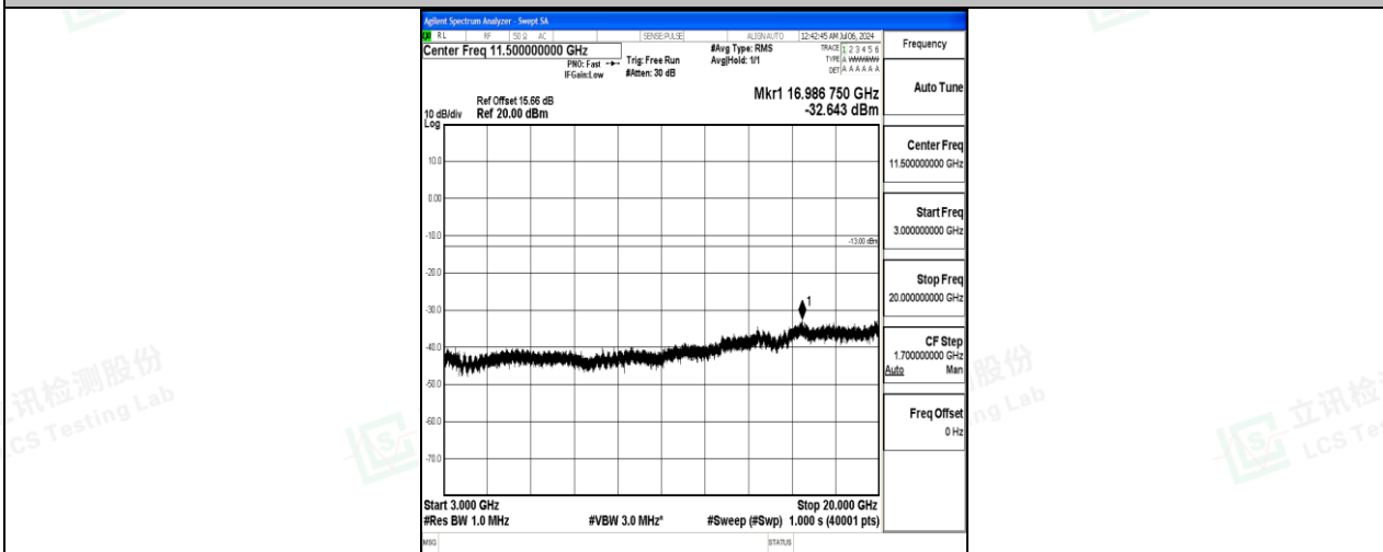
Band4_20MHz_QPSK_20175_1RB#0_3000~20000_3000~20000
