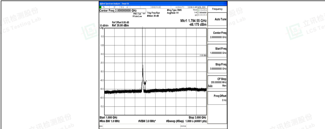
Band4_10MHz_16QAM_20350_1RB#0_1000~3000_1000~3000
