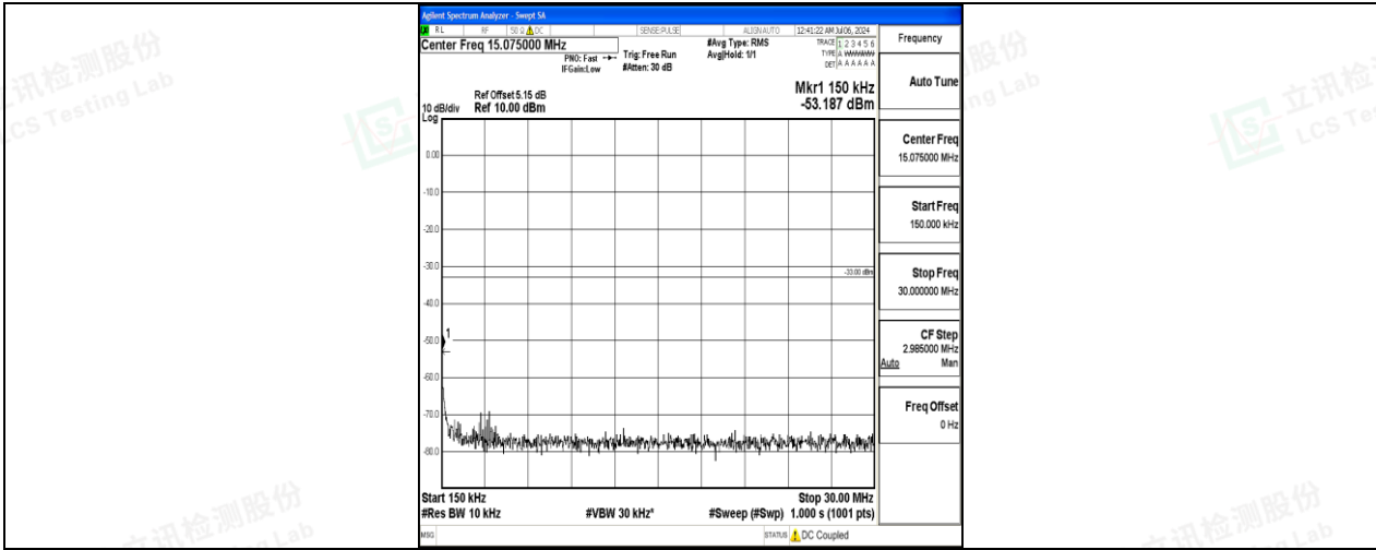
Band4_20MHz_QPSK_20050_1RB#0_0.15~30_0.15~30
