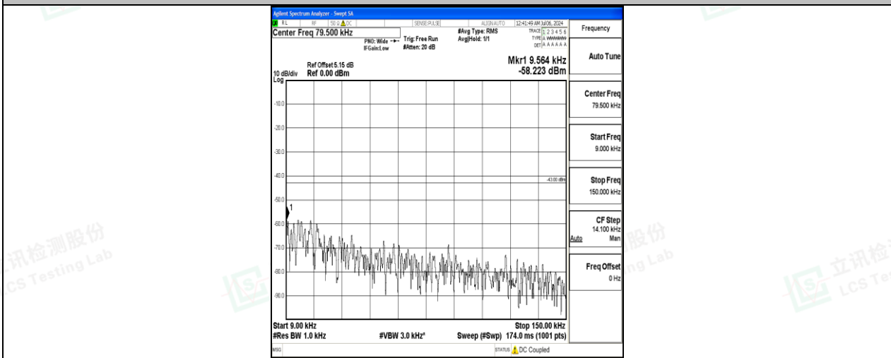
Band4_20MHz_16QAM_20050_1RB#0_0.009~0.15_0.009~0.15
