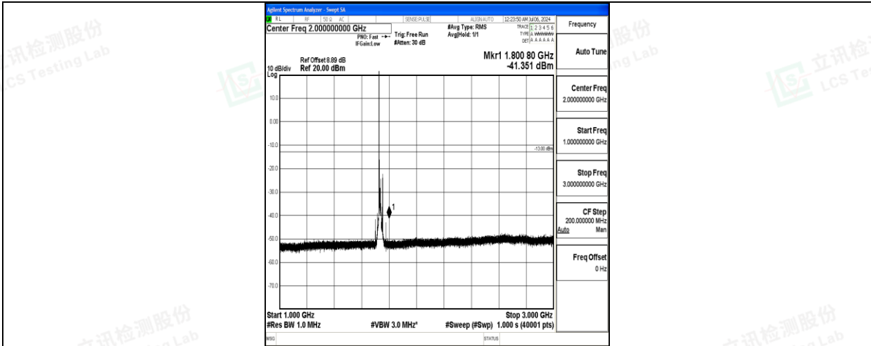
Band4_15MHz_QPSK_20175_1RB#0_1000~3000_1000~3000
