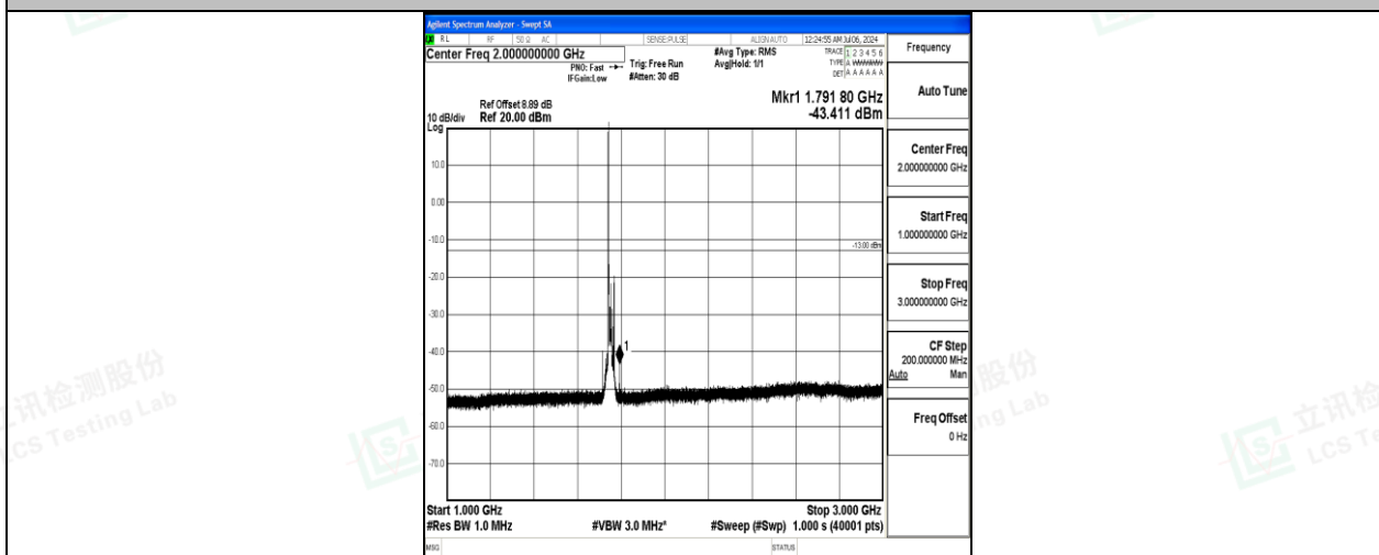
Band4_15MHz_QPSK_20325_1RB#0_1000~3000_1000~3000
