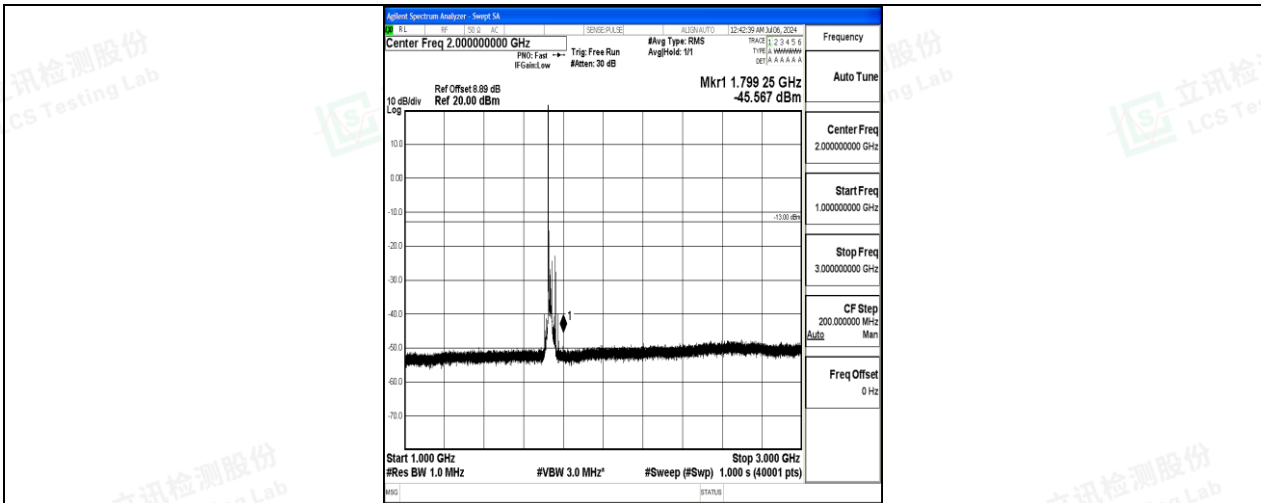
Band4_20MHz_QPSK_20175_1RB#0_1000~3000_1000~3000
