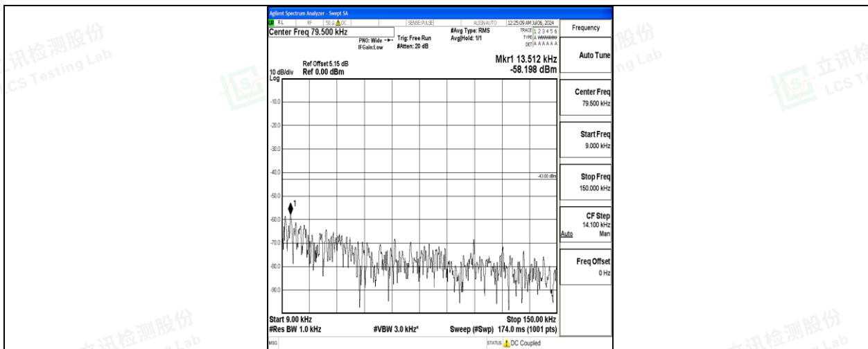
Band4_15MHz_16QAM_20325_1RB#0_0.009~0.15_0.009~0.15
