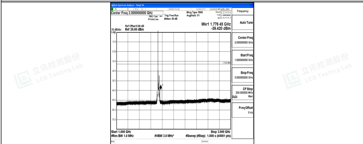
Band4_15MHz_16QAM_20175_1RB#0_1000~3000_1000~3000
