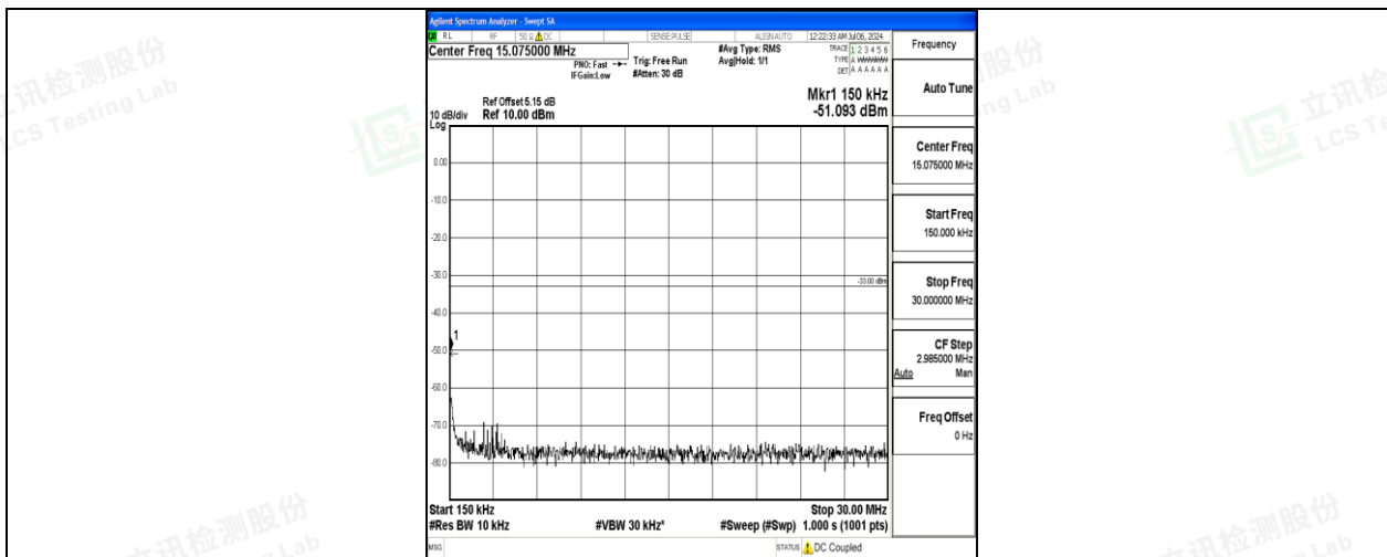
Band4_15MHz_QPSK_20025_1RB#0_0.15~30_0.15~30
