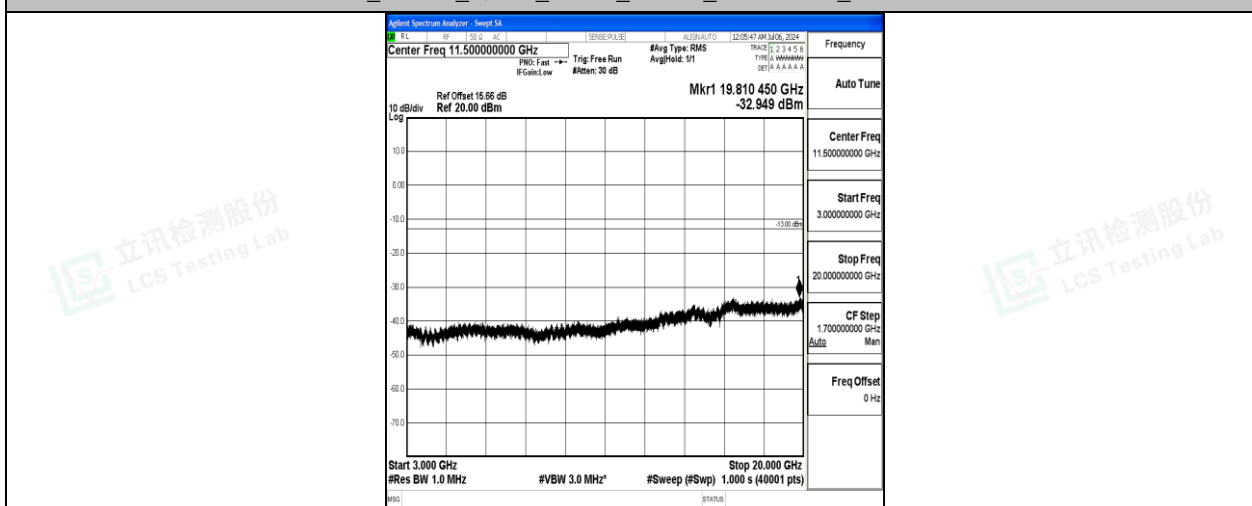
Band4_10MHz_QPSK_20350_1RB#0_3000~20000_3000~20000
