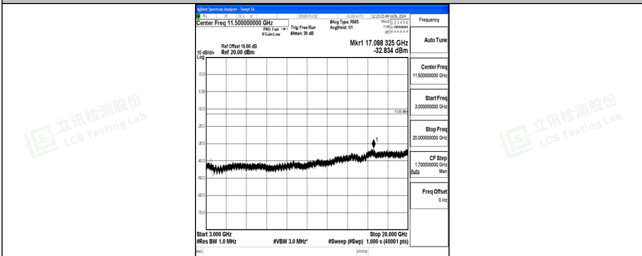
Band4_15MHz_16QAM_20025_1RB#0_3000~20000_3000~20000
