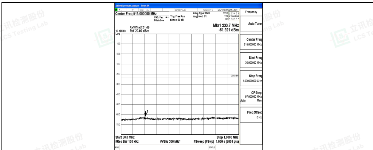
Band4_15MHz_QPSK_20325_1RB#0_30~1000_30~1000
