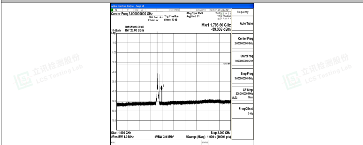
Band4_20MHz_QPSK_20050_1RB#0_1000~3000_1000~3000
