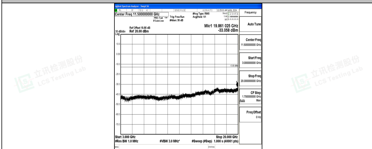
Band4_15MHz_QPSK_20325_1RB#0_3000~20000_3000~20000
