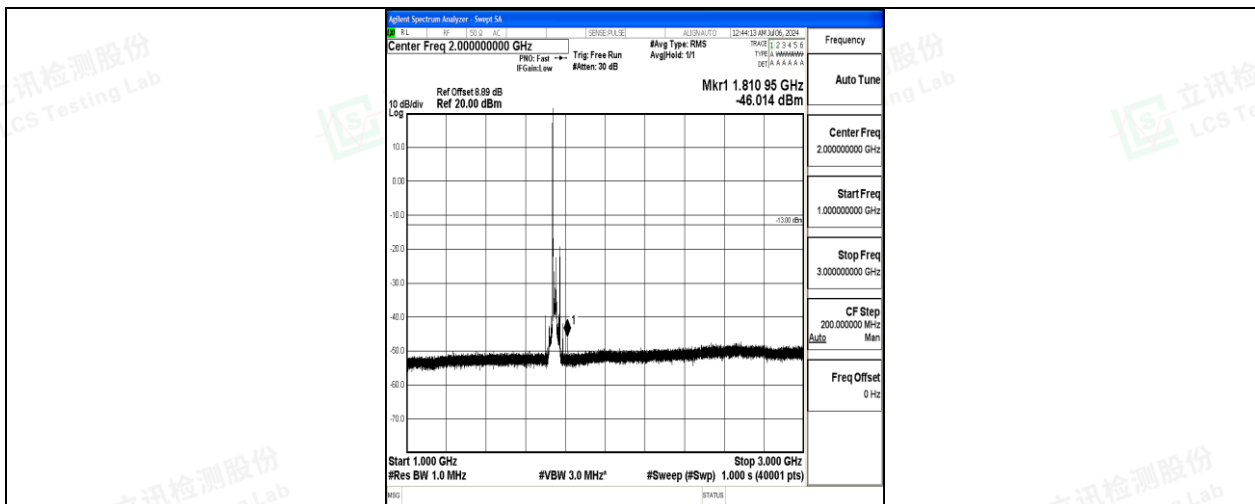
Band4_20MHz_16QAM_20300_1RB#0_1000~3000_1000~3000
