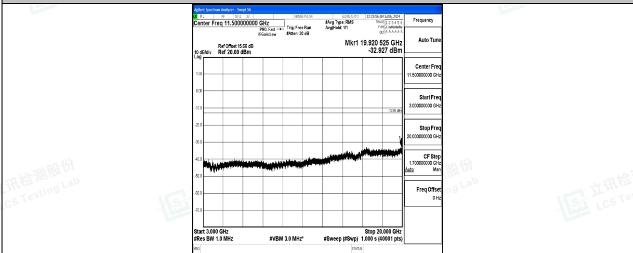
Band4_15MHz_QPSK_20175_1RB#0_3000~20000_3000~20000
