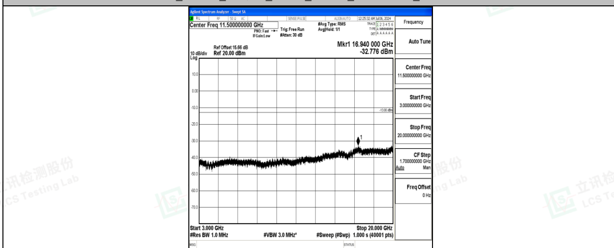
Band4_15MHz_16QAM_20325_1RB#0_3000~20000_3000~20000
