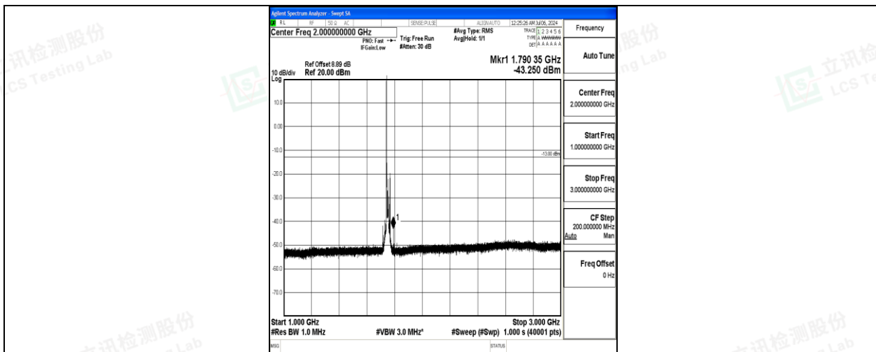
Band4_15MHz_16QAM_20325_1RB#0_1000~3000_1000~3000
