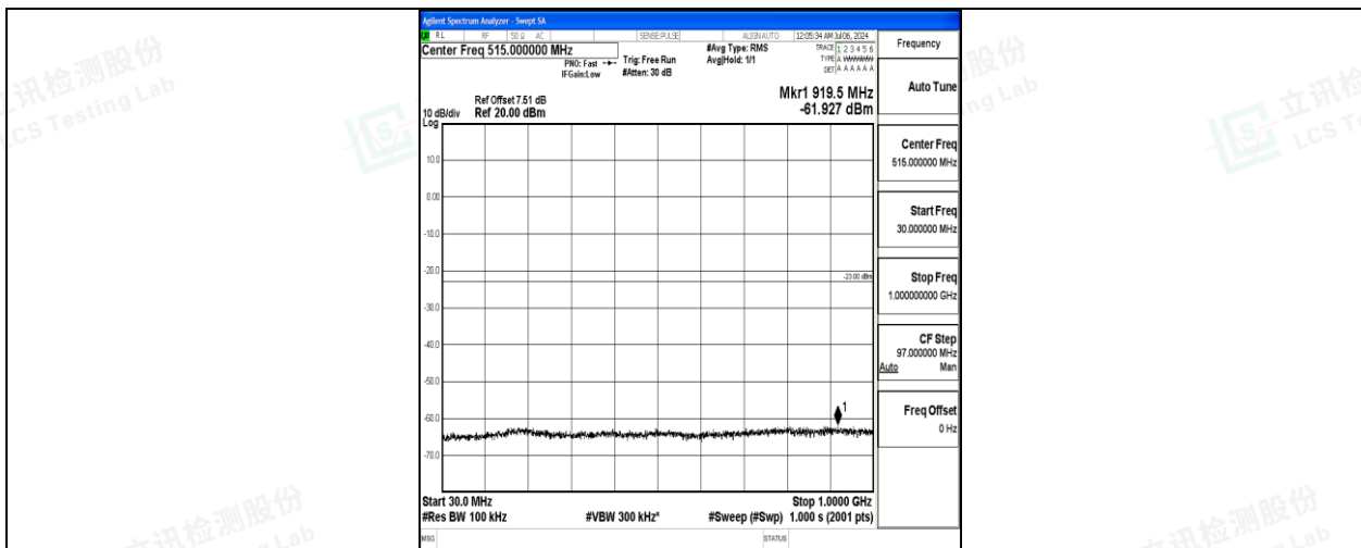
Band4_10MHz_QPSK_20350_1RB#0_30~1000_30~1000
