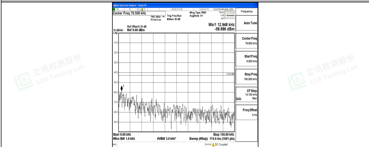
Band4_20MHz_16QAM_20175_1RB#0_0.009~0.15_0.009~0.15
