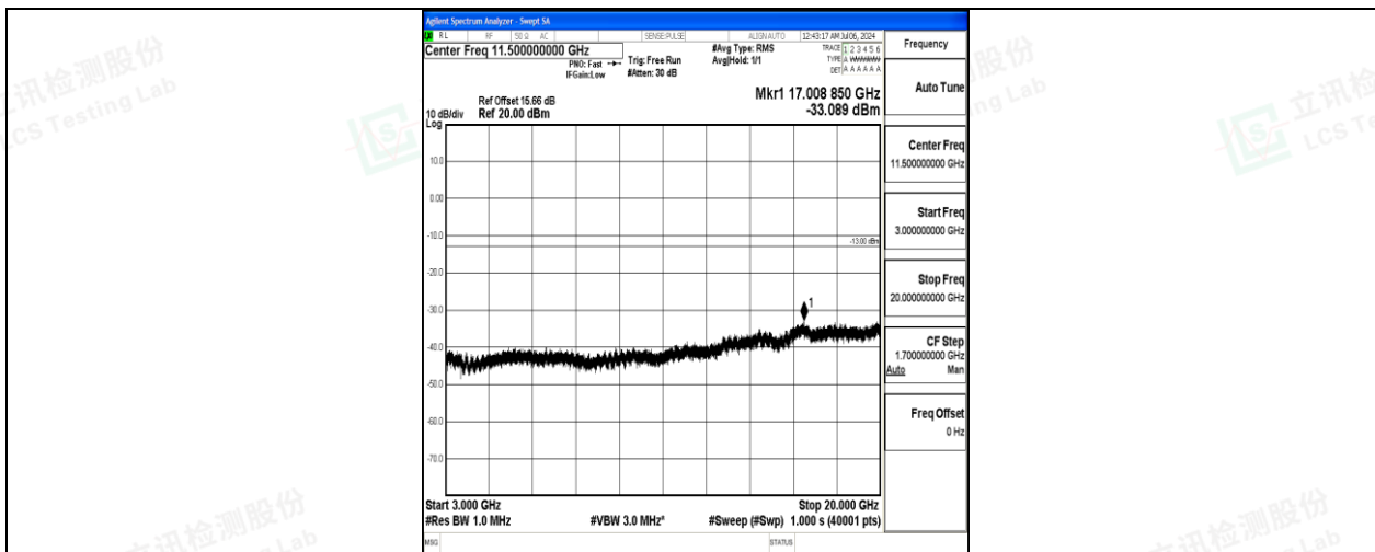
Band4_20MHz_16QAM_20175_1RB#0_3000~20000_3000~20000
