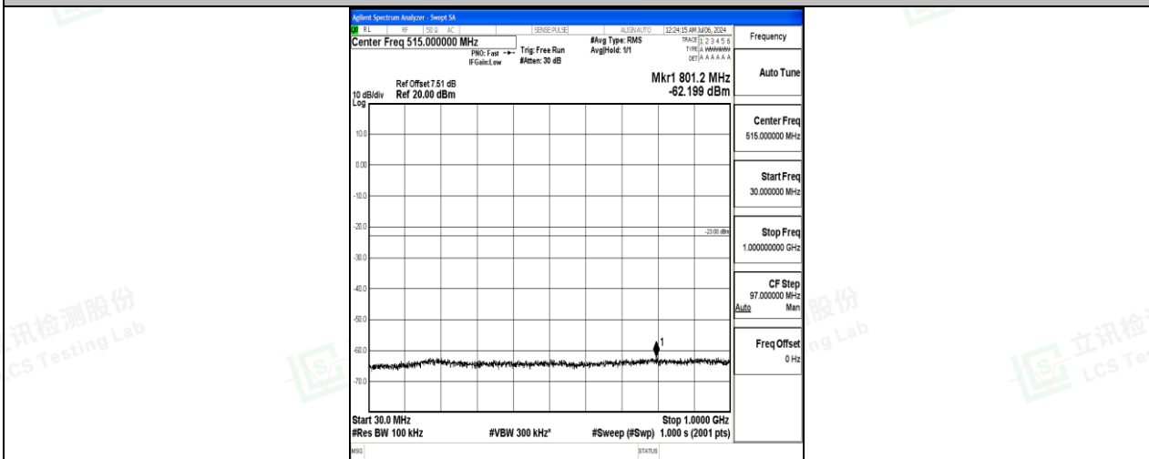
Band4_15MHz_16QAM_20175_1RB#0_30~1000_30~1000
