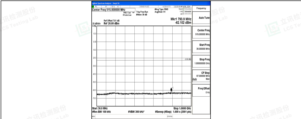
Band4_15MHz_16QAM_20025_1RB#0_30~1000_30~1000
