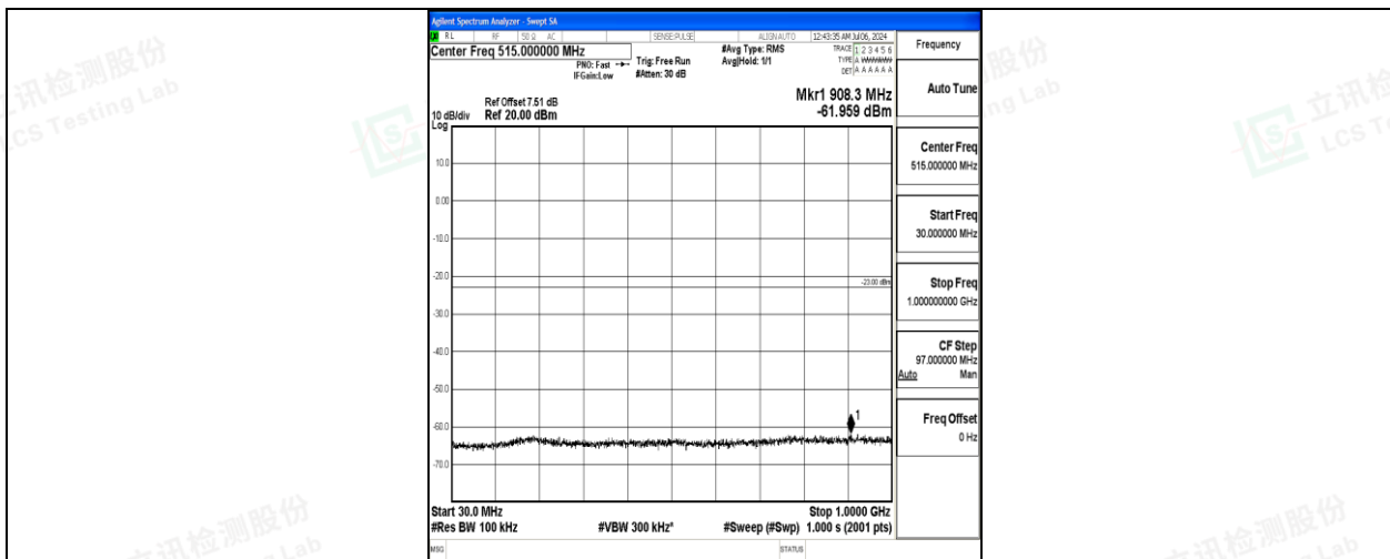
Band4_20MHz_QPSK_20300_1RB#0_30~1000_30~1000
