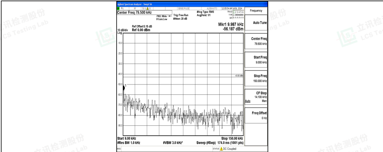
Band4_10MHz_16QAM_20350_1RB#0_0.009~0.15_0.009~0.15
