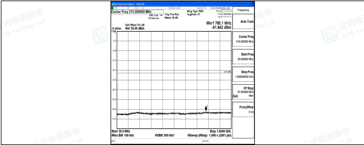
Band4_20MHz_16QAM_20050_1RB#0_30~1000_30~1000
