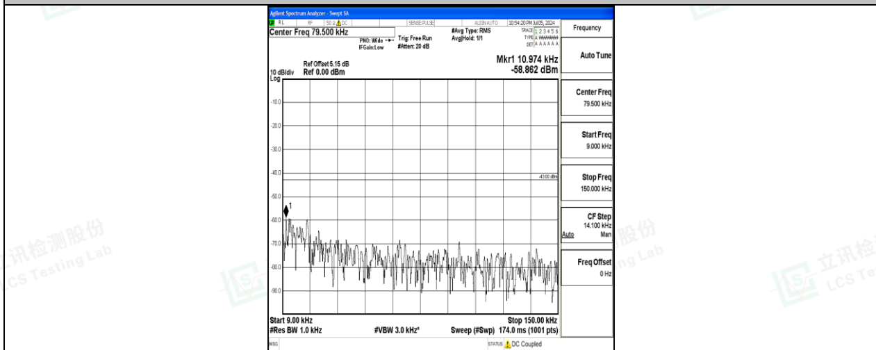
Band4_1.4MHz_QPSK_20393_1RB#0_0.009~0.15_0.009~0.15
