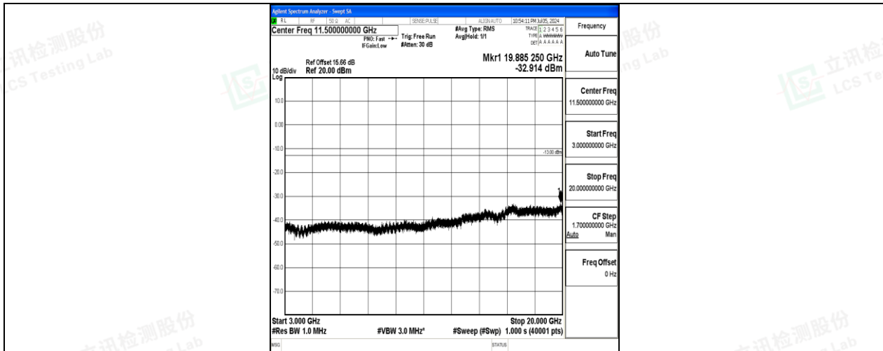
Band4_1.4MHz_16QAM_20175_1RB#0_3000~20000_3000~20000
