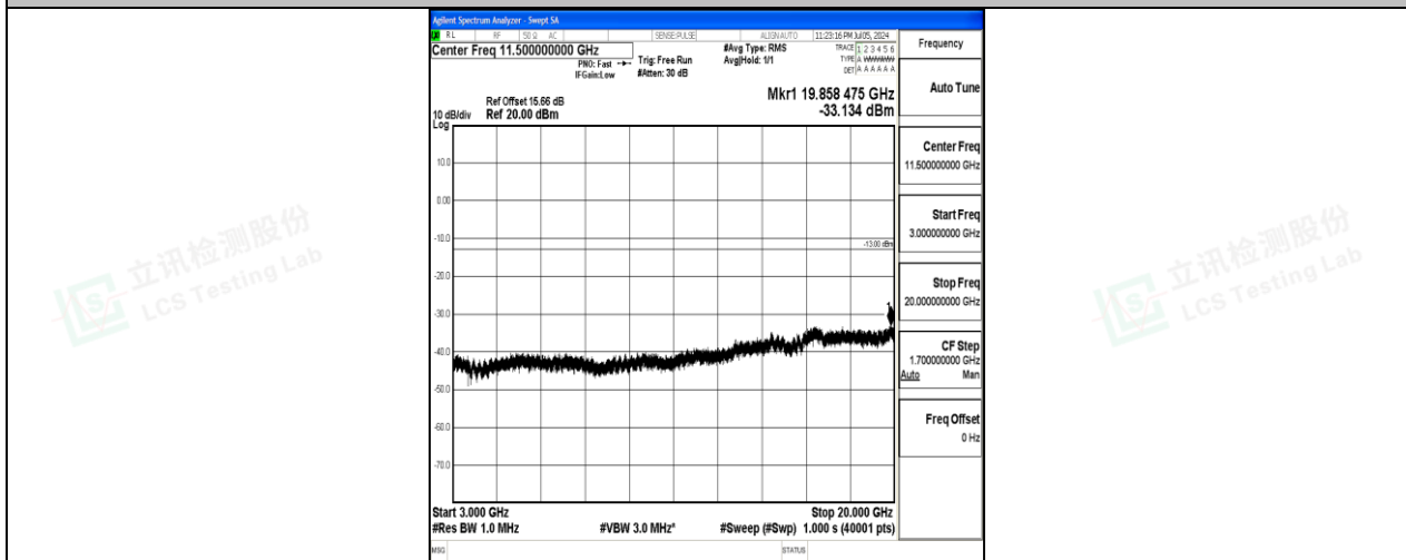
Band4_3MHz_QPSK_20385_1RB#0_3000~20000_3000~20000
