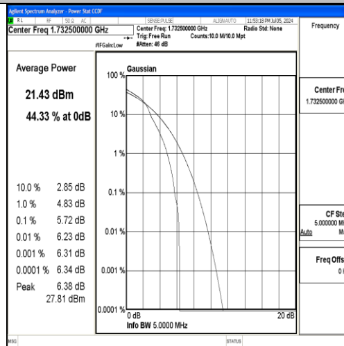
Band4-5MHz-16QAM-20175-1RB#0-PASS
