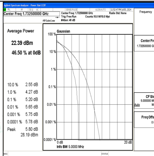
Band4-5MHz-QPSK-20175-1RB#0-PASS
