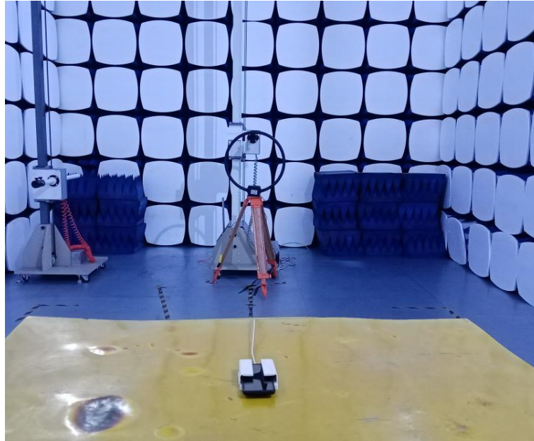
Radiated emission 9KHz~30MHz
