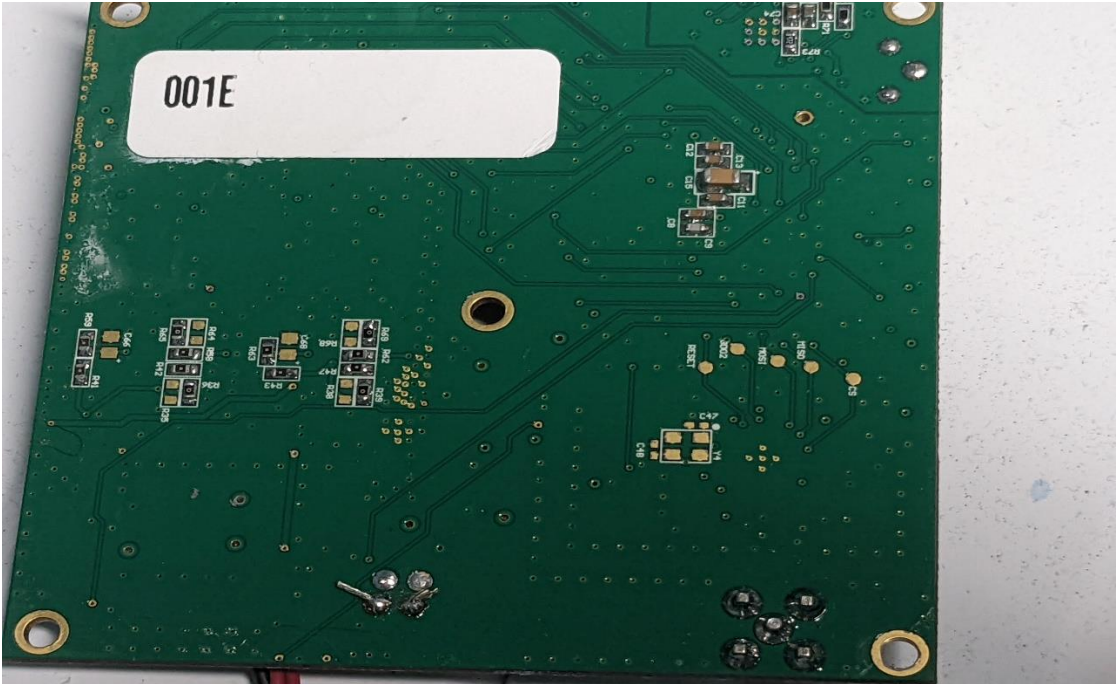
Internal Photos – Transmitter PCB Bottom
