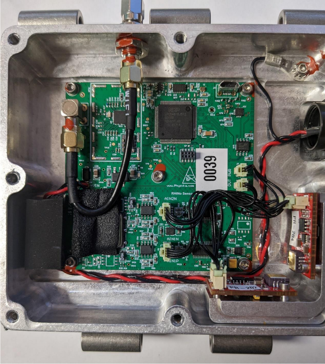
Internal Photos – Transmitter – PHYZ-0001
