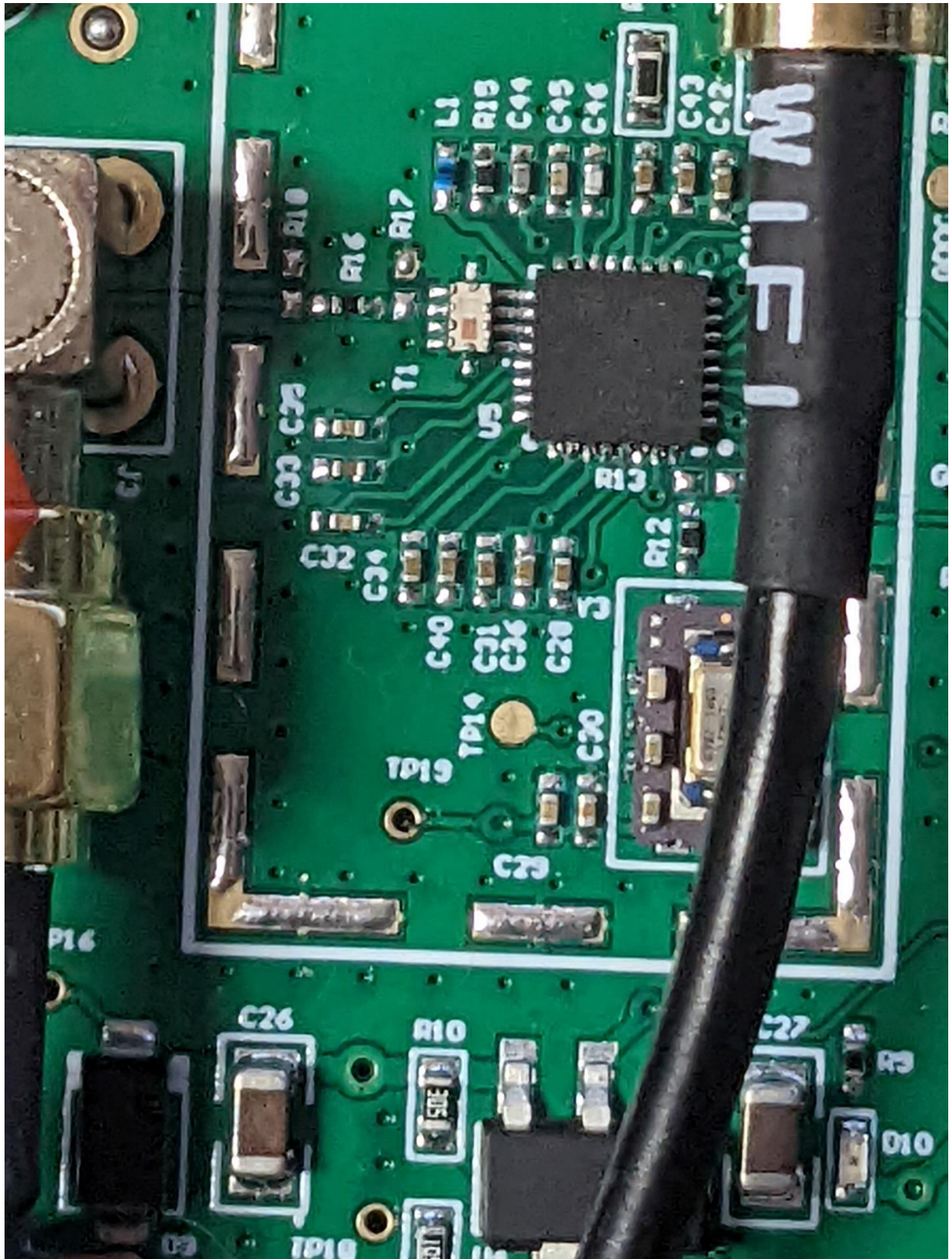
Internal Photos Transmitter – Radio
