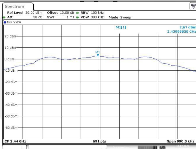
BLE_1M_Ant1_2440
