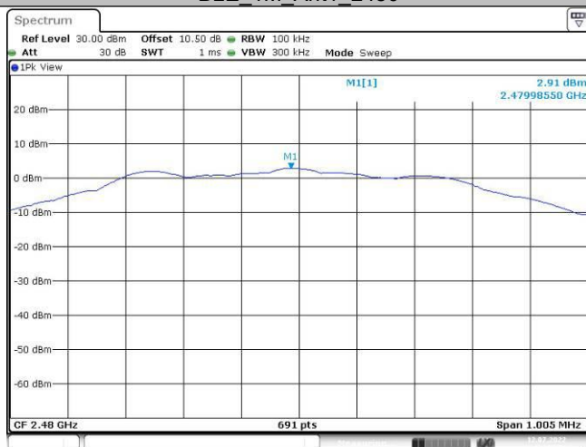
BLE_1M_Ant1_2480
