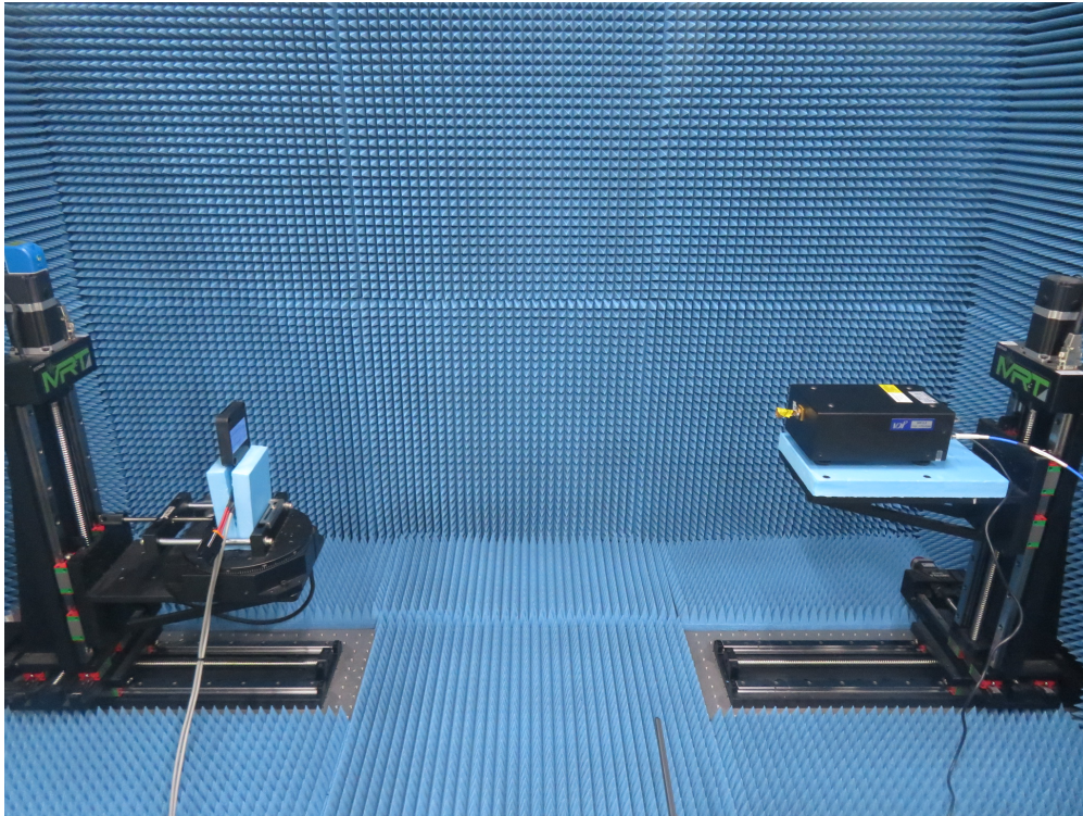
Description: Radiated Emission Test Setup for Above 220GHz
