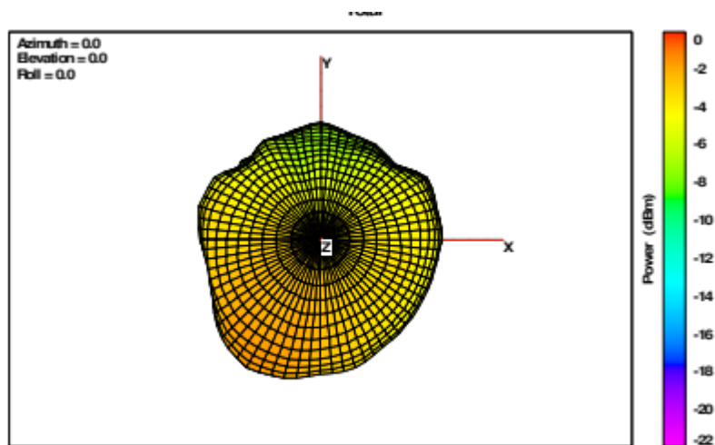
Robot Antenna Front View
