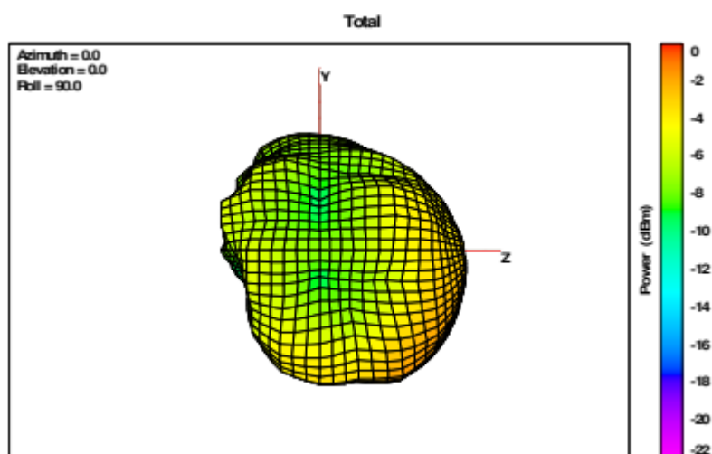
Robot Antenna Front View
