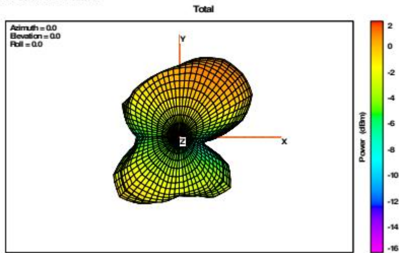
Controller Antenna Front View
