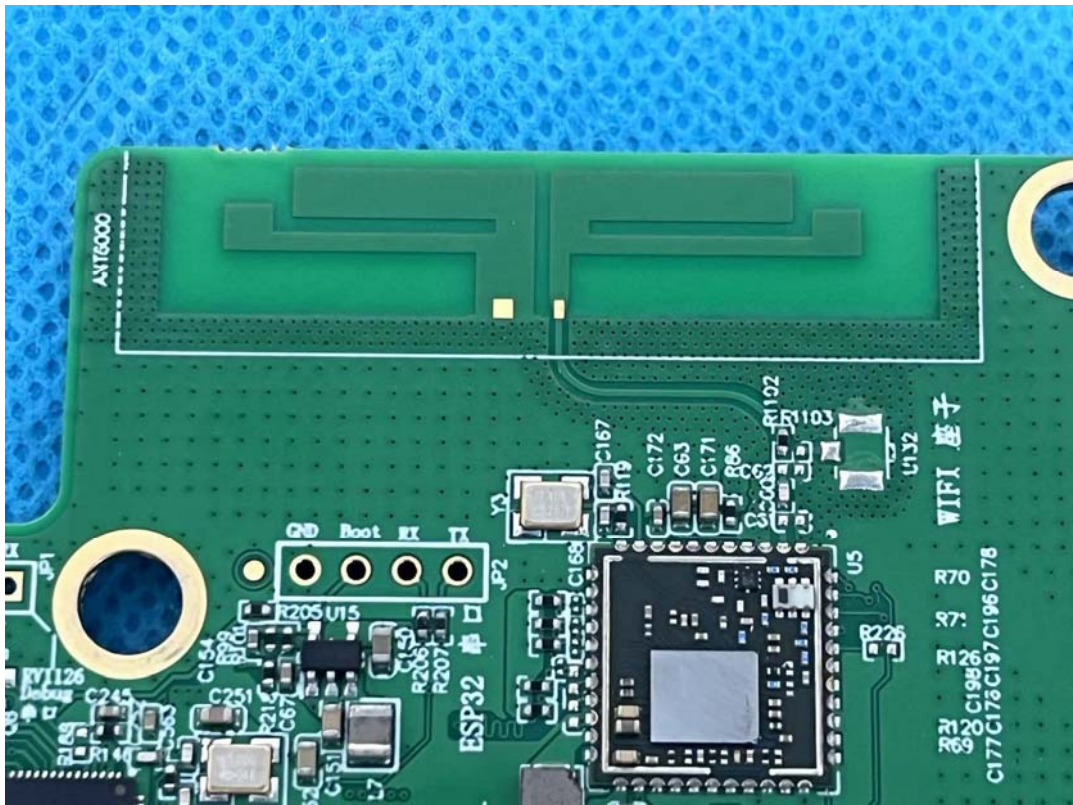
WLAN&Bluetooth Antenna
