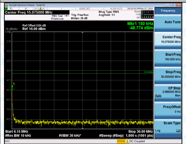
Band4_3MHz_QPSK_20175_1RB#14_1000-3000_1000-3000
