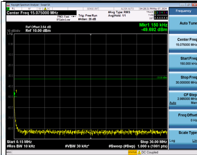
Band4_1.4MHz_QPSK_20393_1RB#5_1000-3000_1000-3000
