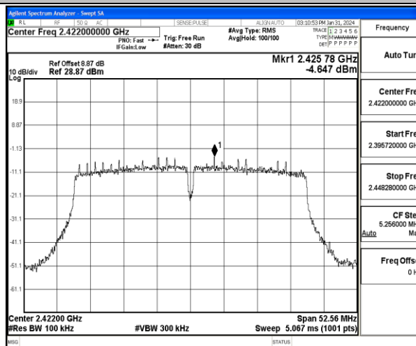
11N40MIMO-Ant2-2422-PASS
