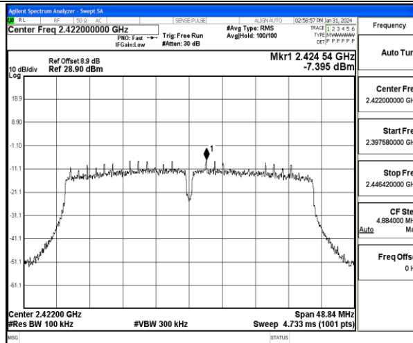
11N40MIMO-Ant1-2422-PASS
