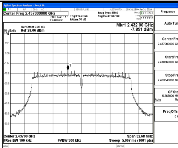
11N40MIMO-Ant1-2437-PASS
