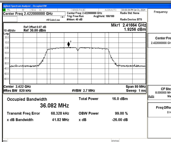
11N40MIMO-Ant2-2422
