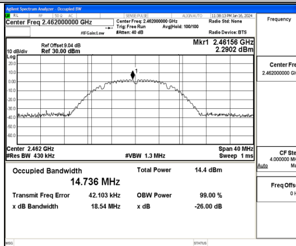
11B-Ant2-2462
