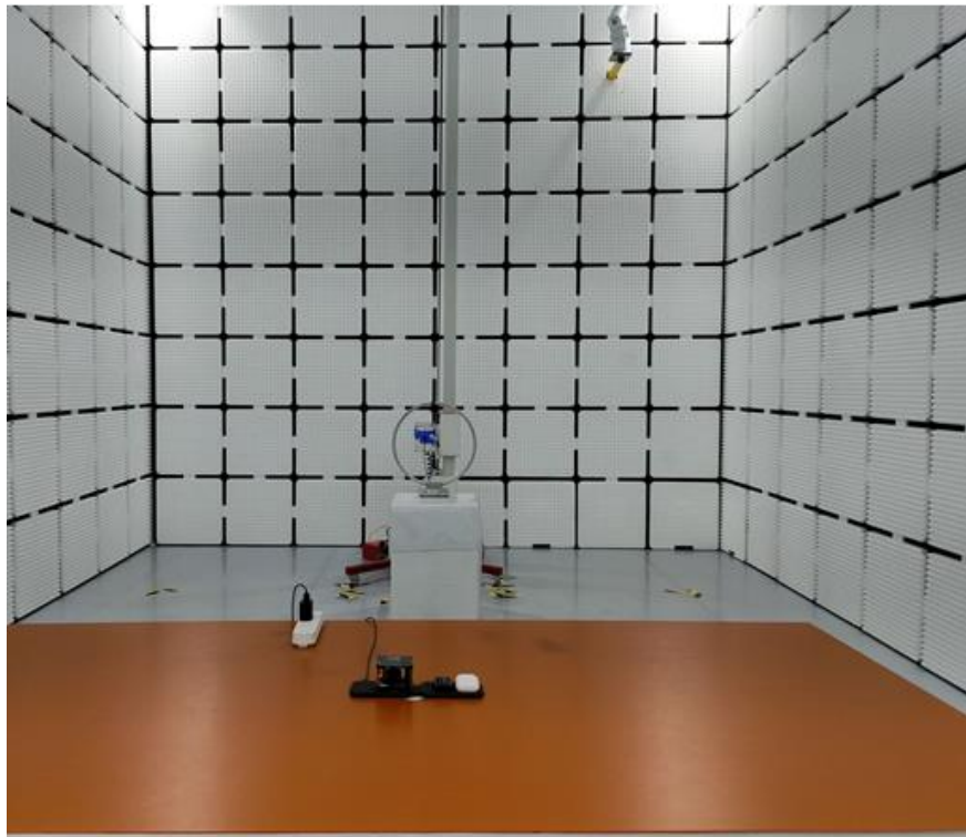
Radiated emissions- Below 30MHz
