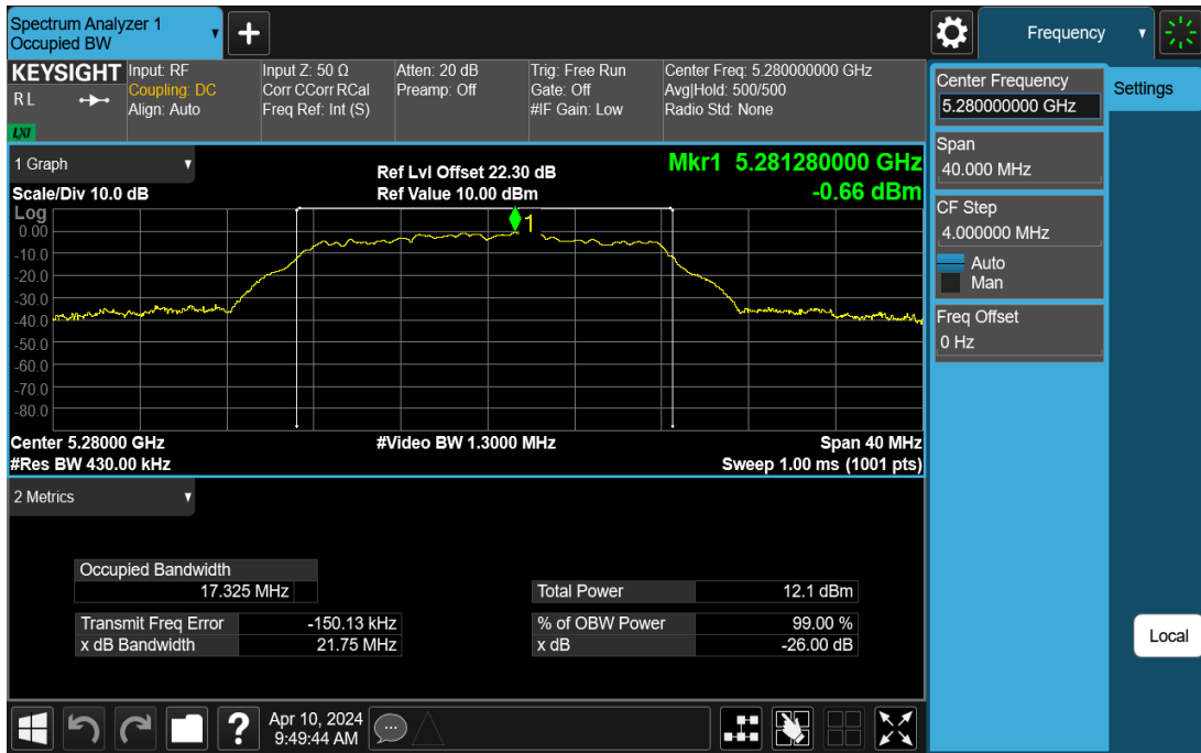
11AC20SISO-Ant1-5280
