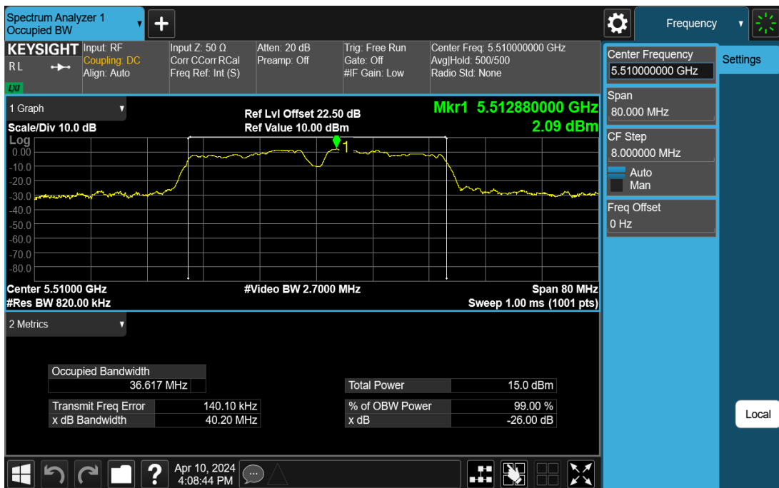
11AC40SISO-Ant1-5510
