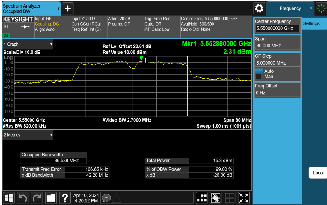
11AC40SISO-Ant1-5550
