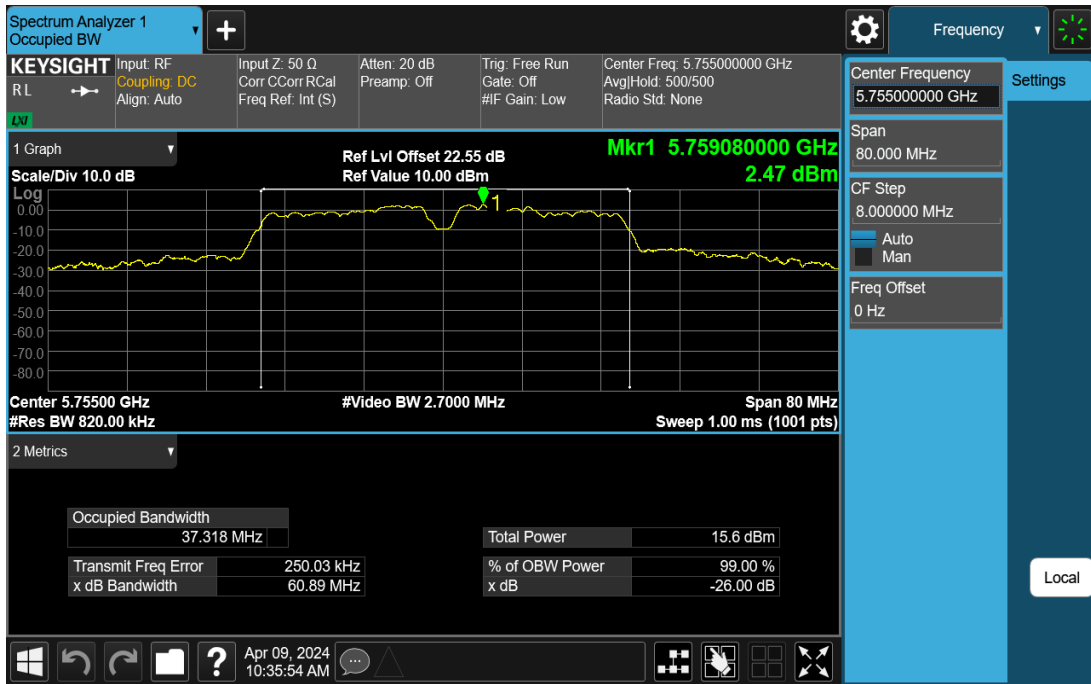
11N40SISO-Ant1-5755
