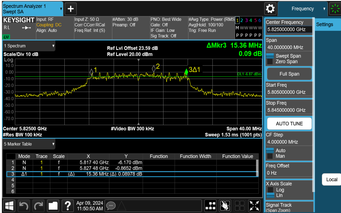
11AC20SISO-Ant1-5825-PASS
