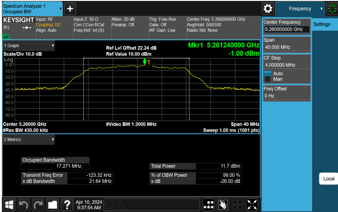
11AC20SISO-Ant1-5260
