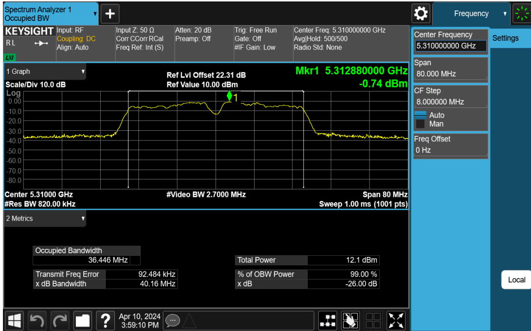
11AC40SISO-Ant1-5310
