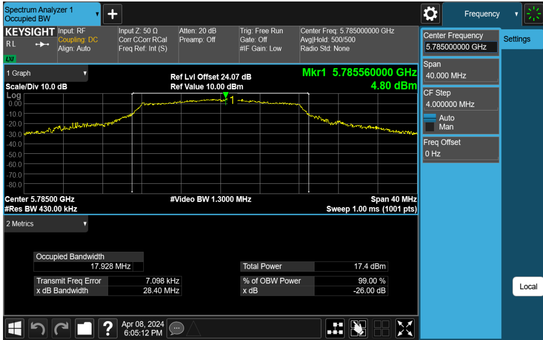
11A-Ant1-5785
