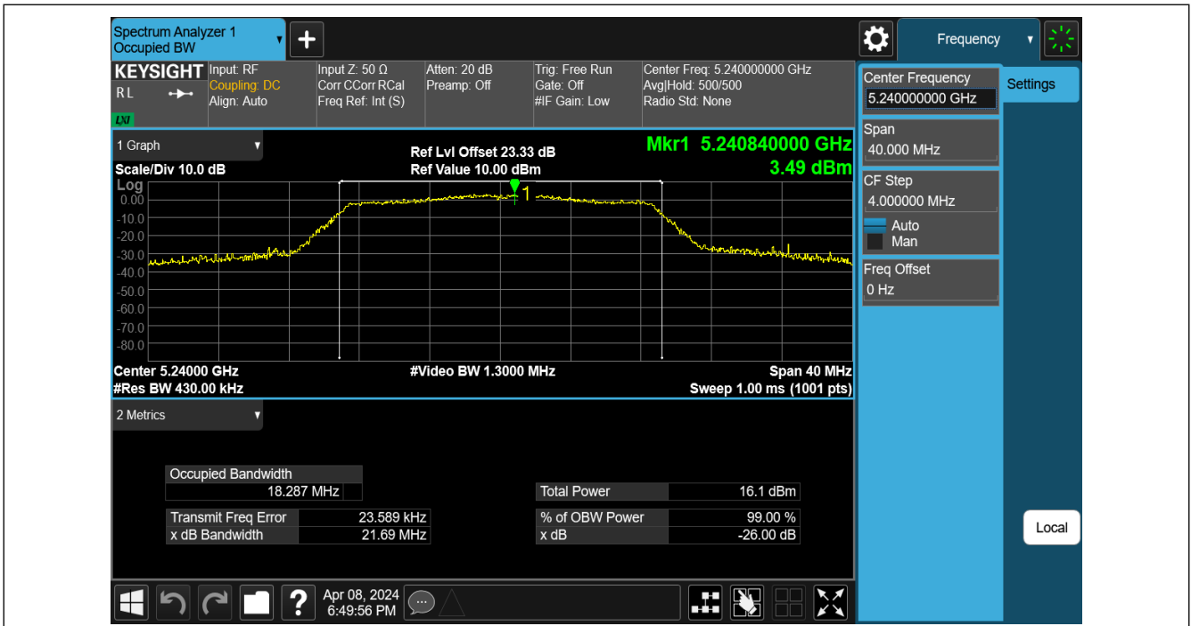
11N20SISO-Ant1-5240
