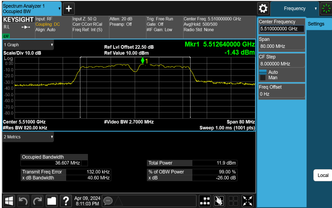
11N40SISO-Ant1-5510
