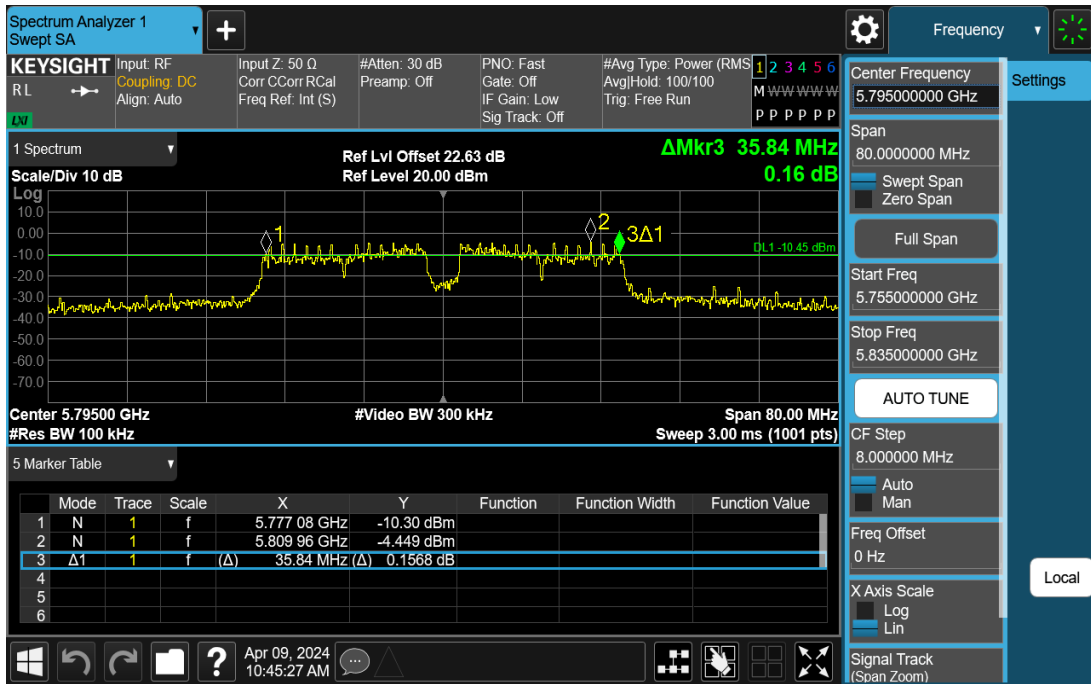
11N40SISO-Ant1-5795-PASS
