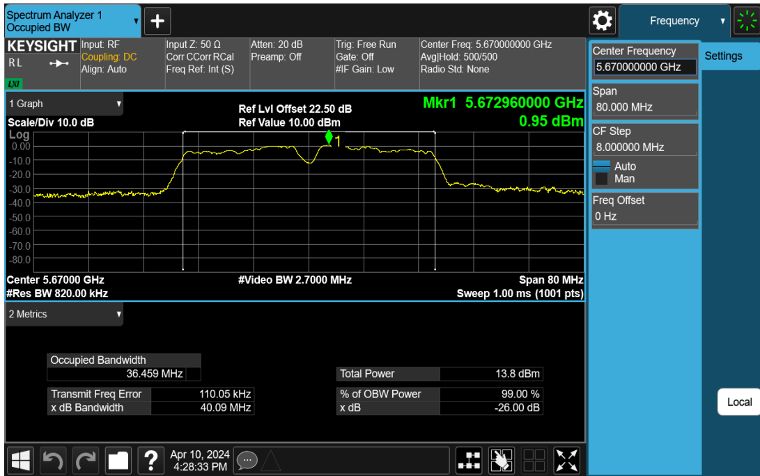
11AC40SISO-Ant1-5670
