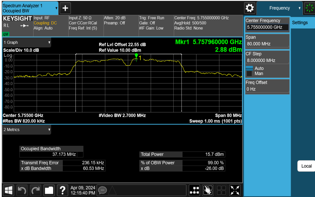
11AC40SISO-Ant1-5755
