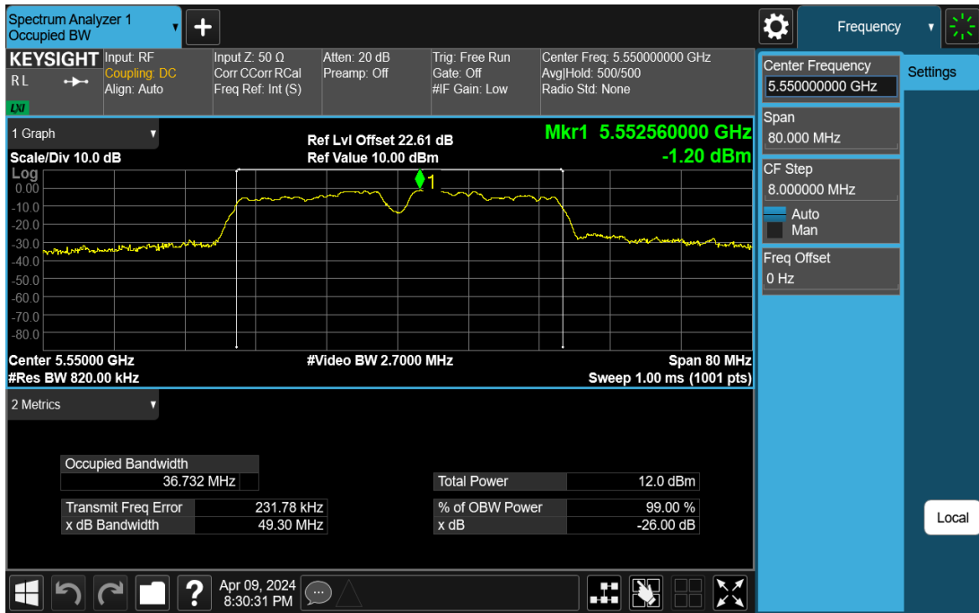
11N40SISO-Ant1-5550
