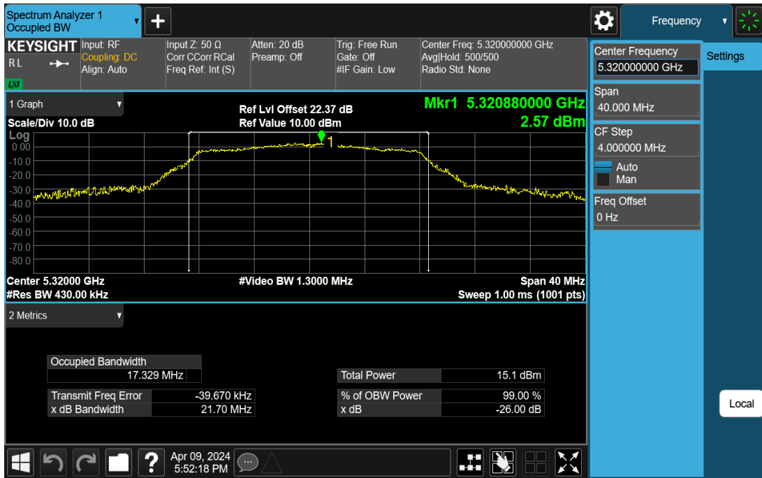
11A-Ant1-5320
