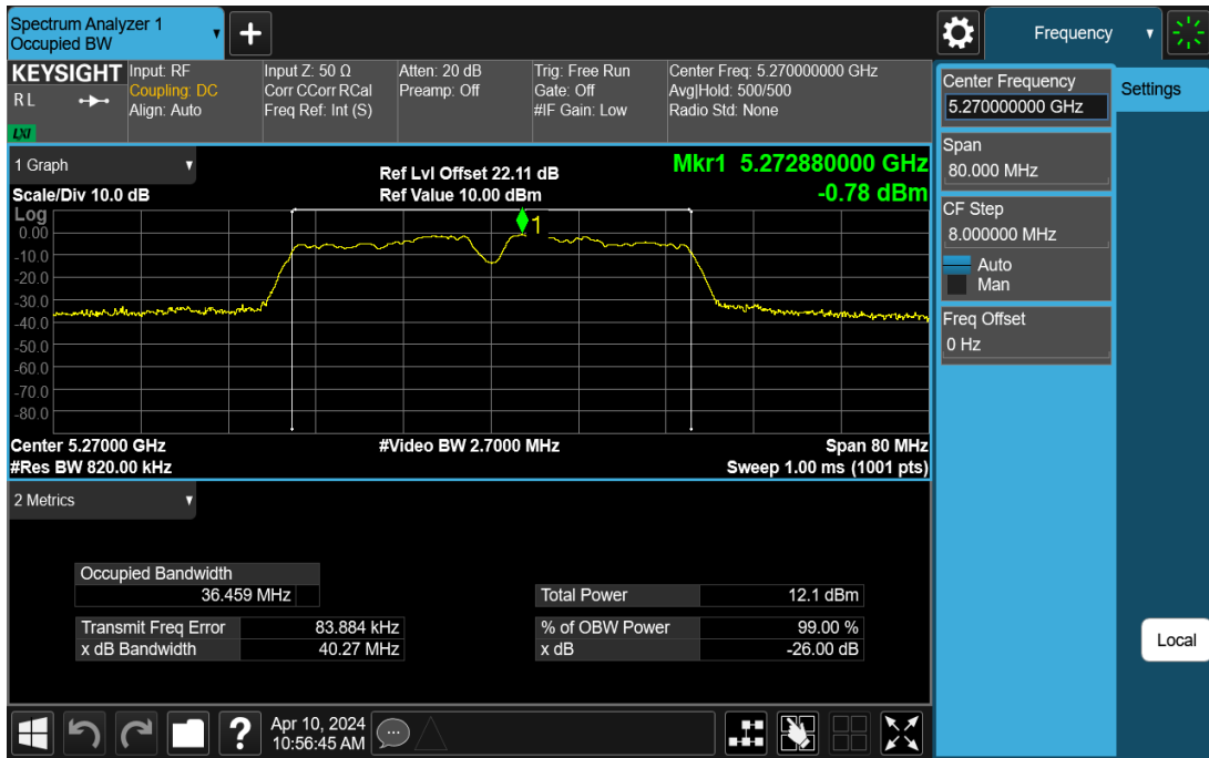
11AC40SISO-Ant1-5270
