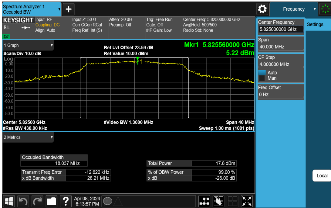
11A-Ant1-5825
