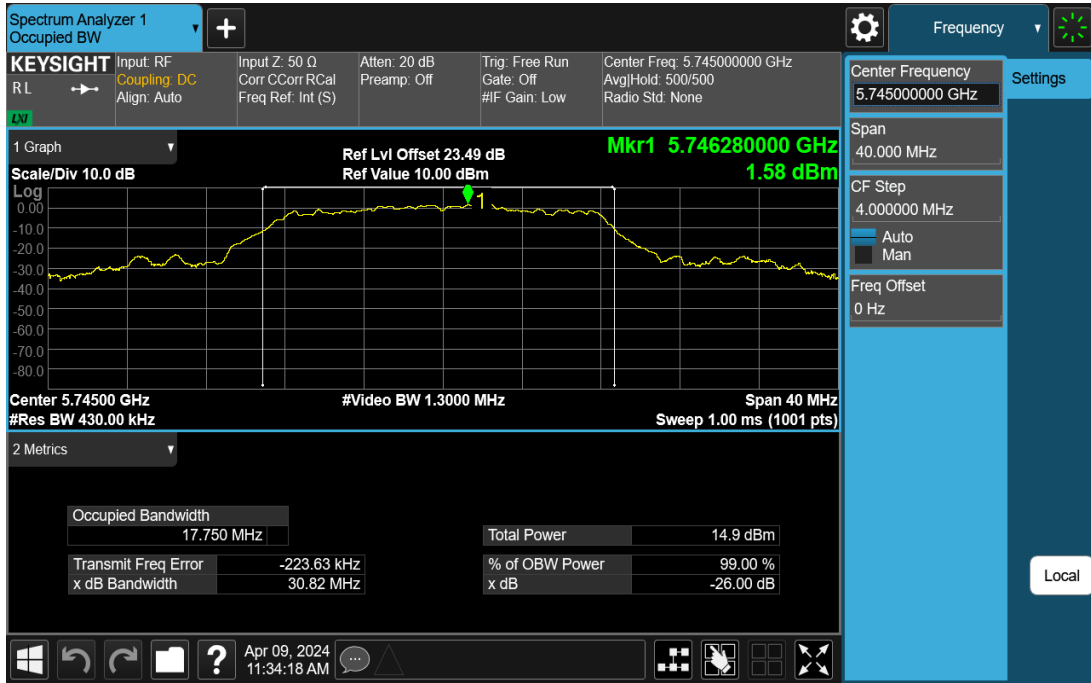
11AC20SISO-Ant1-5745
