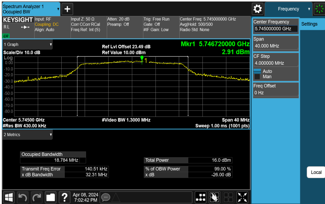
11N20SISO-Ant1-5745
