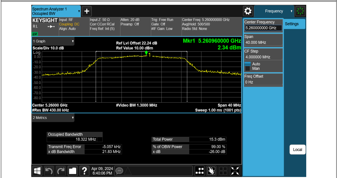
11N20SISO-Ant1-5260
