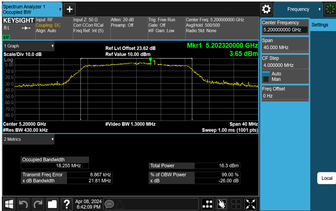
11N20SISO-Ant1-5200
