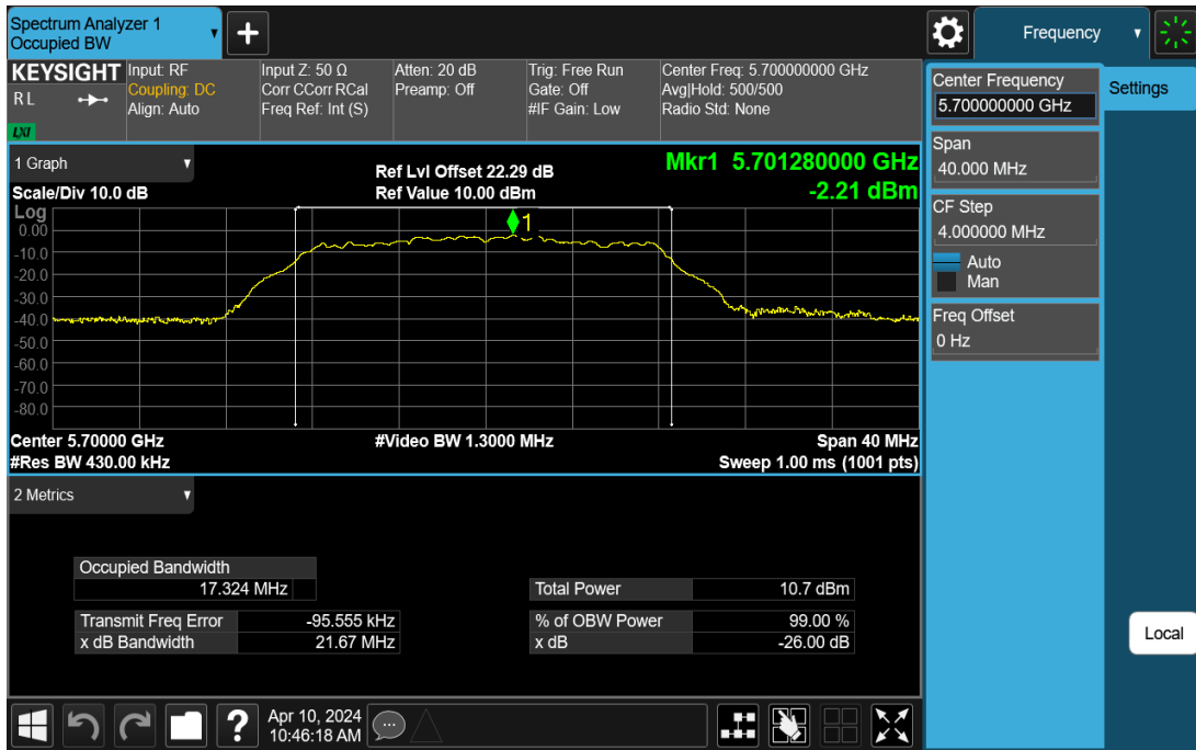
11AC20SISO-Ant1-5700
