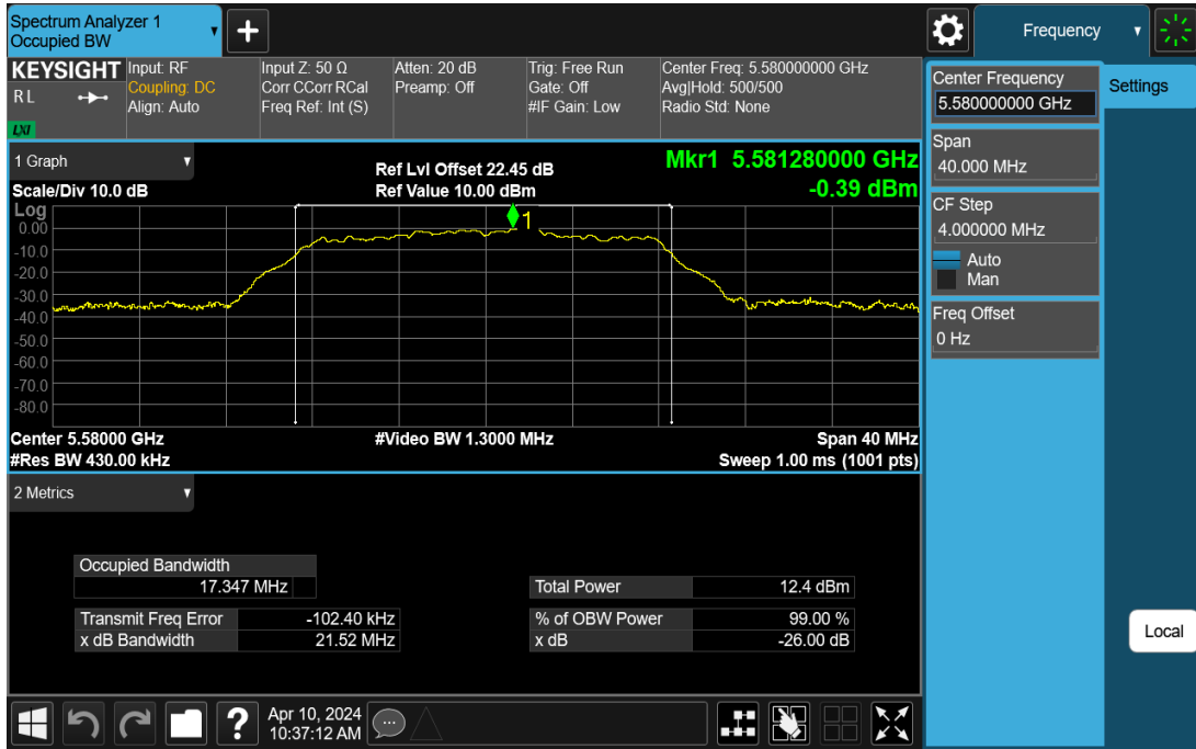
11AC20SISO-Ant1-5580
