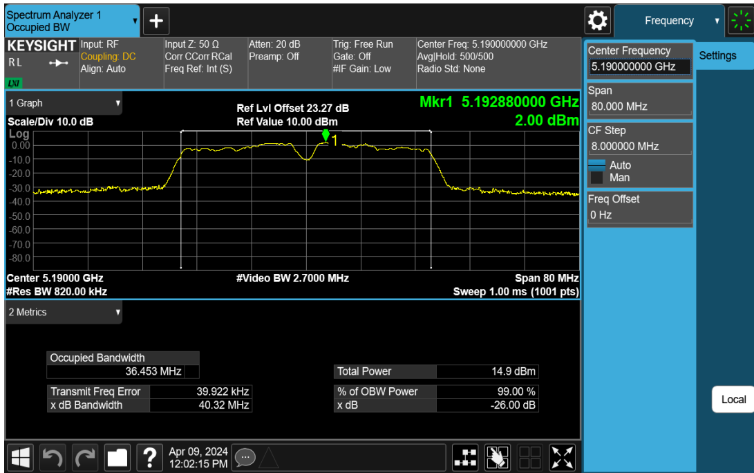
11AC40SISO-Ant1-5190
