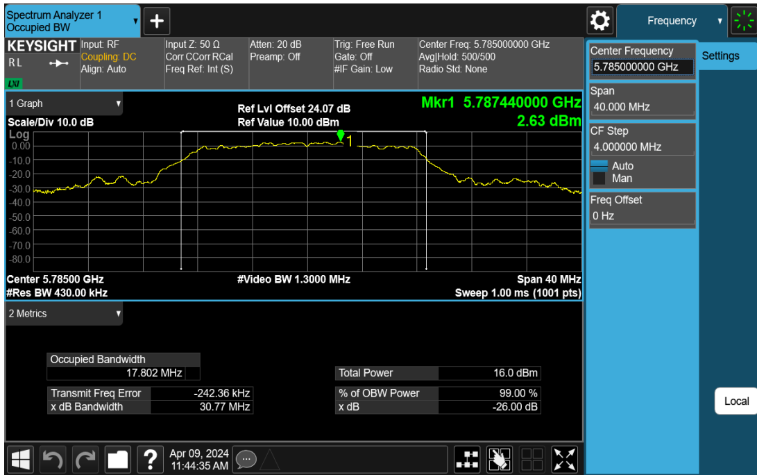
11AC20SISO-Ant1-5785
