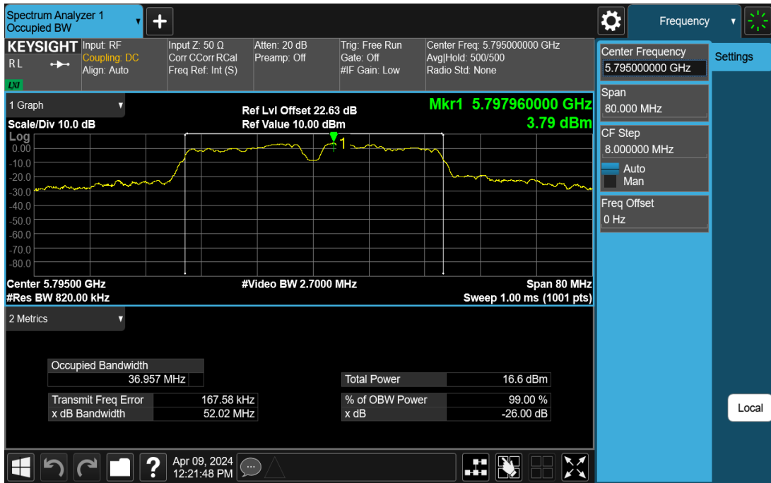
11AC40SISO-Ant1-5795
