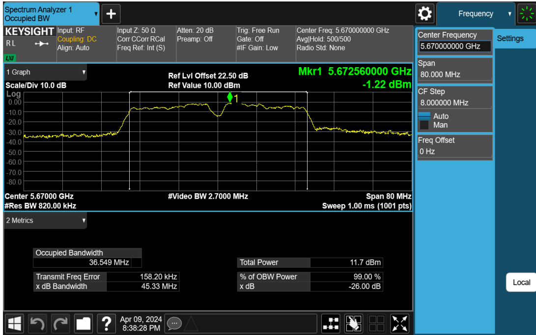
11N40SISO-Ant1-5670
