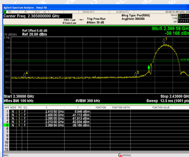
802.11b_Low Channel
