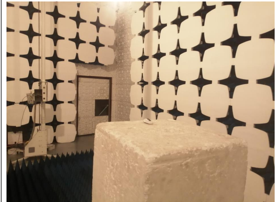
Above 1GHz
