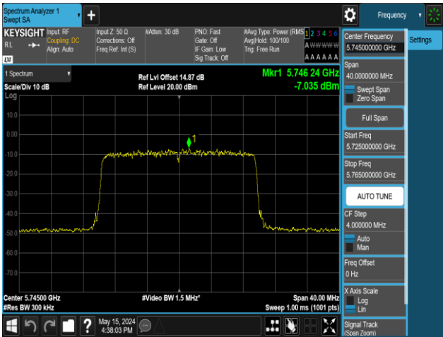
11AX20MIMO-Ant1-5745-106Tone-RU54-PASS
