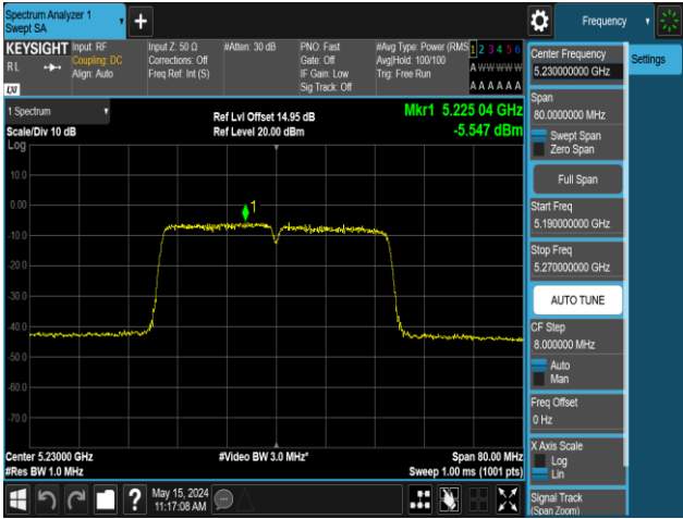
11AC40MIMO-Ant2-5230-PASS
