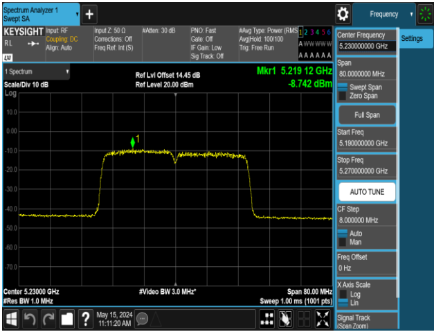
11AC40MIMO-Ant1-5230-PASS
