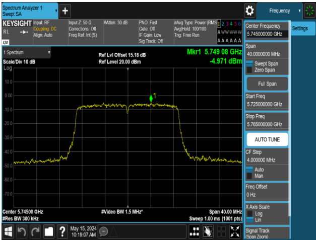
11AC20MIMO-Ant2-5745-PASS
