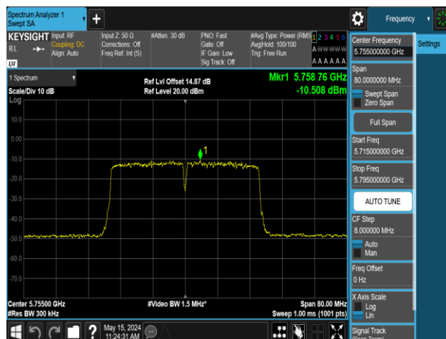
11AC40MIMO-Ant1-5755-PASS
