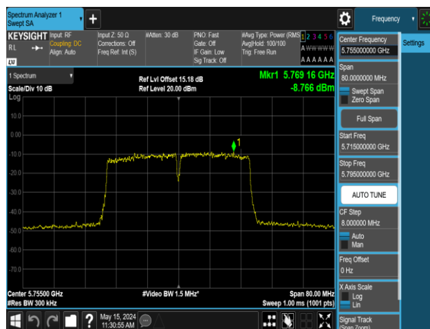
11AC40MIMO-Ant2-5755-PASS
