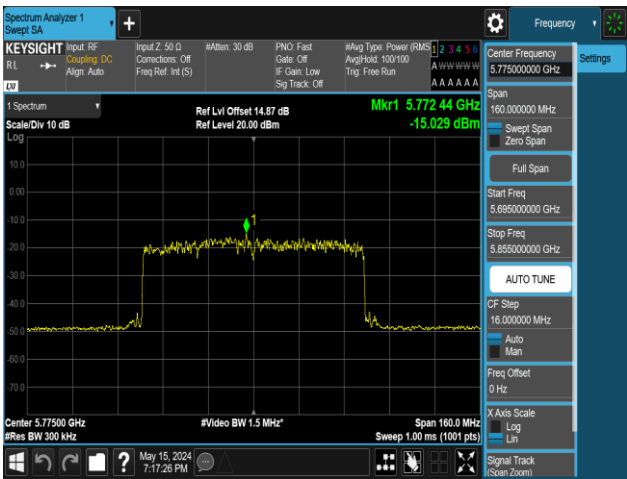
11AX80MIMO-Ant1-5775-484Tone-RU66-PASS
