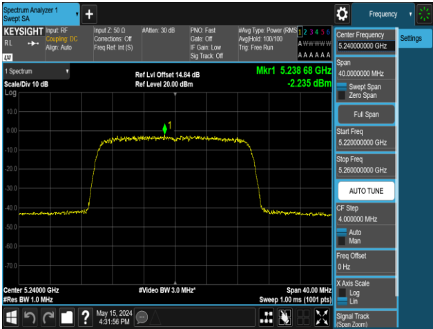
11AX20MIMO-Ant2-5240-106Tone-RU54-PASS
