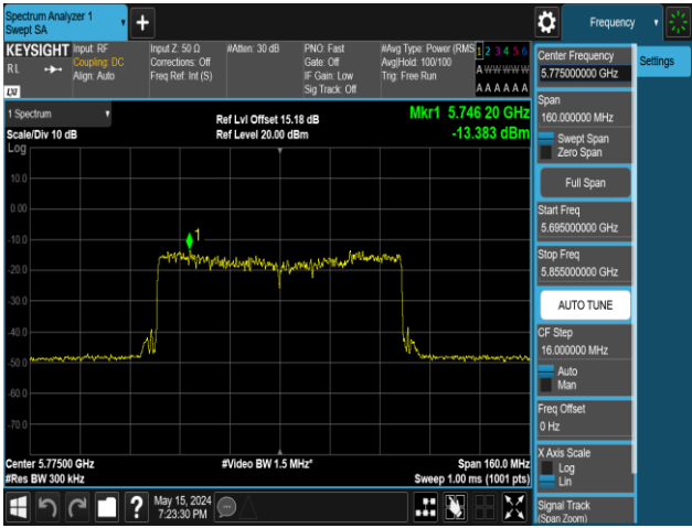
11AX80MIMO-Ant2-5775-484Tone-RU66-PASS
