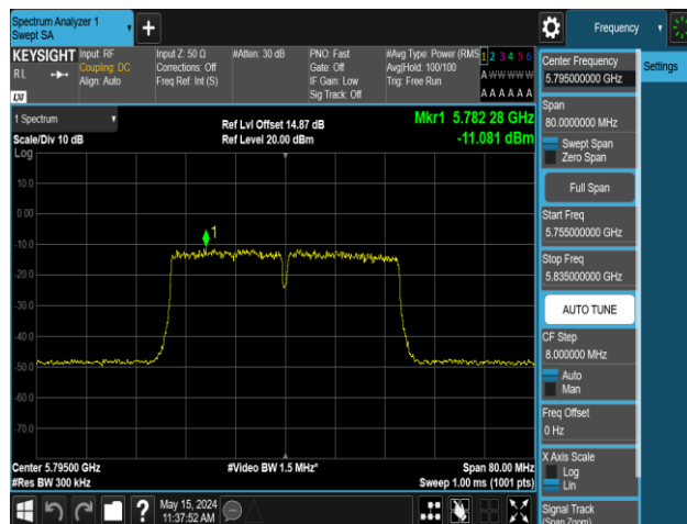
11AC40MIMO-Ant1-5795-PASS
