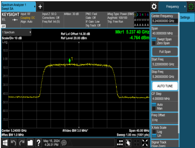
11AX20MIMO-Ant1-5240-106Tone-RU54-PASS
