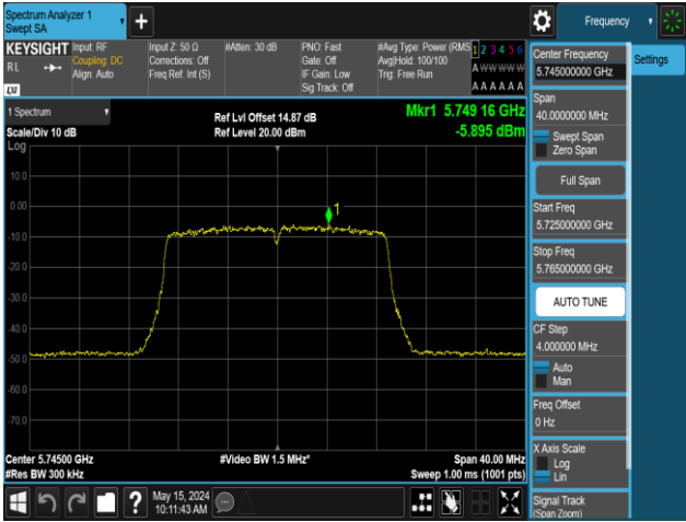
11AC20MIMO-Ant1-5745-PASS
