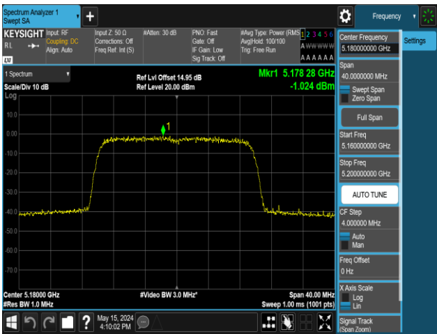
11AX20MIMO-Ant2-5180-106Tone-RU54-PASS
