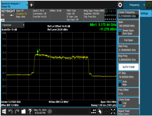
11AX80MIMO-Ant1-5210-484Tone-RU66-PASS
