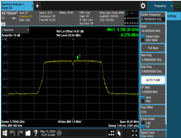
11AC20MIMO-Ant1-5785-PASS
