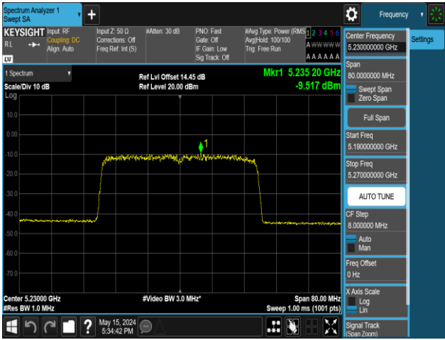
11AX40MIMO-Ant1-5230-242Tone-RU62-PASS
