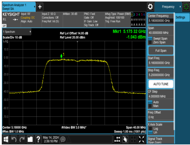
11N20MIMO-Ant2-5180-PASS
