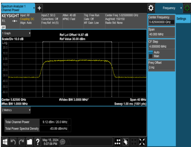
11AX20MIMO-Ant1-5825-106Tone-RU54-PASS
