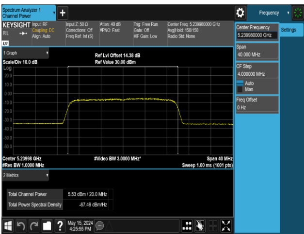
11AX20MIMO-Ant1-5240-106Tone-RU54-PASS
