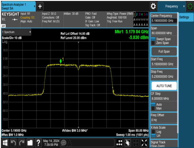
11N40MIMO-Ant2-5190-PASS
