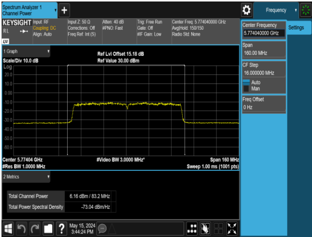
11AC80MIMO-Ant2-5775-PASS
