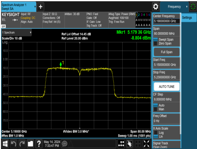
11N40MIMO-Ant1-5190-PASS
