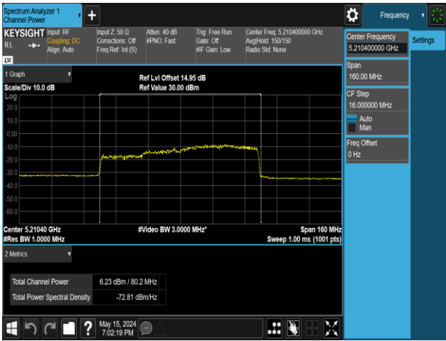
11AX80MIMO-Ant2-5210-484Tone-RU66-PASS
