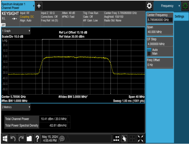
11AX20MIMO-Ant2-5785-106Tone-RU54-PASS
