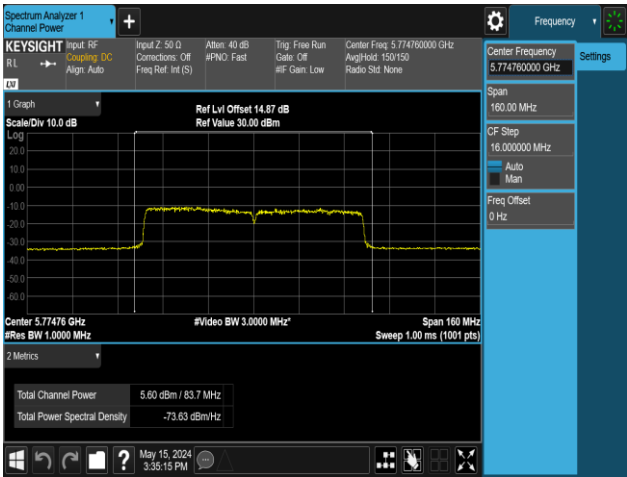
11AC80MIMO-Ant1-5775-PASS
