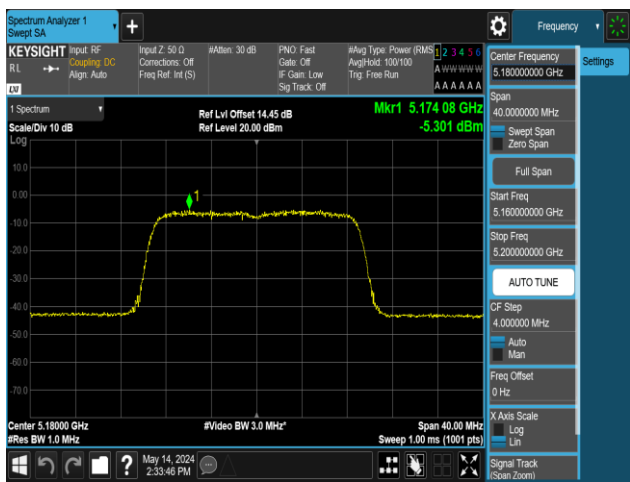
11N20MIMO-Ant1-5180-PASS
