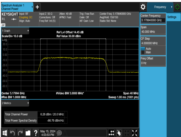
11AX20MIMO-Ant1-5180-106Tone-RU54-PASS
