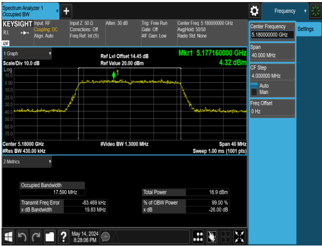
11AC20MIMO-Ant1-5180
