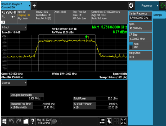
11AX20MIMO-Ant1-5745-106Tone-RU54
