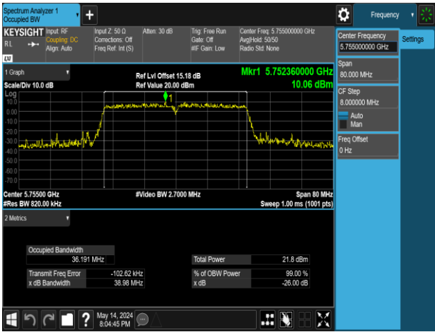
11N40MIMO-Ant2-5755
