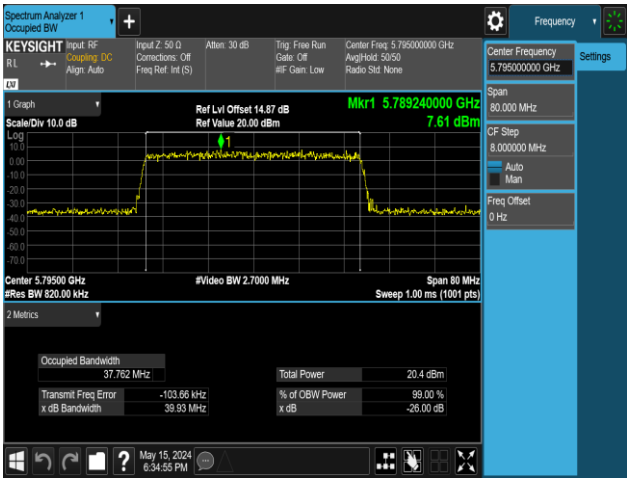
11AX40MIMO-Ant1-5795-242Tone-RU62
