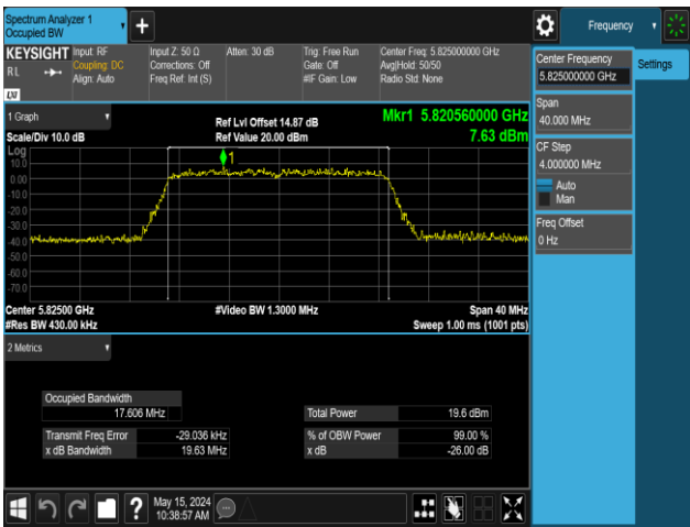
11AC20MIMO-Ant1-5825
