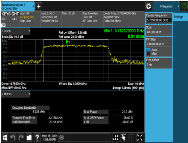
11AX20MIMO-Ant2-5785-106Tone-RU54
