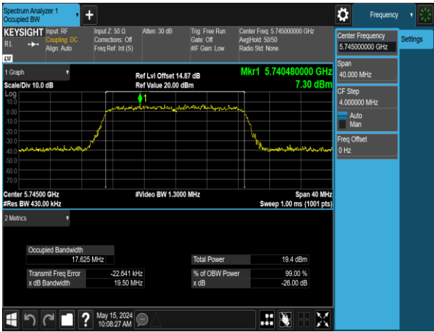
11AC20MIMO-Ant1-5745
