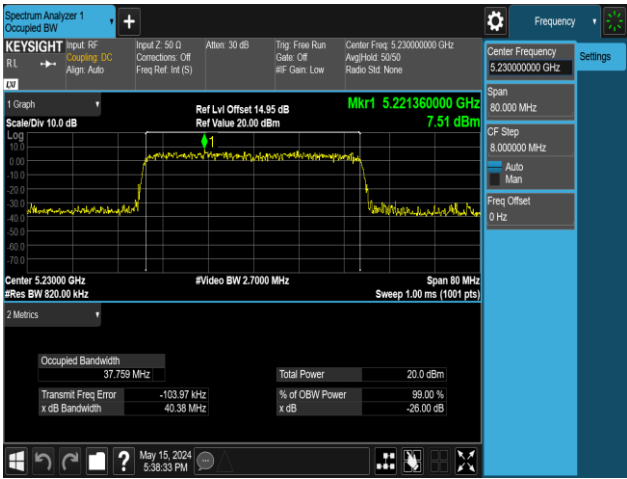
11AX40MIMO-Ant2-5230-242Tone-RU62
