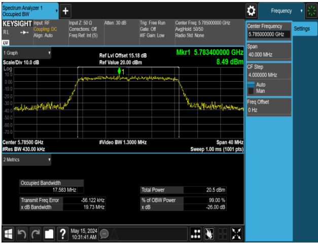
11AC20MIMO-Ant2-5785
