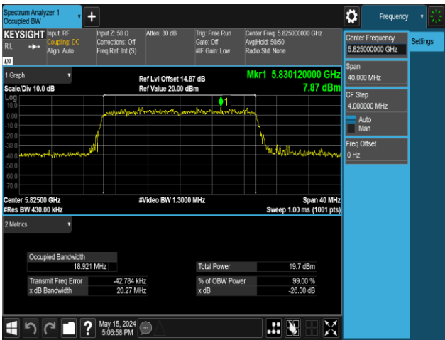
11AX20MIMO-Ant1-5825-106Tone-RU54
