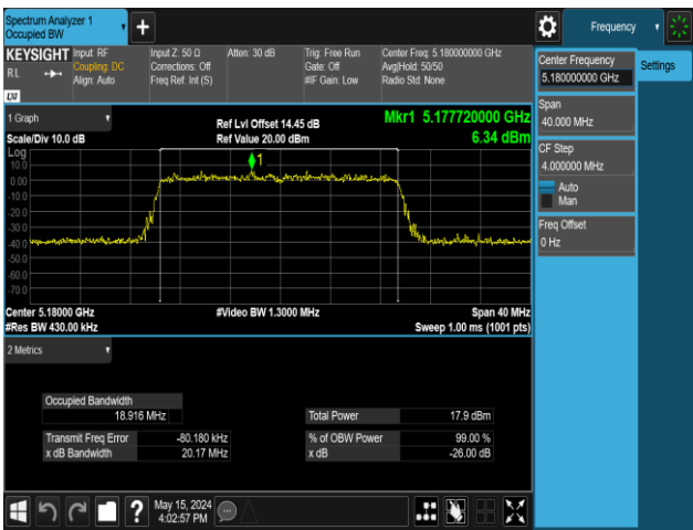
11AX20MIMO-Ant1-5180-106Tone-RU54
