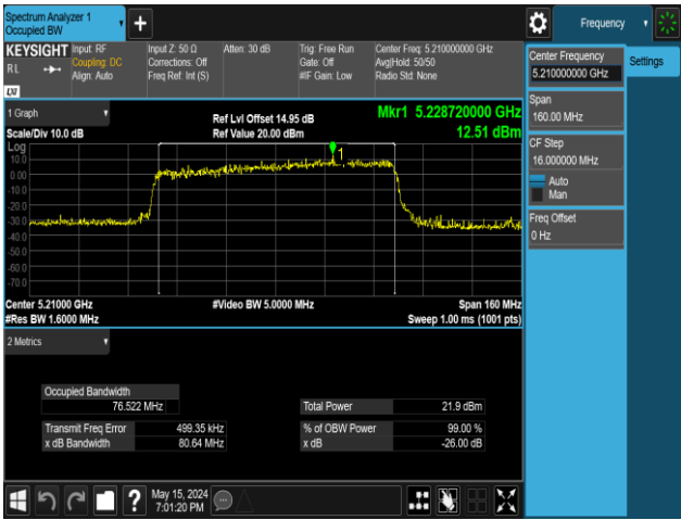
11AX80MIMO-Ant2-5210-484Tone-RU66
