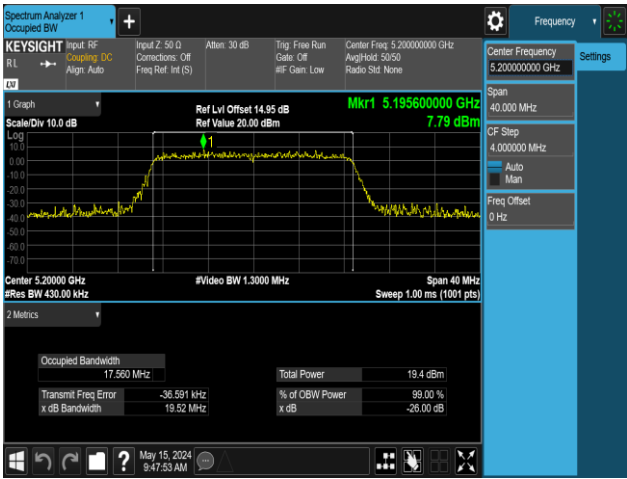
11AC20MIMO-Ant2-5200
