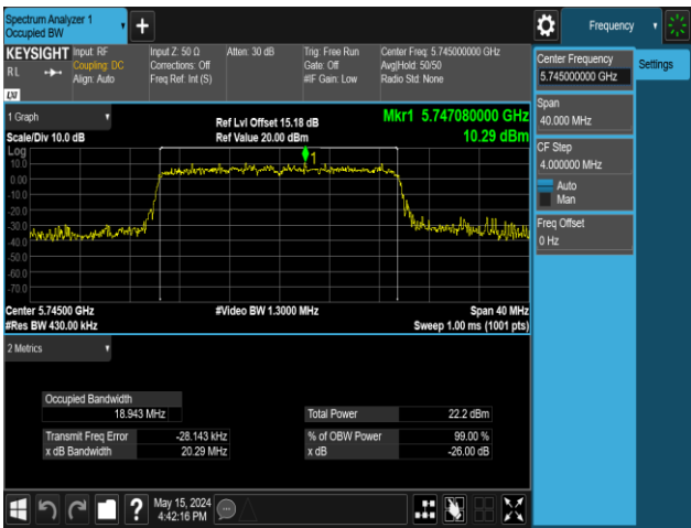
11AX20MIMO-Ant2-5745-106Tone-RU54
