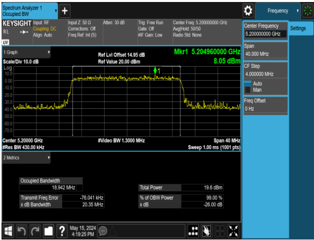
11AX20MIMO-Ant2-5200-106Tone-RU54
