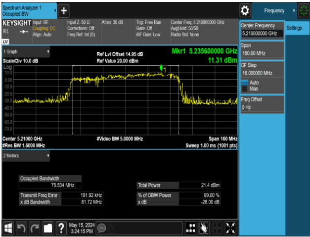
11AC80MIMO-Ant2-5210
