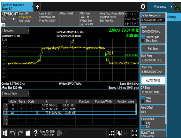
11AX80MIMO-Ant1-5775-484Tone-RU66
