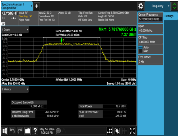
11N20MIMO-Ant1-5785
