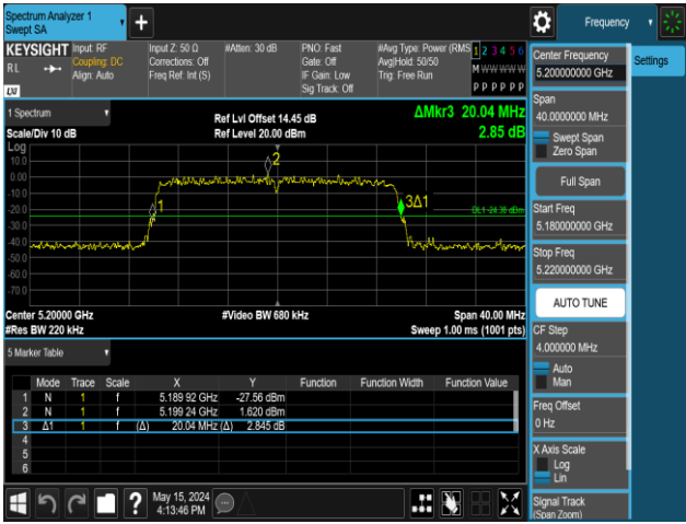
11AX20MIMO-Ant1-5200-106Tone-RU54
