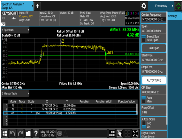
11AX40MIMO-Ant2-5755-242Tone-RU62
