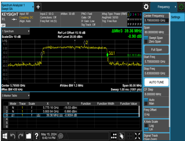
11AX40MIMO-Ant2-5795-242Tone-RU62
