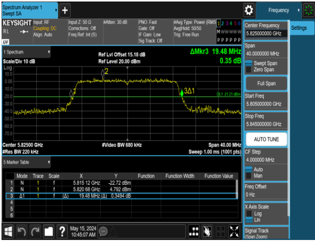
11AC20MIMO-Ant2-5825
