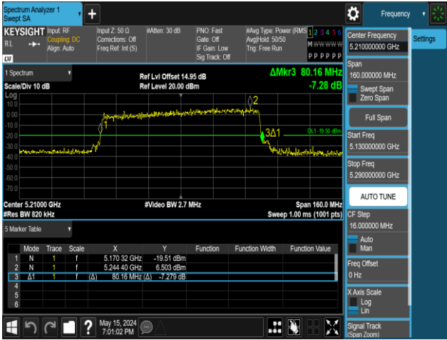
11AX80MIMO-Ant2-5210-484Tone-RU66
