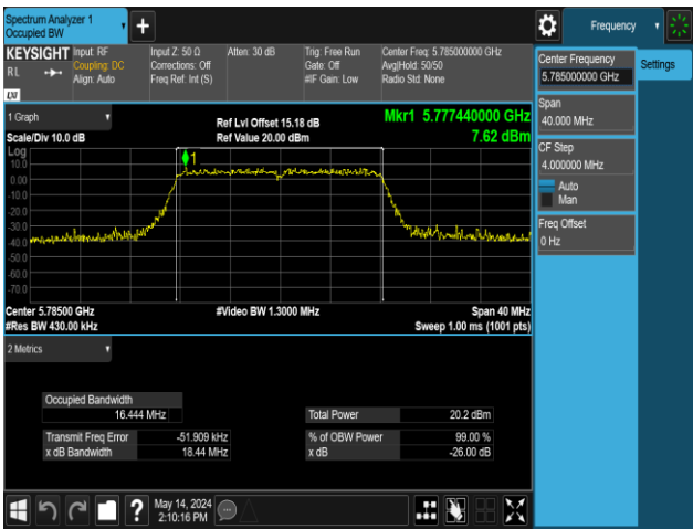
11A-Ant2-5785
