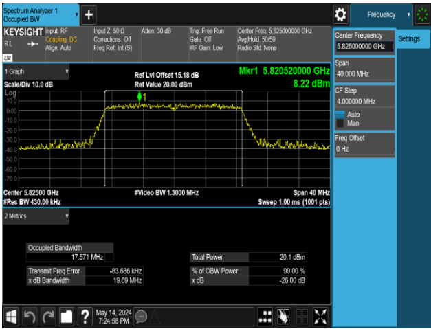
11N20MIMO-Ant2-5825
