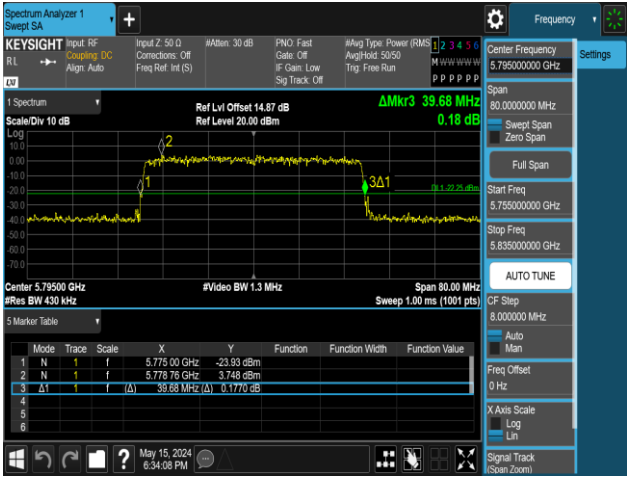
11AX40MIMO-Ant1-5795-242Tone-RU62
