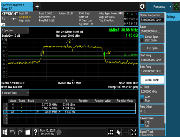
11AC40MIMO-Ant2-5190
