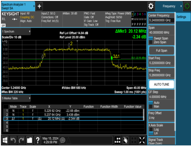
11AX20MIMO-Ant2-5240-106Tone-RU54
