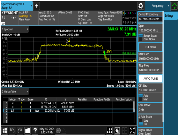
11AC80MIMO-Ant2-5775
