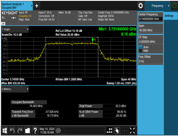
11A-Ant2-5745
