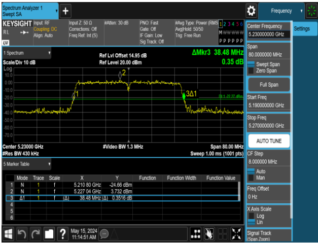
11AC40MIMO-Ant2-5230
