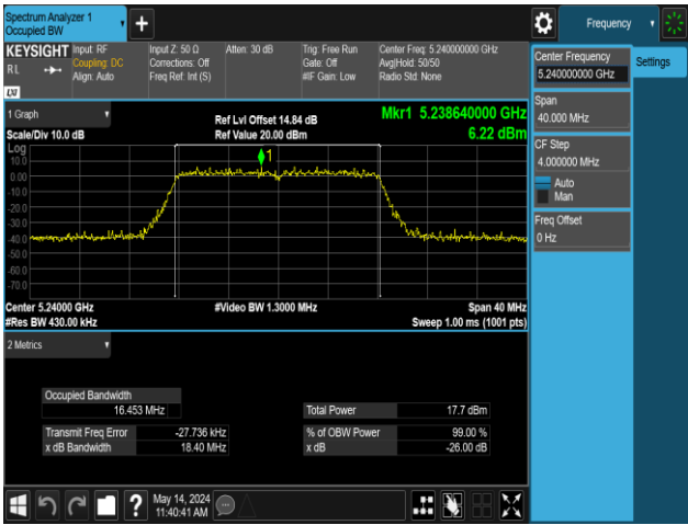
11A-Ant2-5240
