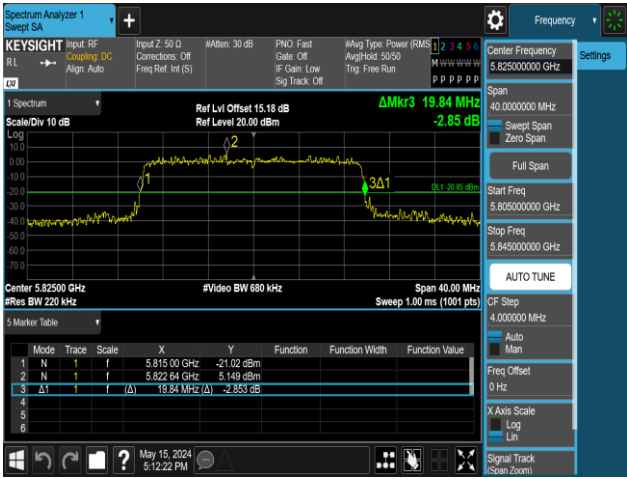
11AX20MIMO-Ant2-5825-106Tone-RU54
