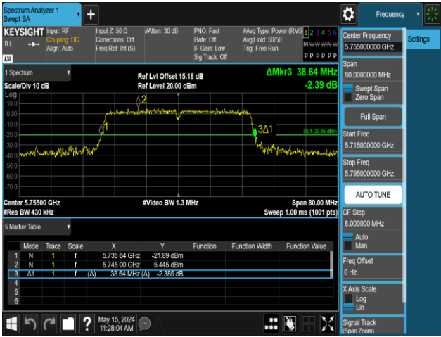
11AC40MIMO-Ant2-5755
