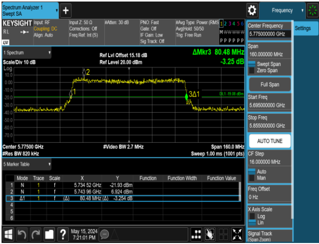
11AX80MIMO-Ant2-5775-484Tone-RU66
