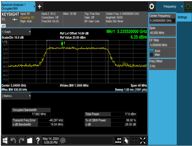
11N20MIMO-Ant2-5240
