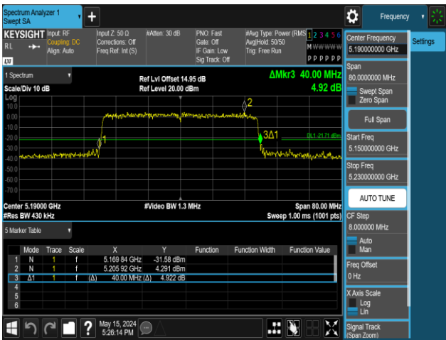
11AX40MIMO-Ant2-5190-242Tone-RU62
