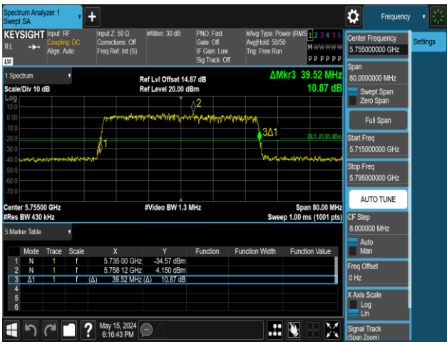
11AX40MIMO-Ant1-5755-242Tone-RU62
