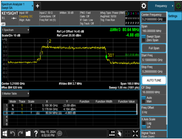
11AX80MIMO-Ant1-5210-484Tone-RU66
