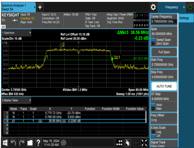
11AC40MIMO-Ant2-5795
