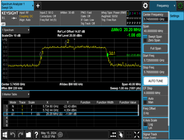
11AX20MIMO-Ant1-5745-106Tone-RU54
