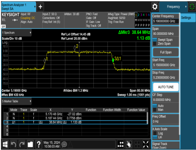
11AC40MIMO-Ant1-5190
