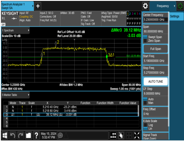
11AX40MIMO-Ant1-5230-242Tone-RU62
