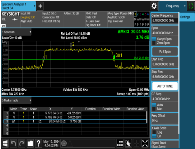
11AX20MIMO-Ant2-5785-106Tone-RU54
