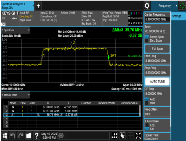
11AX40MIMO-Ant1-5190-242Tone-RU62
