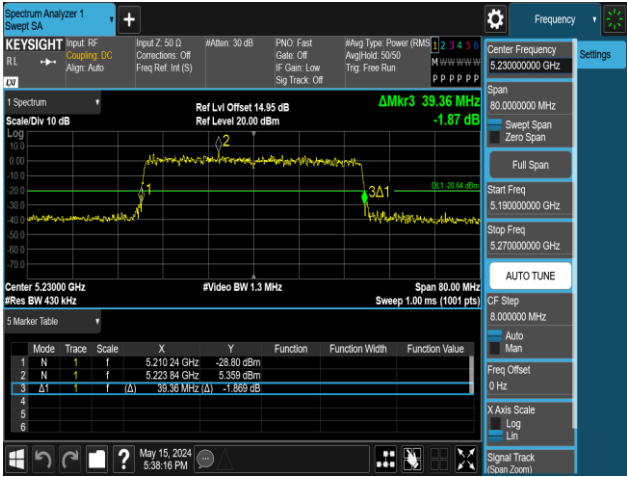
11AX40MIMO-Ant2-5230-242Tone-RU62
