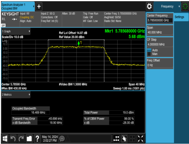
11A-Ant1-5785
