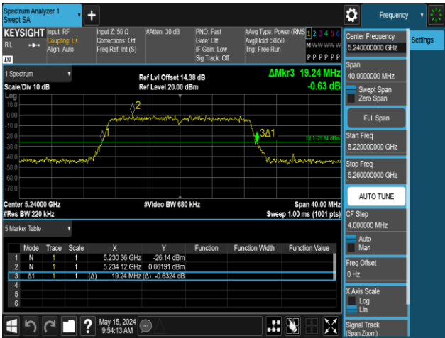
11AC20MIMO-Ant1-5240
