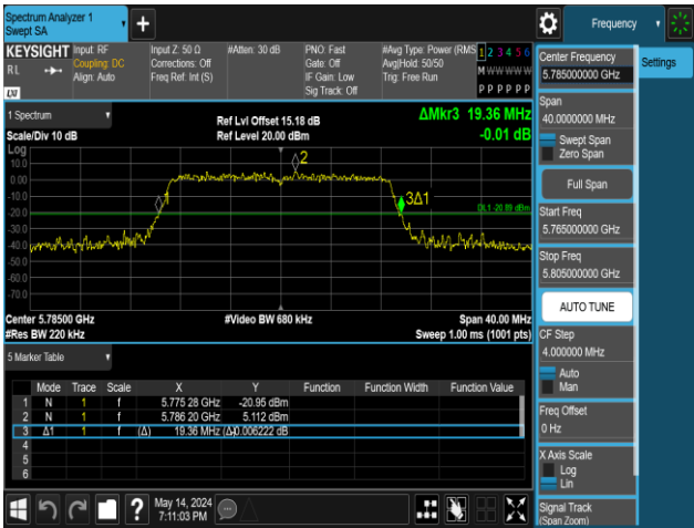
11N20MIMO-Ant2-5785
