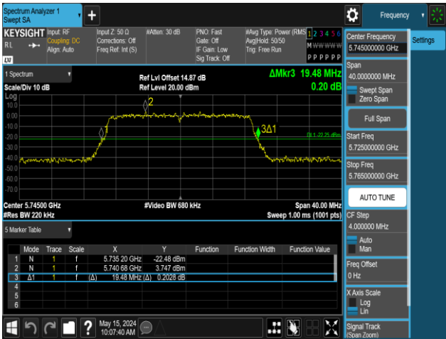
11AC20MIMO-Ant1-5745
