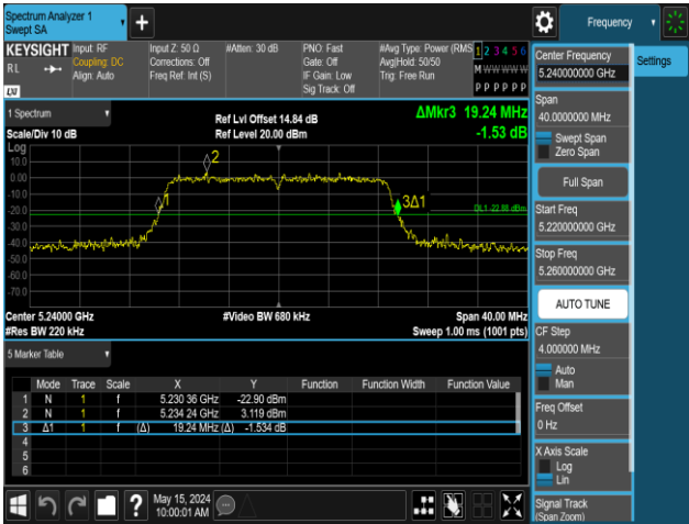
11AC20MIMO-Ant2-5240
