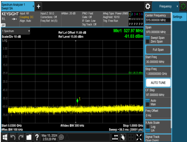
11AX20MIMO-Ant2-2437-106Tone-RU54-30~1000-PASS
