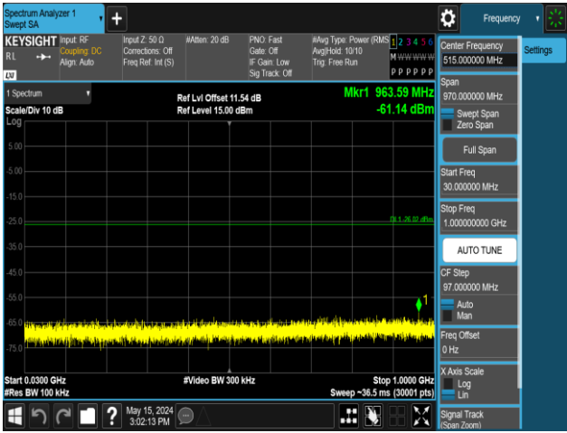
11AX40MIMO-Ant1-2437-242Tone-RU62-30~1000-PASS
