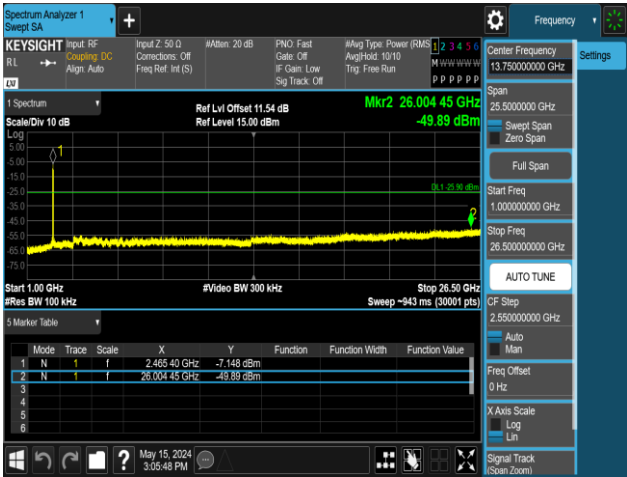
11AX40MIMO-Ant1-2452-242Tone-RU62-1000~26500-PASS
