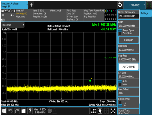
11AX20MIMO-Ant1-2437-106Tone-RU54-30~1000-PASS
