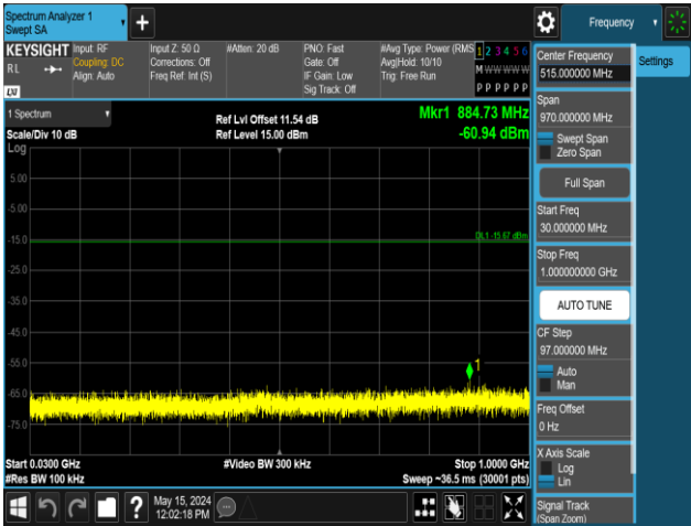
11B-Ant1-2437-30~1000-PASS
