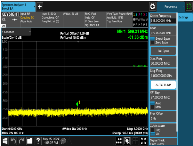
11B-Ant2-2462-30~1000-PASS
