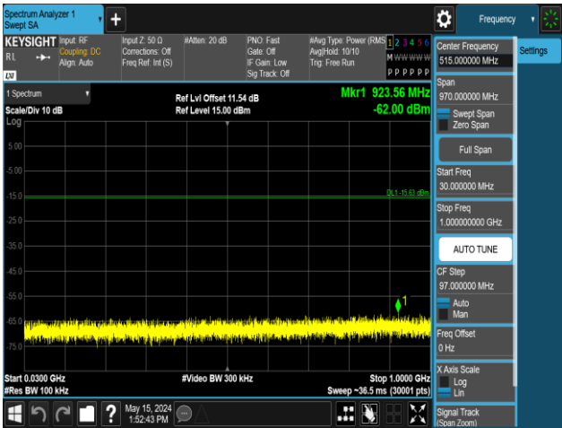
11B-Ant1-2462-30~1000-PASS
