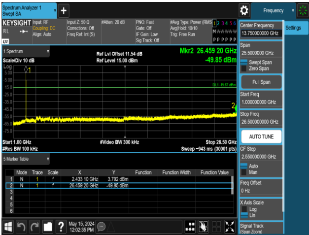
11B-Ant1-2437-1000~26500-PASS
