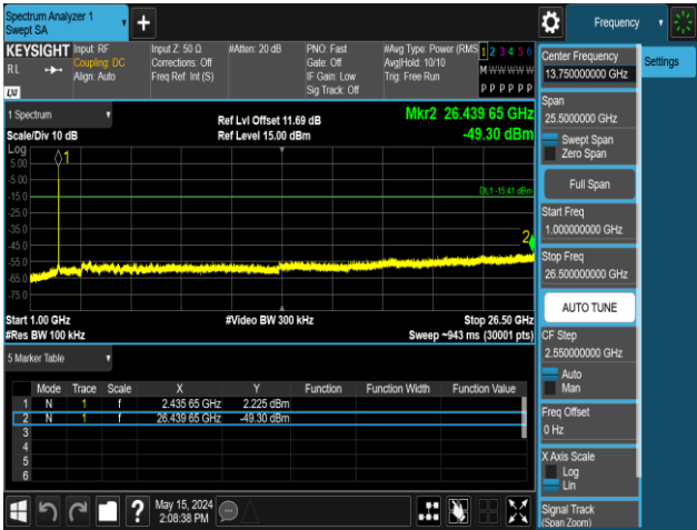
11B-Ant2-2437-1000~26500-PASS
