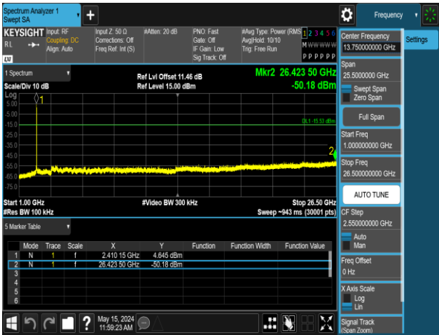
11B-Ant1-2412-1000~26500-PASS
