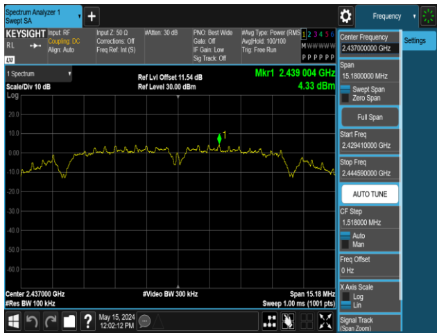
11B-Ant1-2437-PASS
