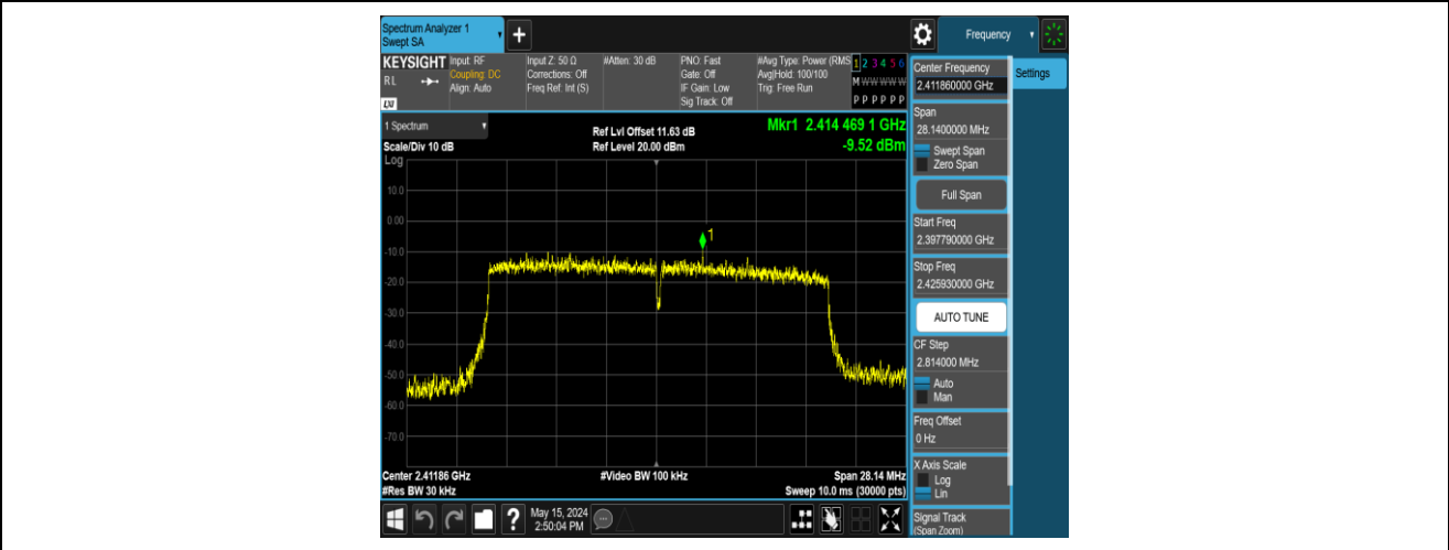
11AX20MIMO-Ant2-2412-106Tone-RU54-PASS
