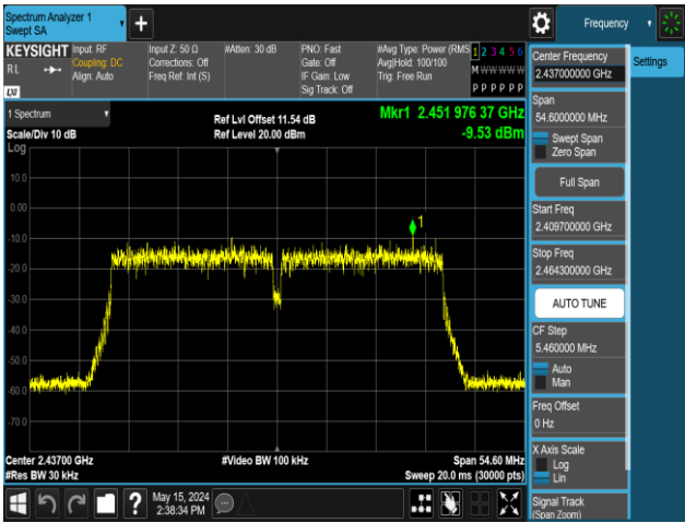
11N40MIMO-Ant1-2437-PASS
