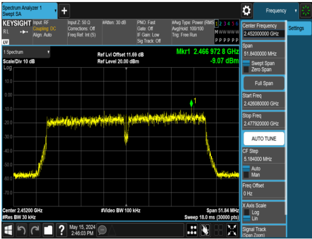
11N40MIMO-Ant2-2452-PASS
