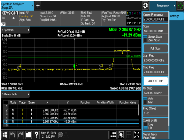
11G-Ant2-2412-PASS
