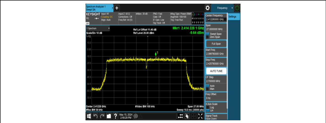
11AX20MIMO-Ant1-2412-106Tone-RU54-PASS
