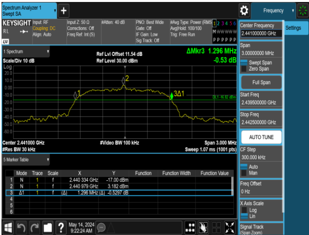
2DH5-Ant1-2441
