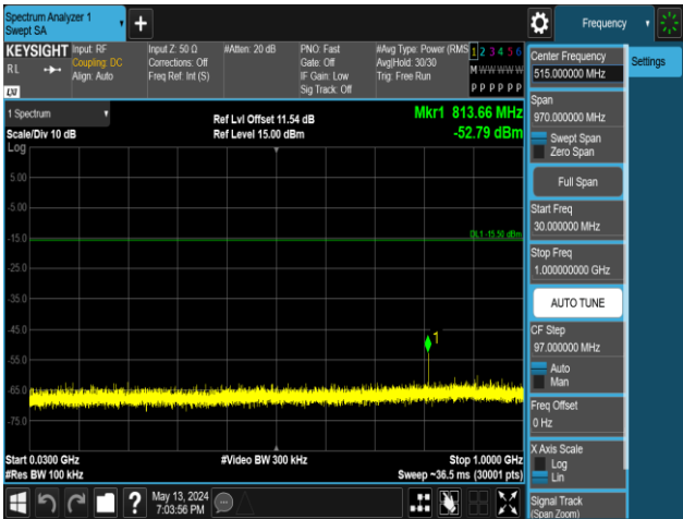
DH5-Ant1-2441-30~1000-PASS
