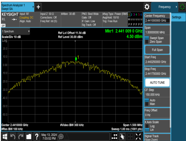
DH5-Ant1-2441-0~Reference-PASS
