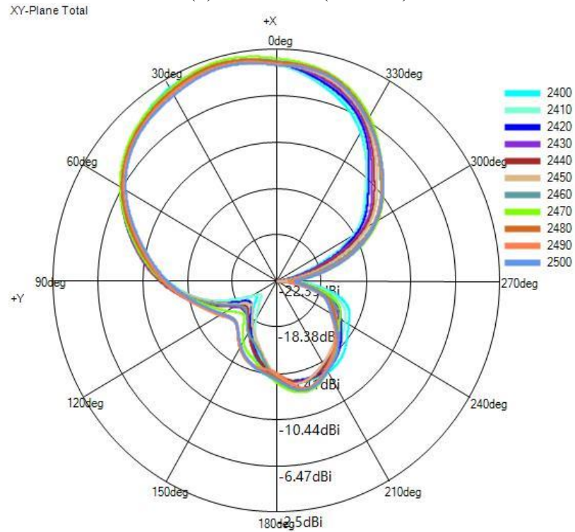
(3) X-Y Plane(unit:dBi):
