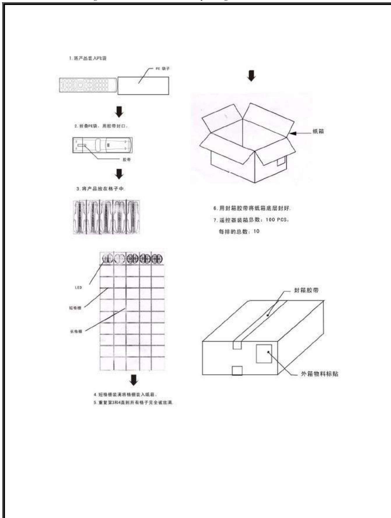
Schematic diagram of remote control package
