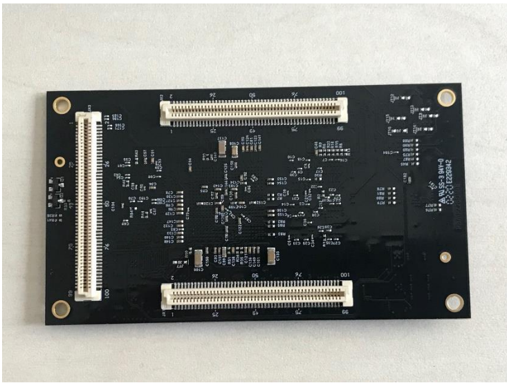
Picozed back
