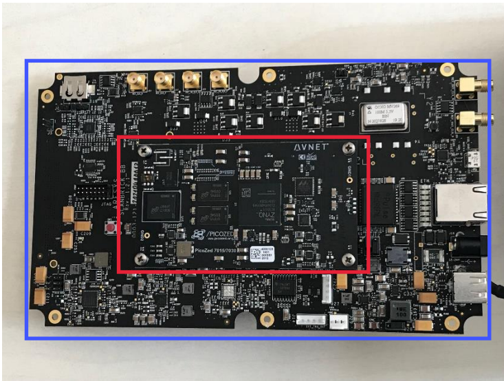
Picozed front
