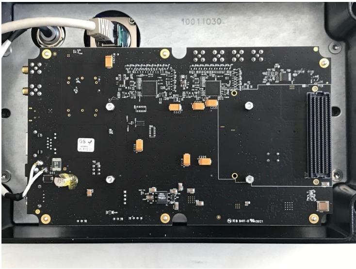
BaseBand back
