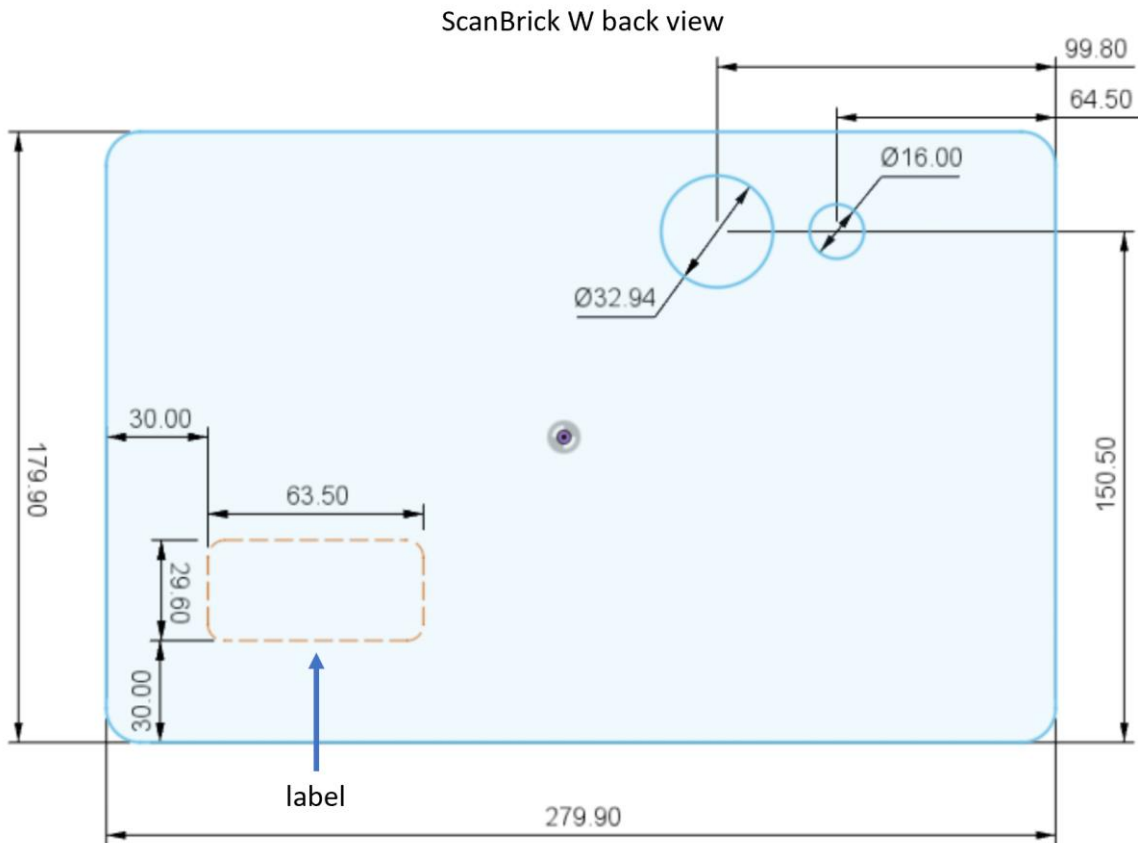
Fig.2 Label position on ScanBrick W® system
