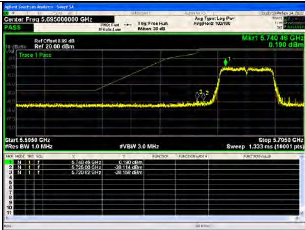
802.11ac(VH20)-5745
