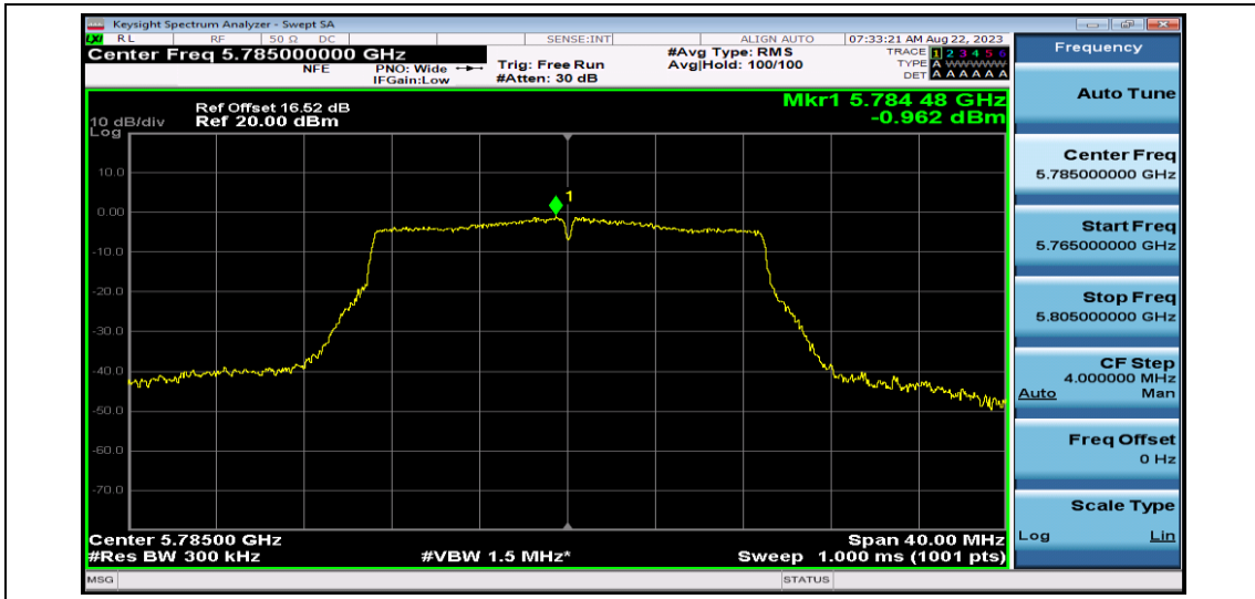
11AC20SISO-Ant1-5785
