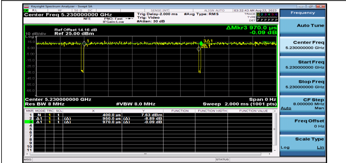
NTNV-11AC40SISO-Ant1-5230
