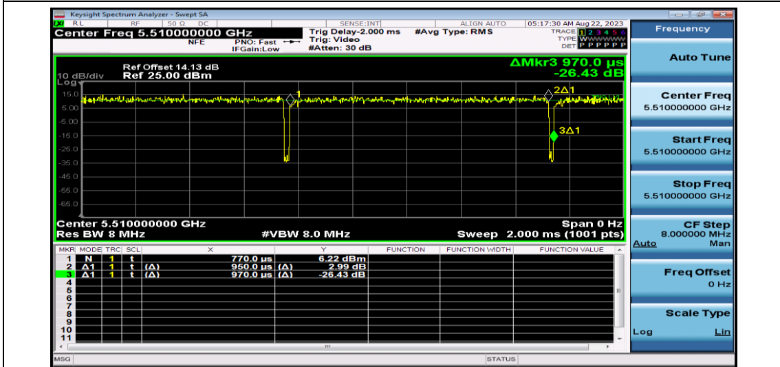
NTNV-11AC40SISO-Ant1-5510
