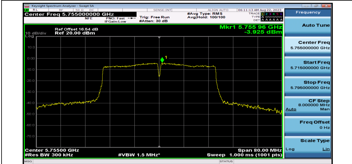
11AC40SISO-Ant1-5755
