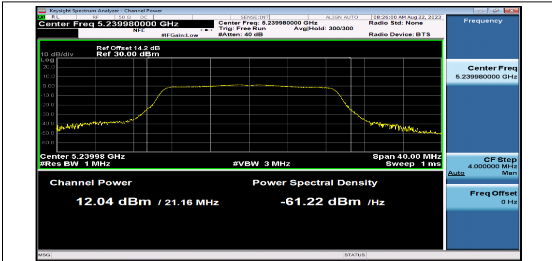
11AC20SISO-Ant1-5240
