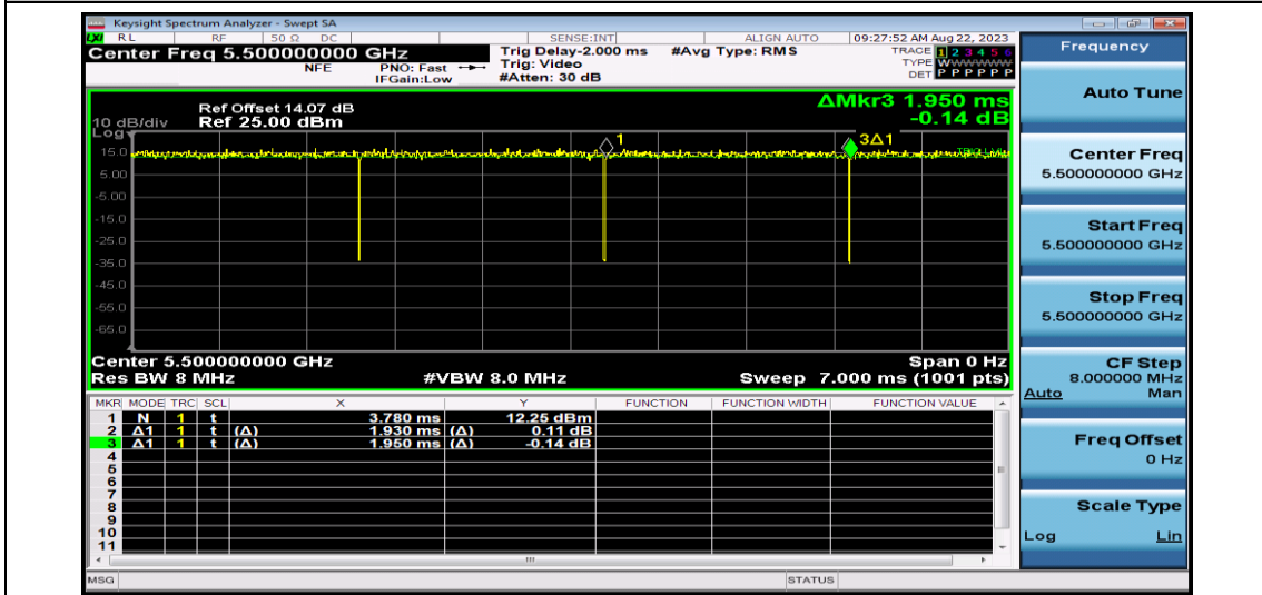
NTNV-11AC20SISO-Ant1-5500
