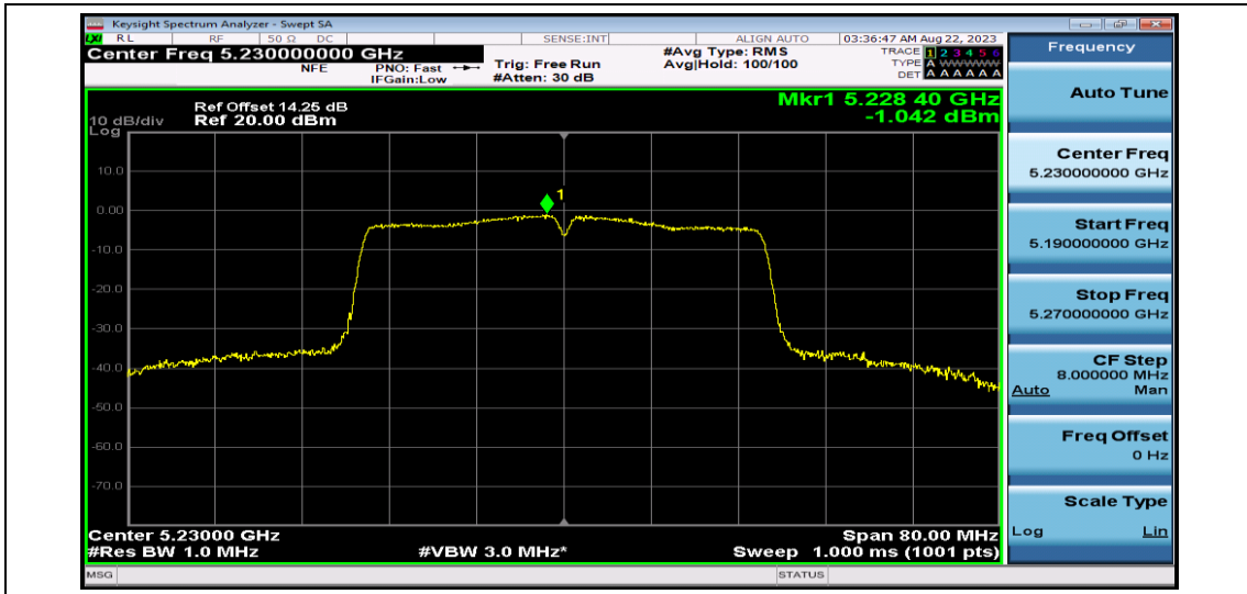
11AC40SISO-Ant1-5230
