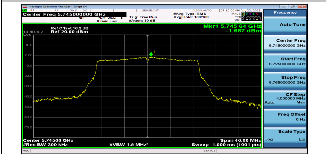
11AC20SISO-Ant1-5745
