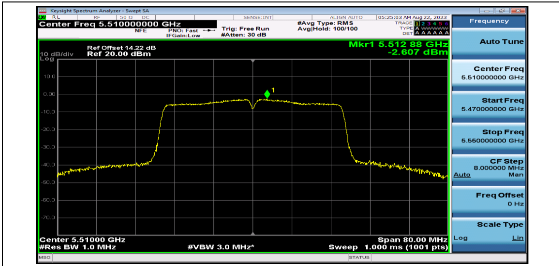
11AC40SISO-Ant1-5510
