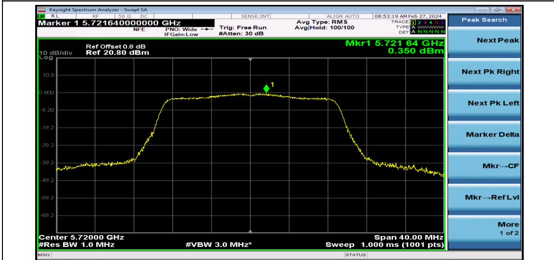
11AC20SISO-Ant1-5720
