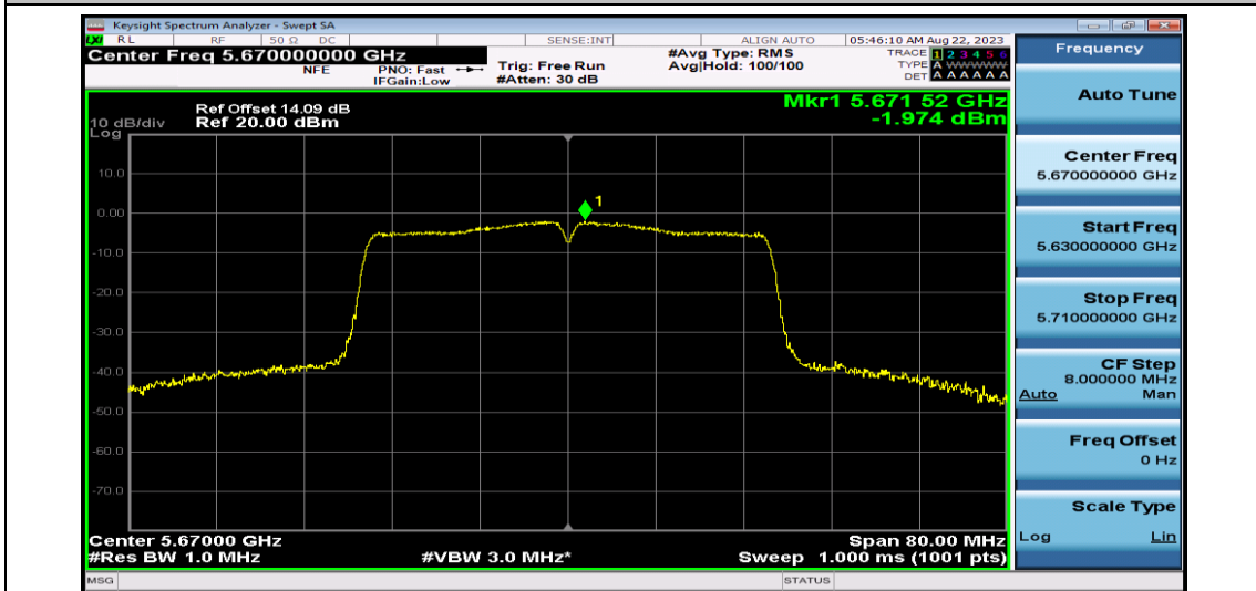
11AC40SISO-Ant1-5670
