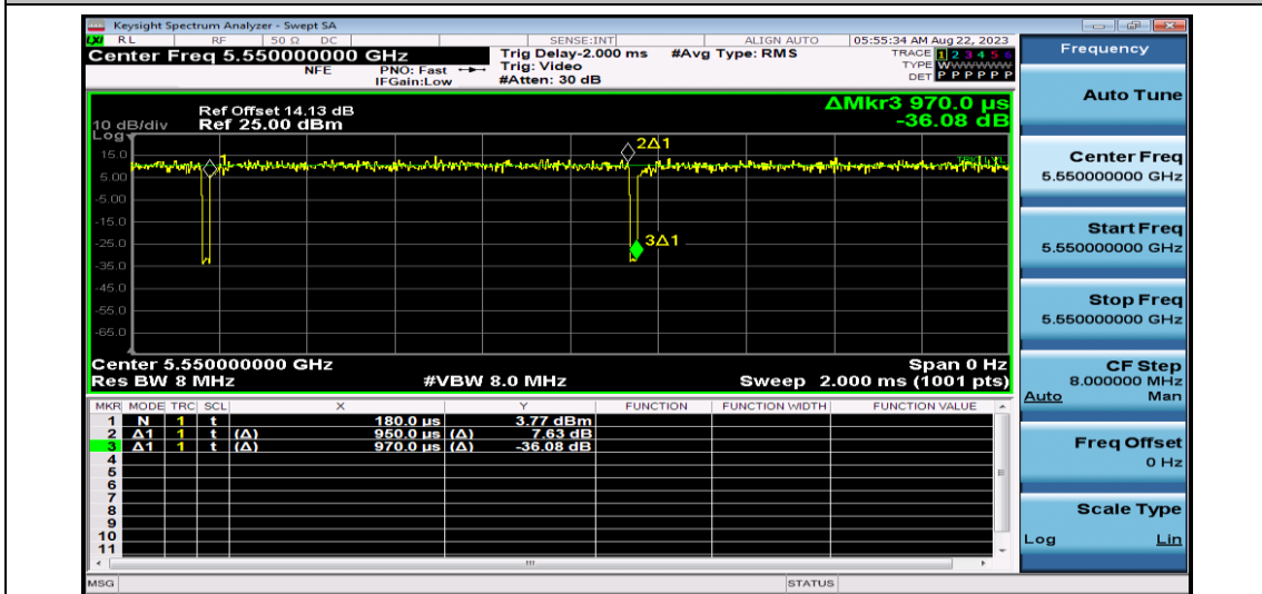
NTNV-11AC40SISO-Ant1-5550
