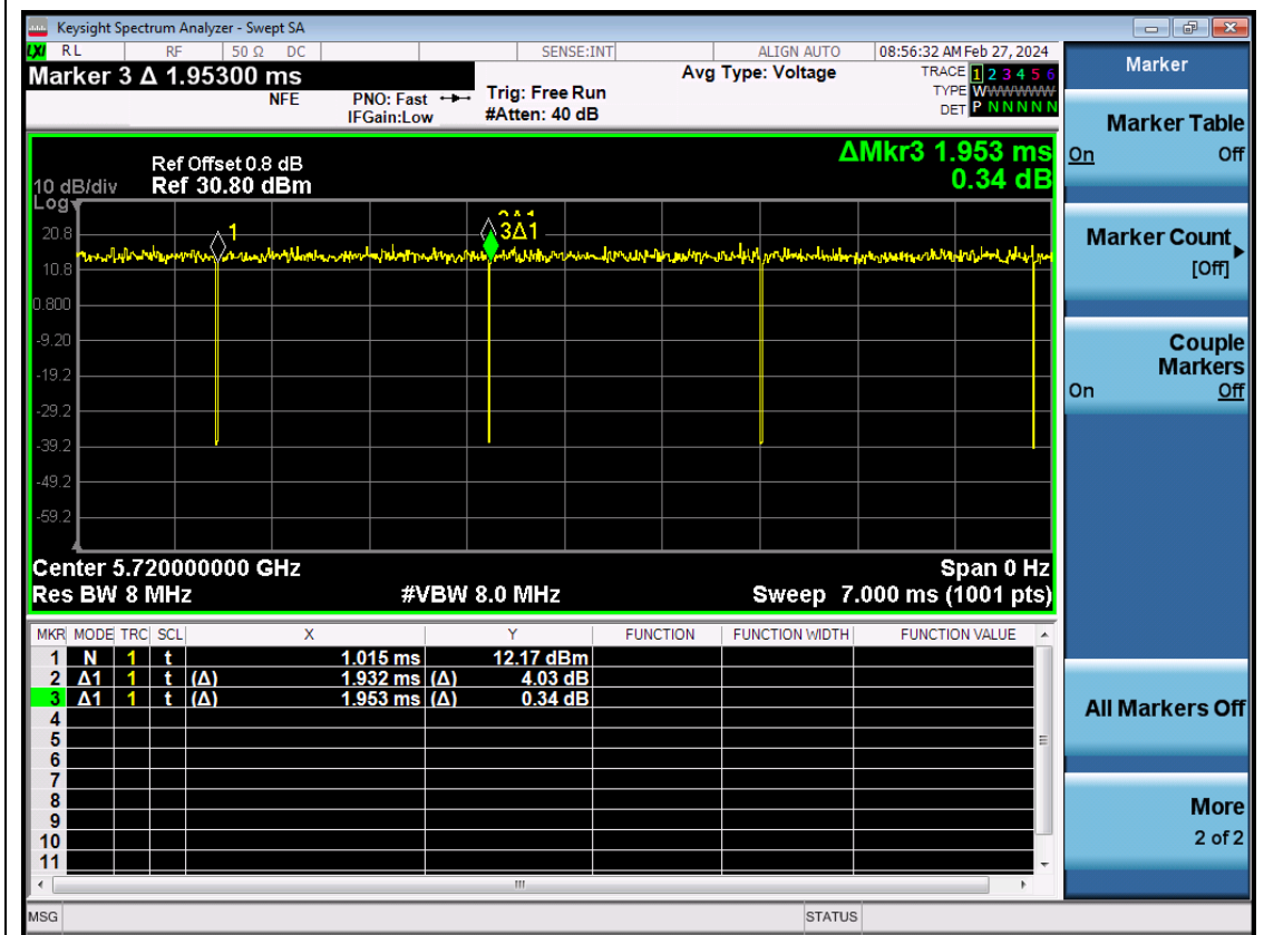
NTNV-11AC20SISO-Ant1-5720
