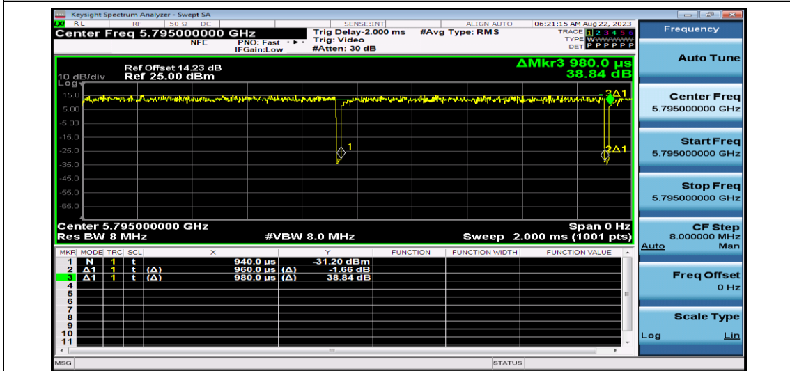
NTV-11AC40SISO-Ant1-5795
