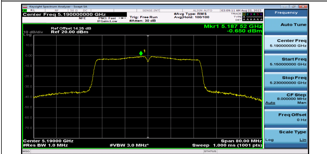
11AC40SISO-Ant1-5190
