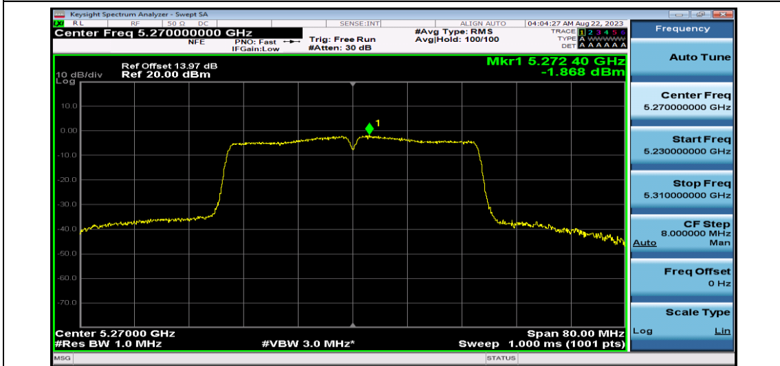
11AC40SISO-Ant1-5270
