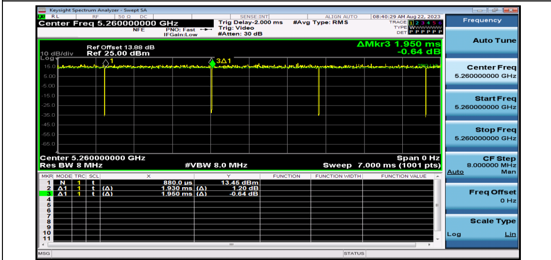
NTNV-11AC20SISO-Ant1-5260
