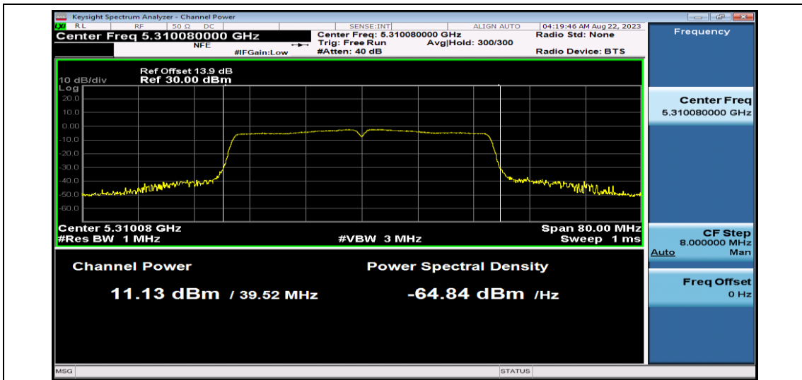
11AC40SISO-Ant1-5310
