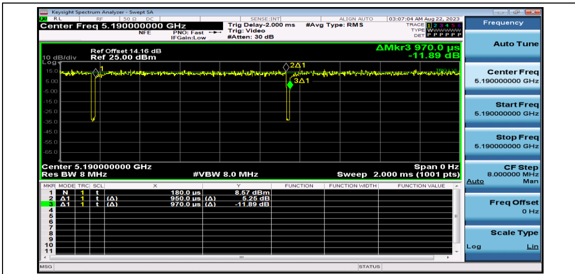
NTNV-11AC40SISO-Ant1-5190
