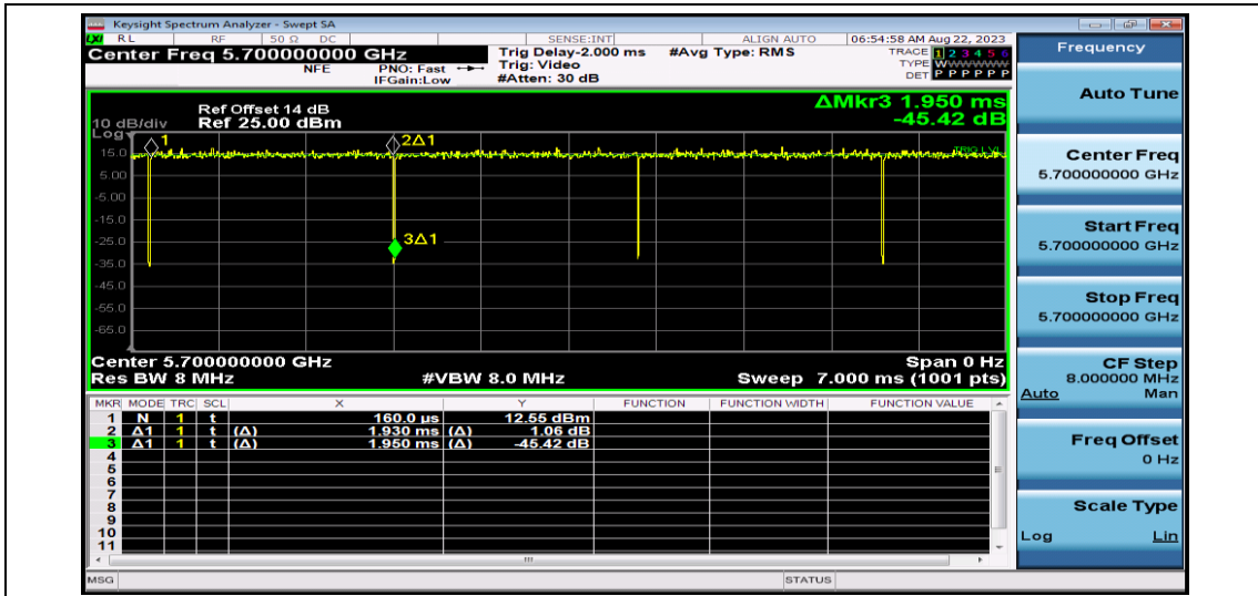
NTNV-11AC20SISO-Ant1-5700
