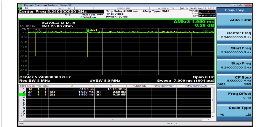
NTNV-11AC20SISO-Ant1-5240
