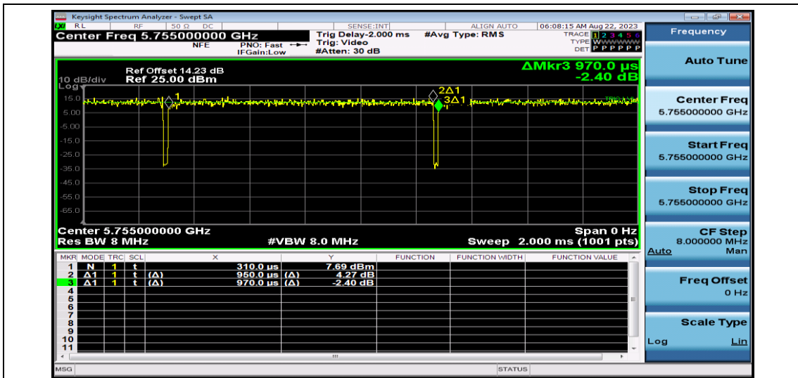
NTV-11AC40SISO-Ant1-5755
