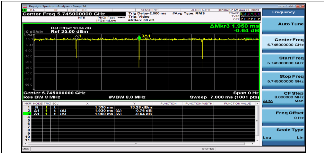
NTV-11AC20SISO-Ant1-5745
