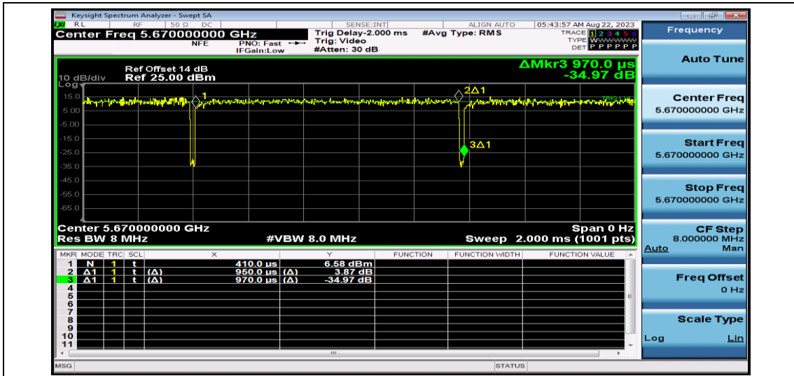
NTNV-11AC40SISO-Ant1-5670
