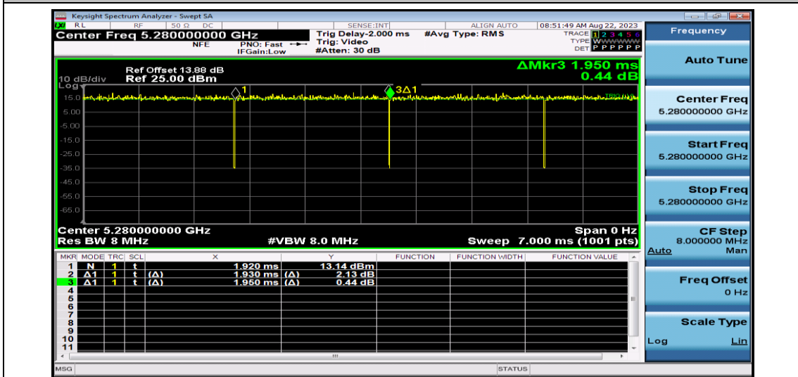
NTNV-11AC20SISO-Ant1-5280
