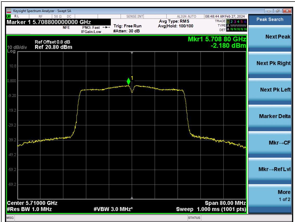
11AC40SISO-Ant1-5710
