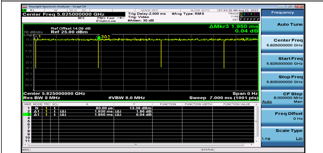
NTV-11AC20SISO-Ant1-5825
