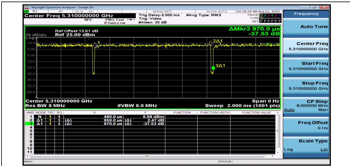
NTNV-11AC40SISO-Ant1-5310
