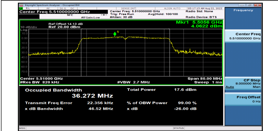
11AC40SISO-Ant1-5510
