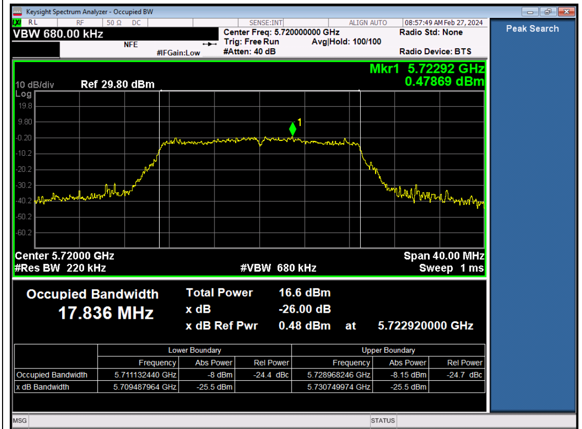
11AC20SISO-Ant1-5720
