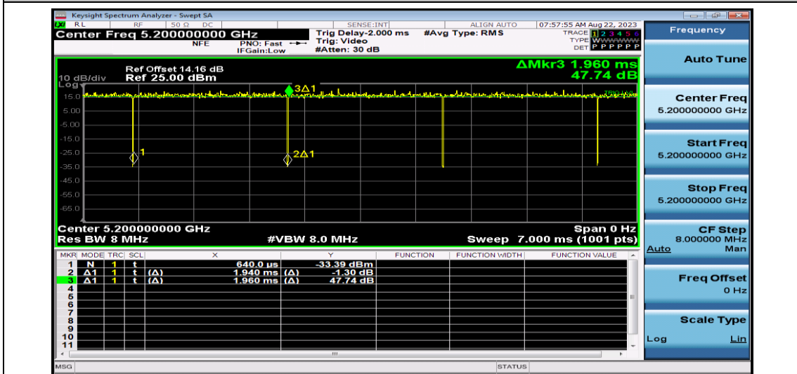
NTNV-11AC20SISO-Ant1-5200
