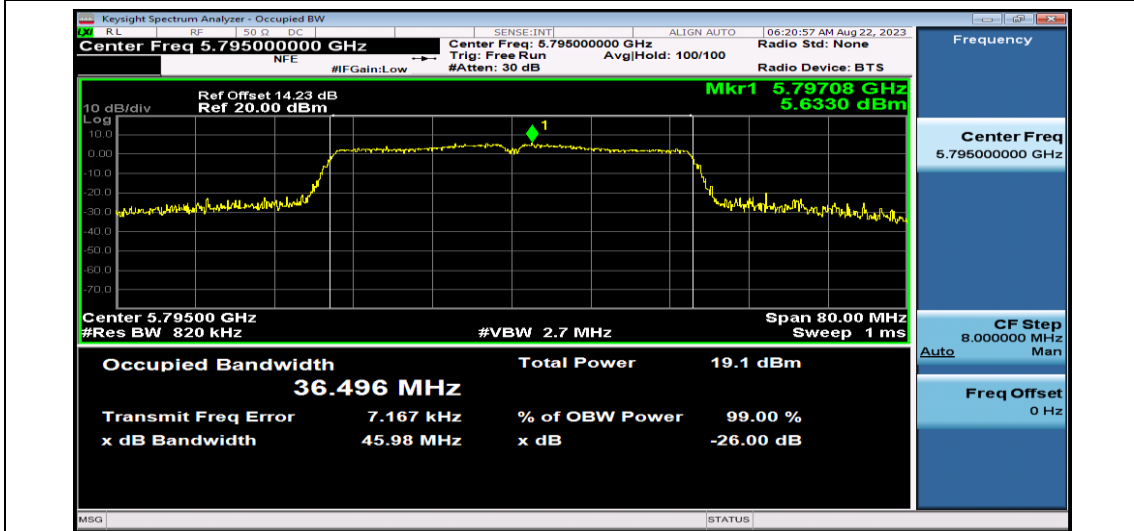
11AC40SISO-Ant1-5795
