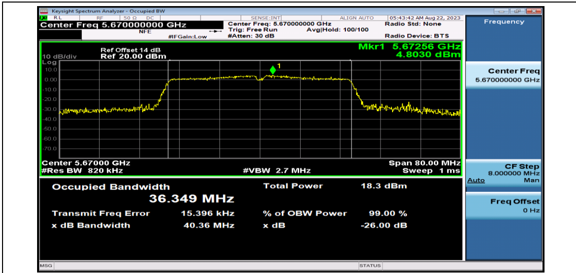
11AC40SISO-Ant1-5670
