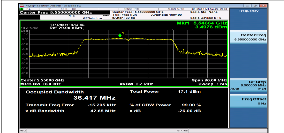
11AC40SISO-Ant1-5550
