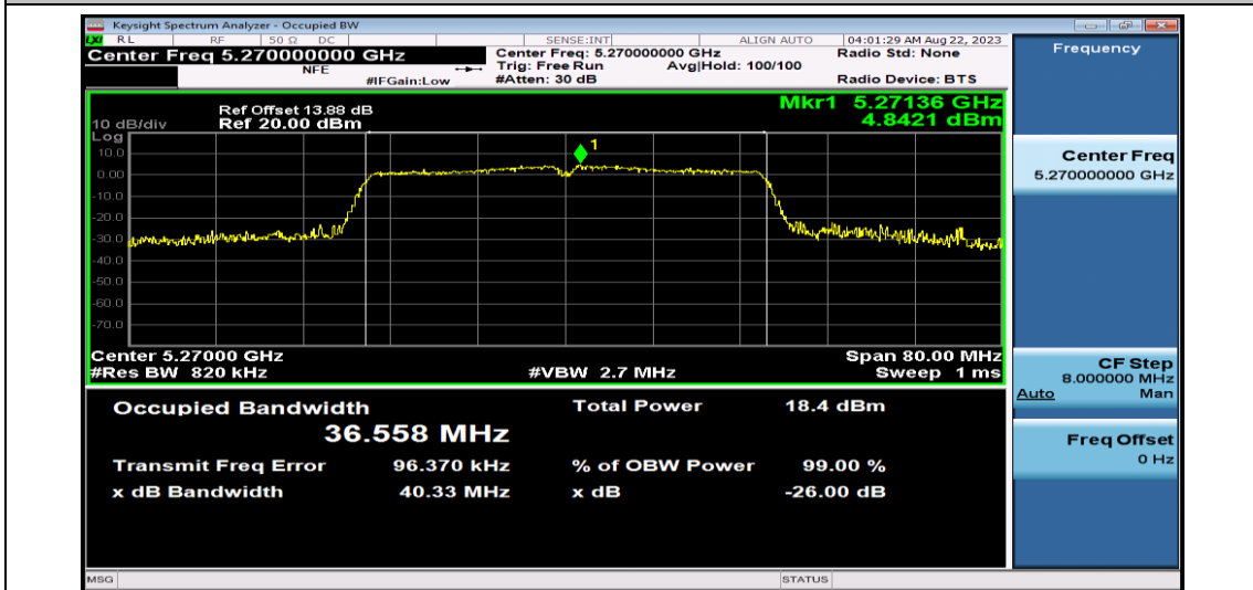
11AC40SISO-Ant1-5270
