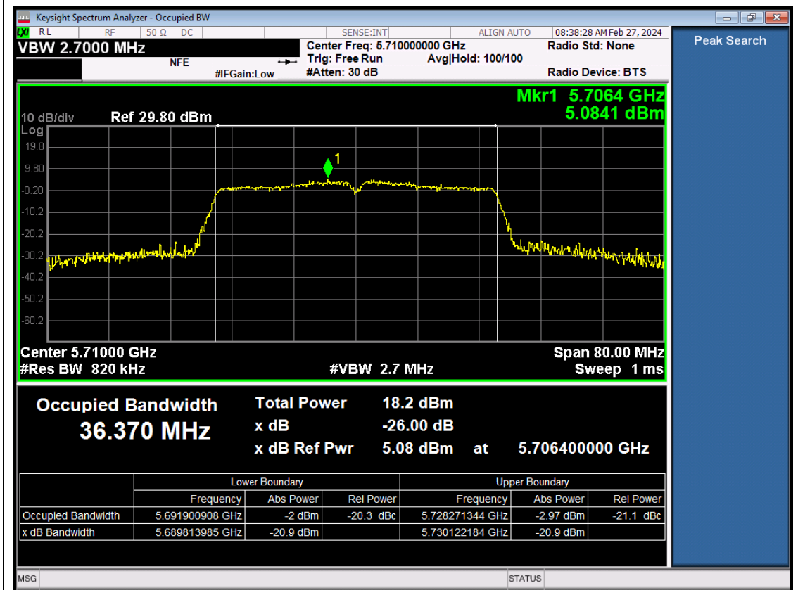
11AC40SISO-Ant1-5710
