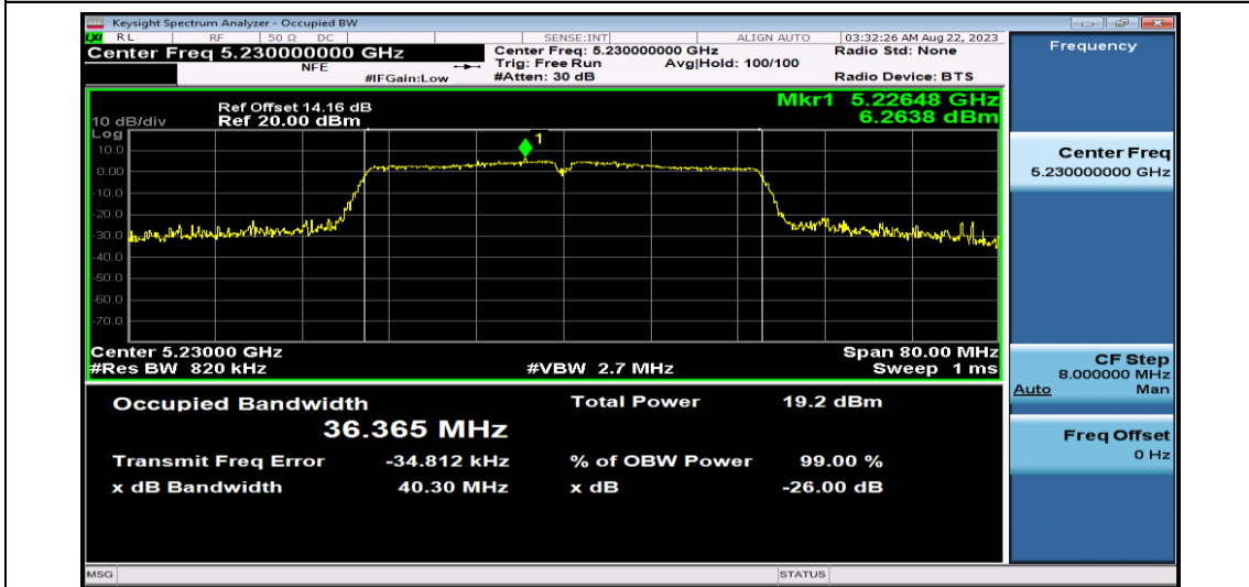
11AC40SISO-Ant1-5230
