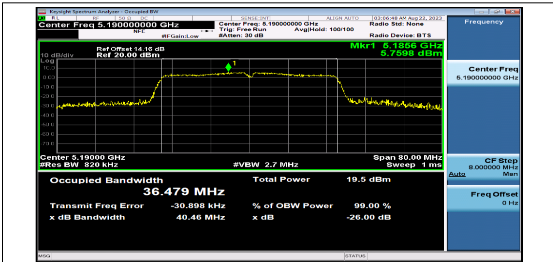
11AC40SISO-Ant1-5190
