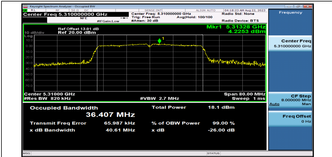
11AC40SISO-Ant1-5310
