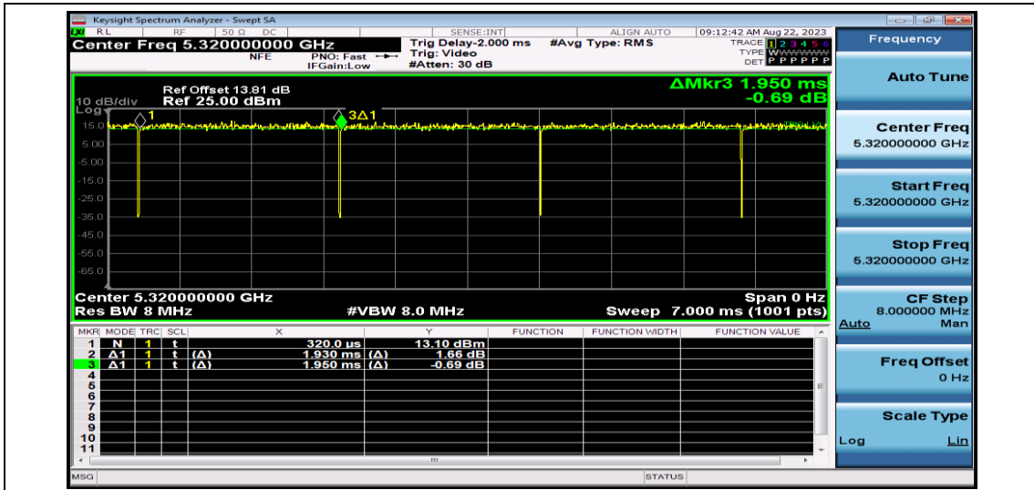
NTNV-11AC20SISO-Ant1-5320
