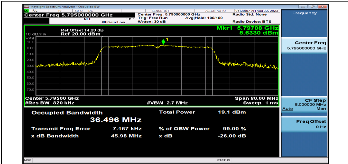
11AC40SISO-Ant1-5795
