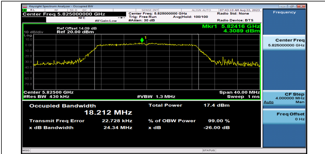
11AC20SISO-Ant1-5825
