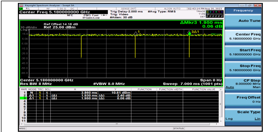
NTNV-11AC20SISO-Ant1-5180
