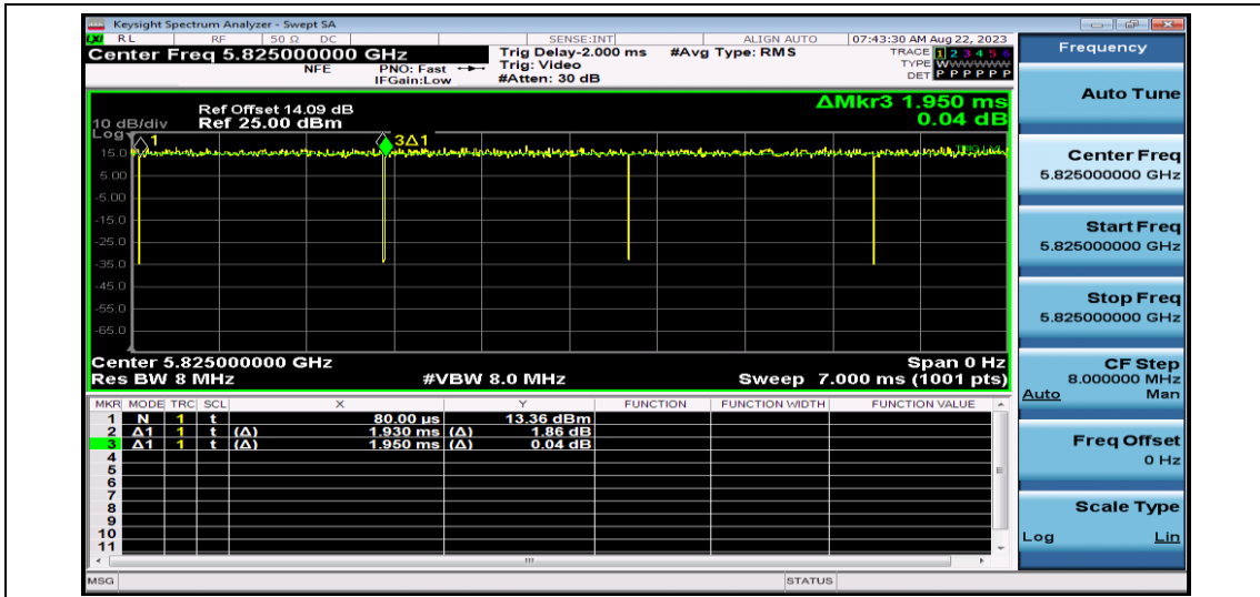
NTNV-11AC20SISO-Ant1-5825
