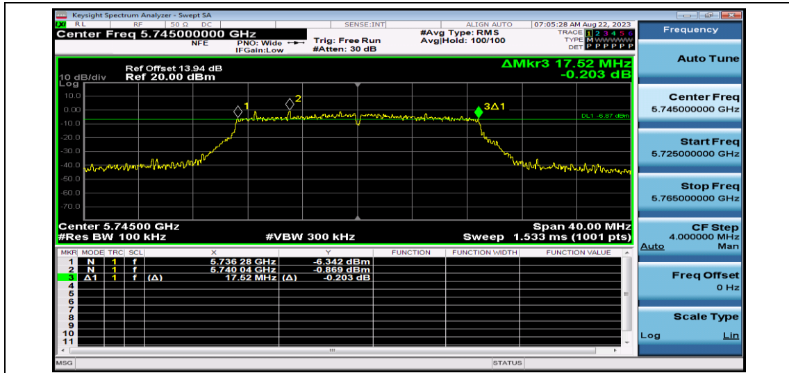
11AC20SISO-Ant1-5745
