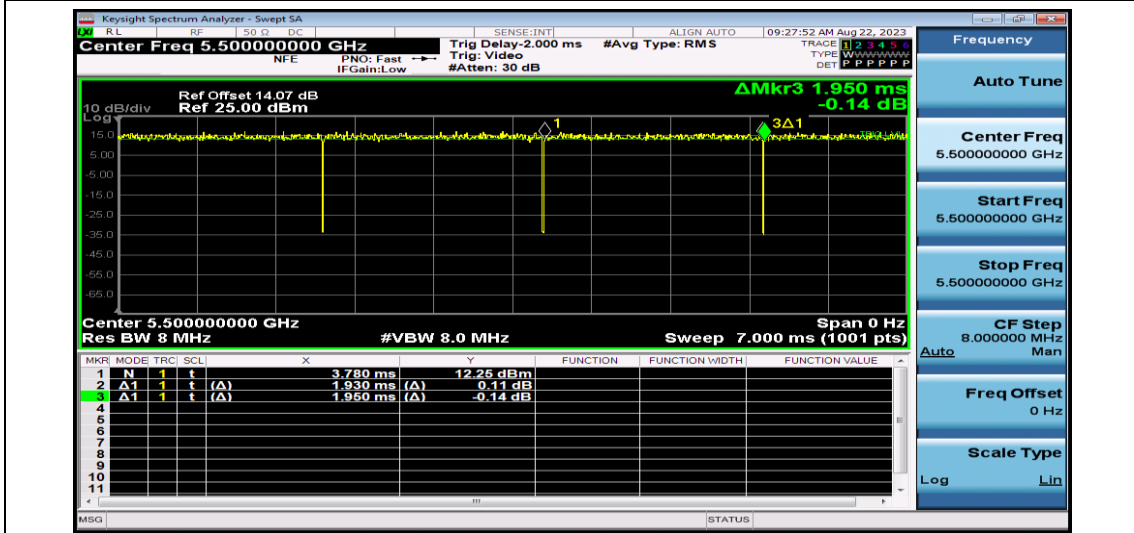
NTNV-11AC20SISO-Ant1-5500
