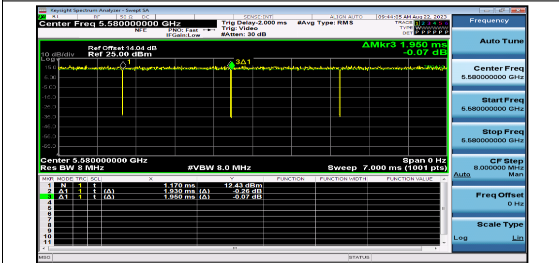
NTNV-11AC20SISO-Ant1-5580
