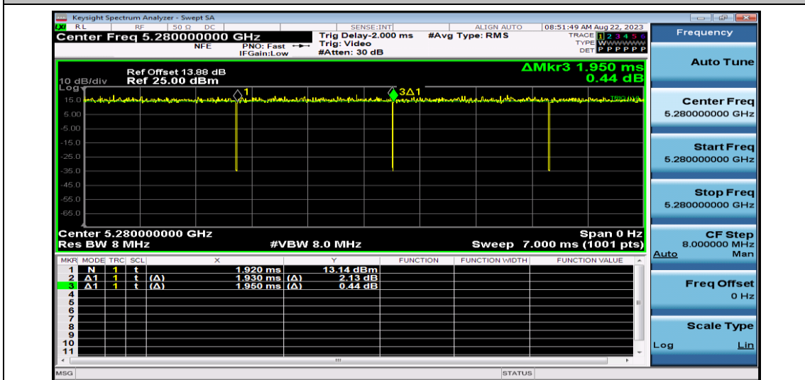
NTV-11AC20SISO-Ant1-5280
