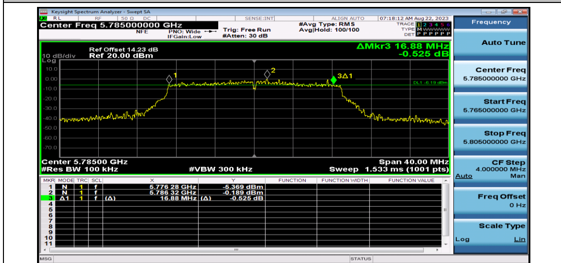
11AC20SISO-Ant1-5785
