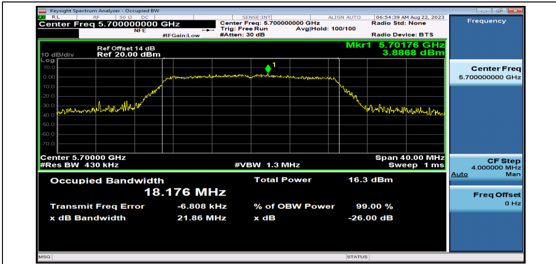
11AC20SISO-Ant1-5700
