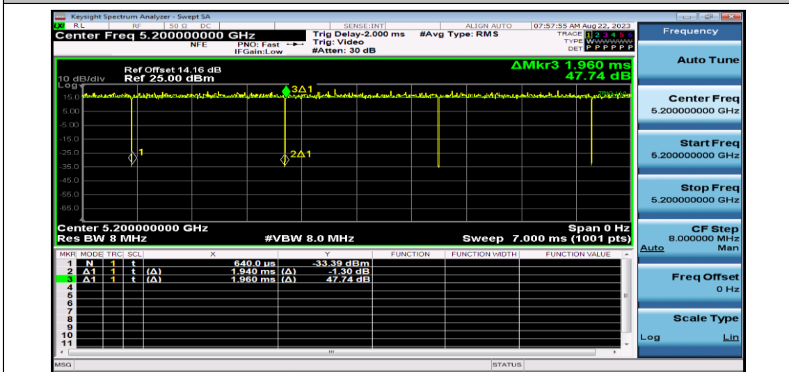
NTNV-11AC20SISO-Ant1-5200
