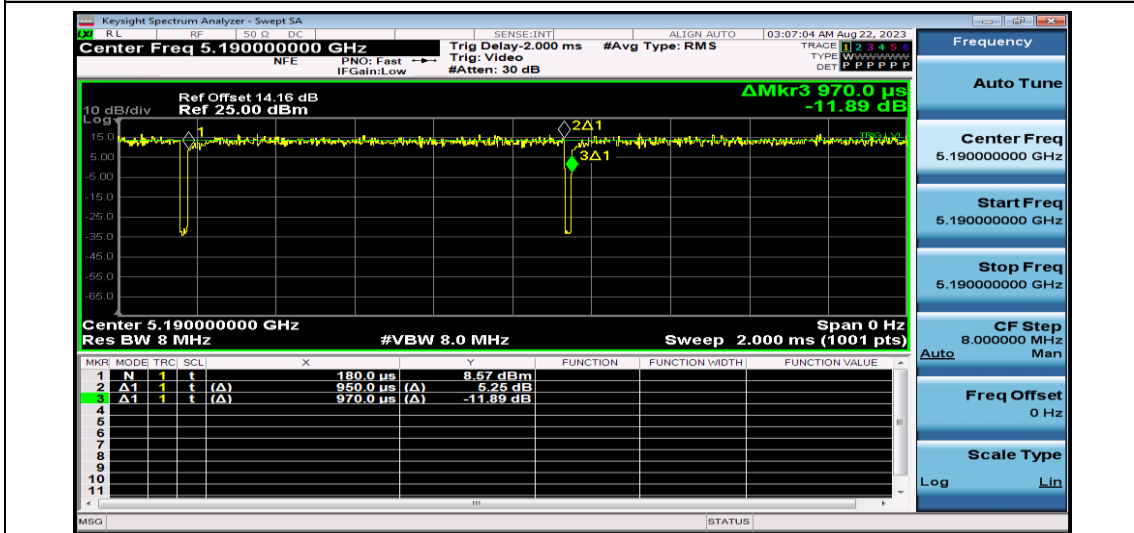
NTNV-11AC40SISO-Ant1-5190
