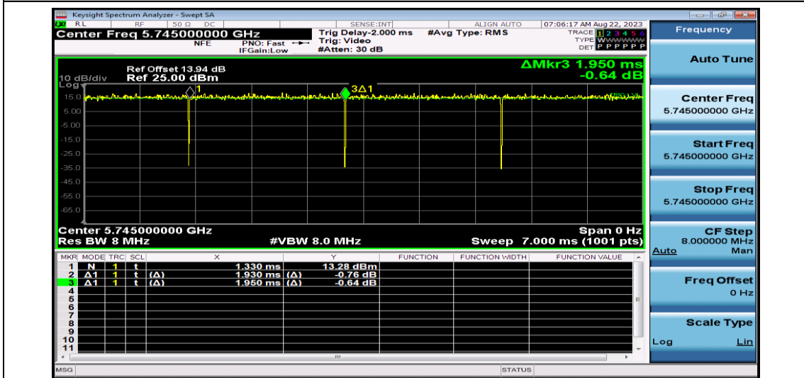
NTV-11AC20SISO-Ant1-5745
