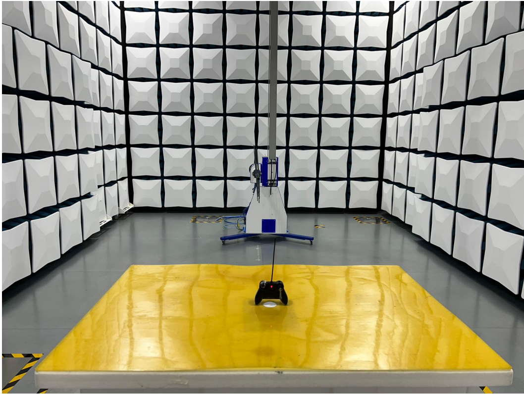
Set-up of Radiation Emission from 200 – 1000MHz
