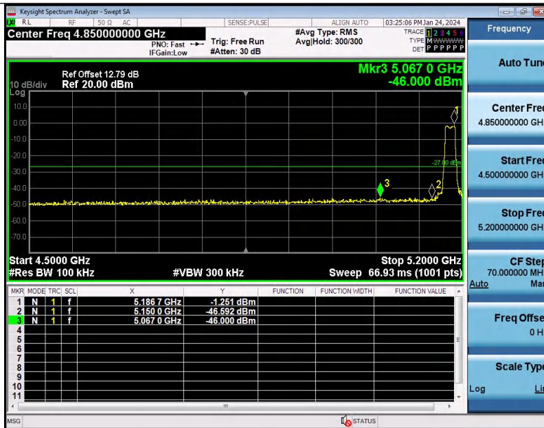
11A-Ant1-5180-PASS
