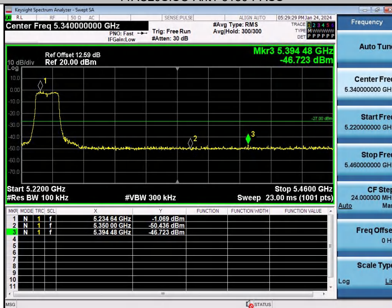
11A20SISO-Ant1-5240-PASS
