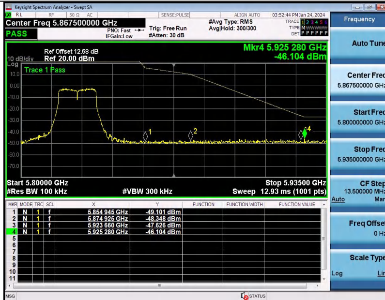
11A-Ant1-5825-PASS
