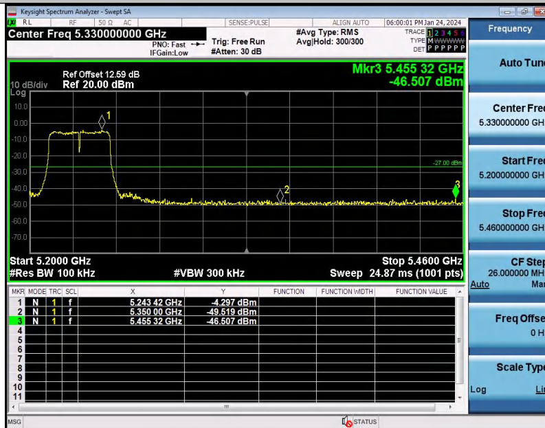
11AC40SISO-Ant1-5230-PASS
