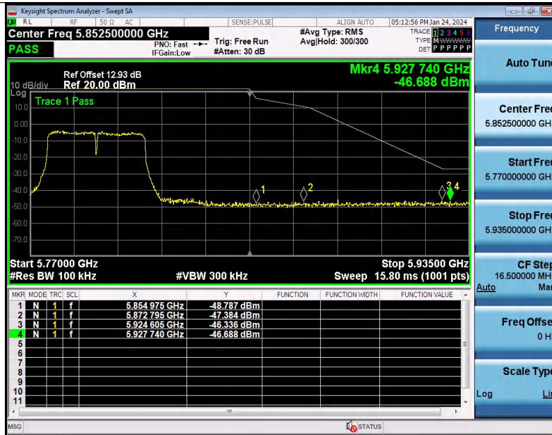
11N40SISO-Ant1-5795-PASS
