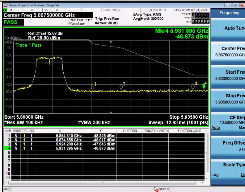
11N20SISO-Ant1-5825-PASS
