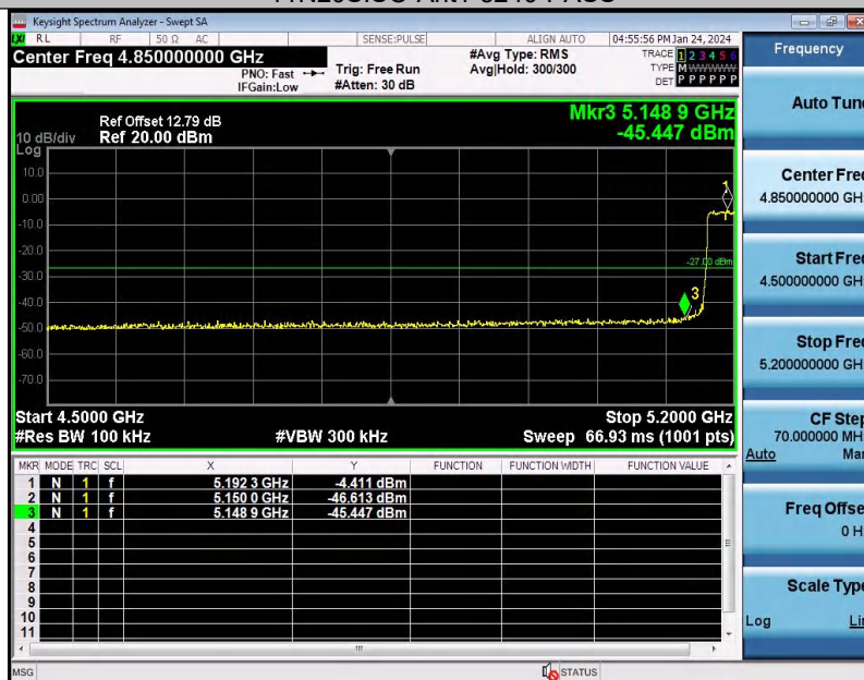
11N40SISO-Ant1-5190-PASS
