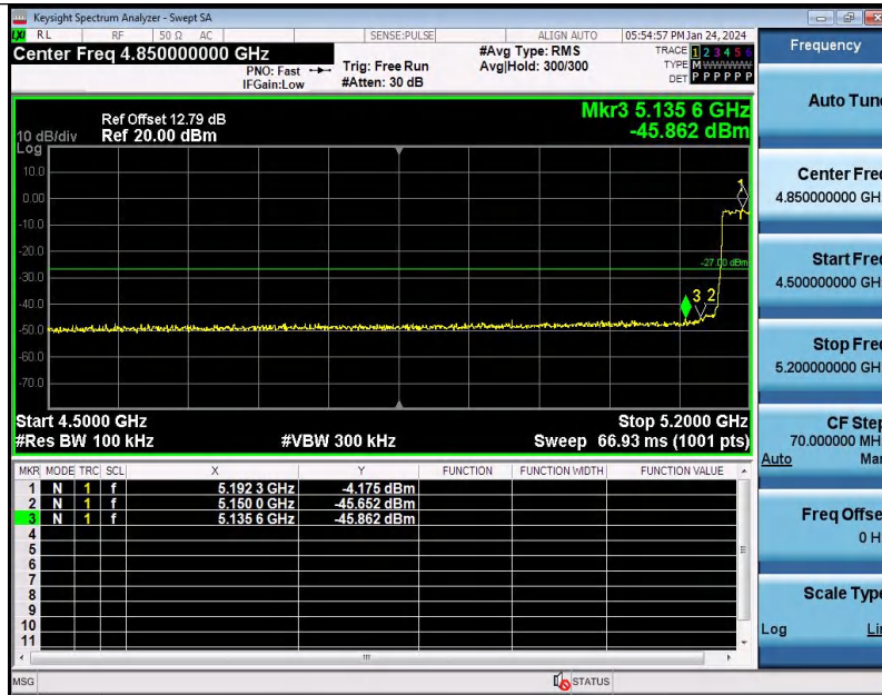
11AC40SISO-Ant1-5190-PASS
