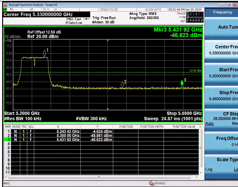
11N40SISO-Ant1-5230-PASS
