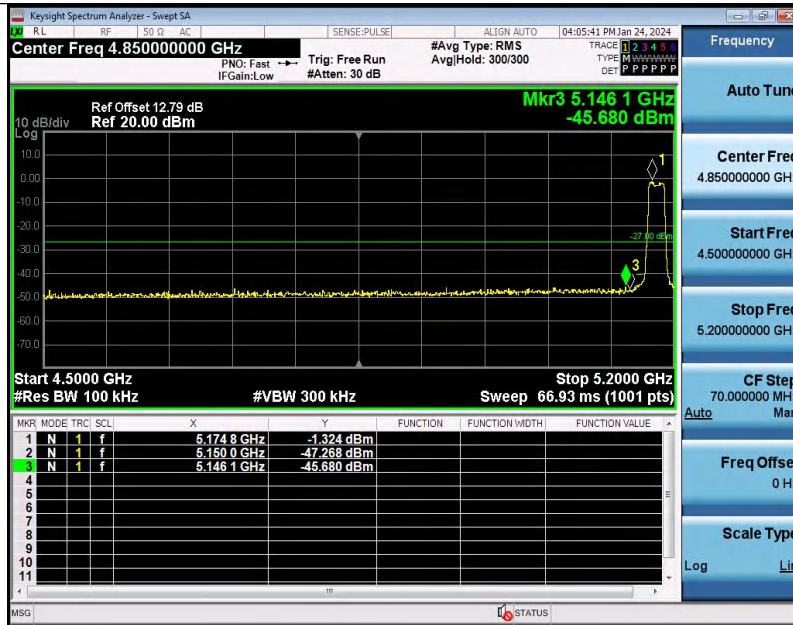
11N20SISO-Ant1-5180-PASS
