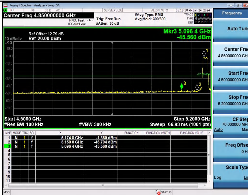
11A20SISO-Ant1-5180-PASS
