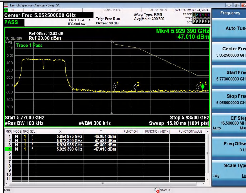
11AC40SISO-Ant1-5795-PASS
