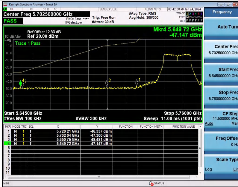
11A-Ant1-5745-PASS
