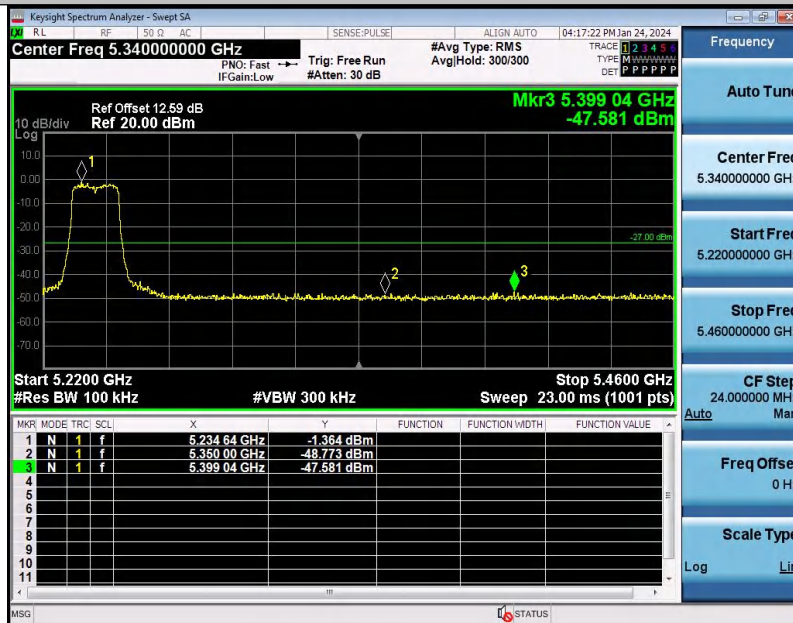
11N20SISO-Ant1-5240-PASS
