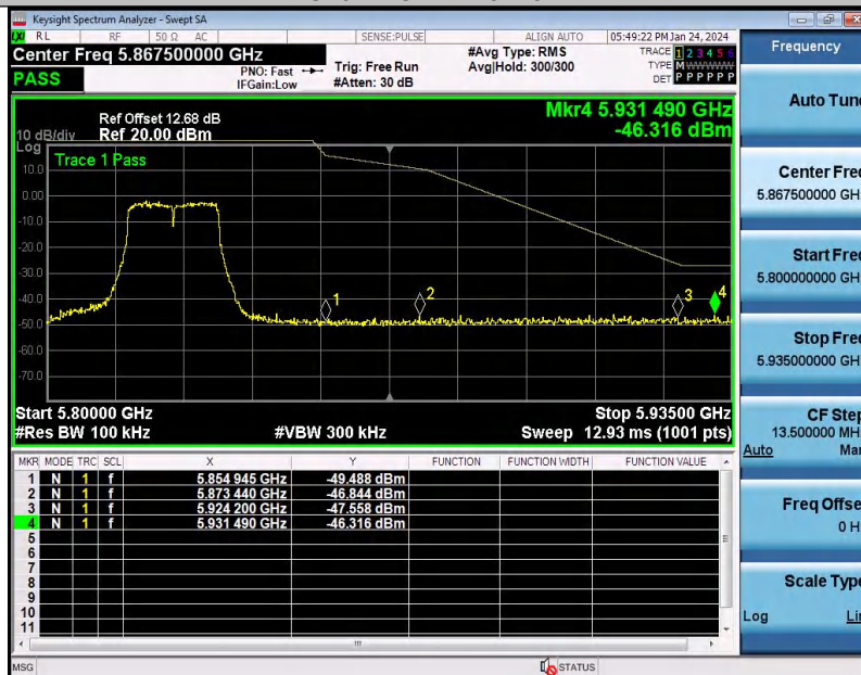
11A20SISO-Ant1-5825-PASS
