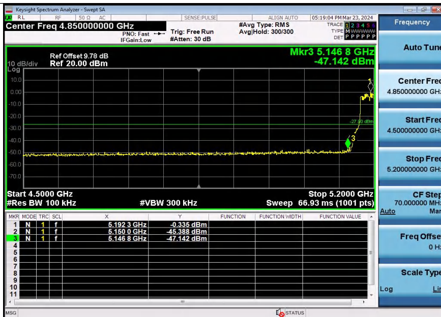
11AC40SISO-Ant1-5190-PASS
