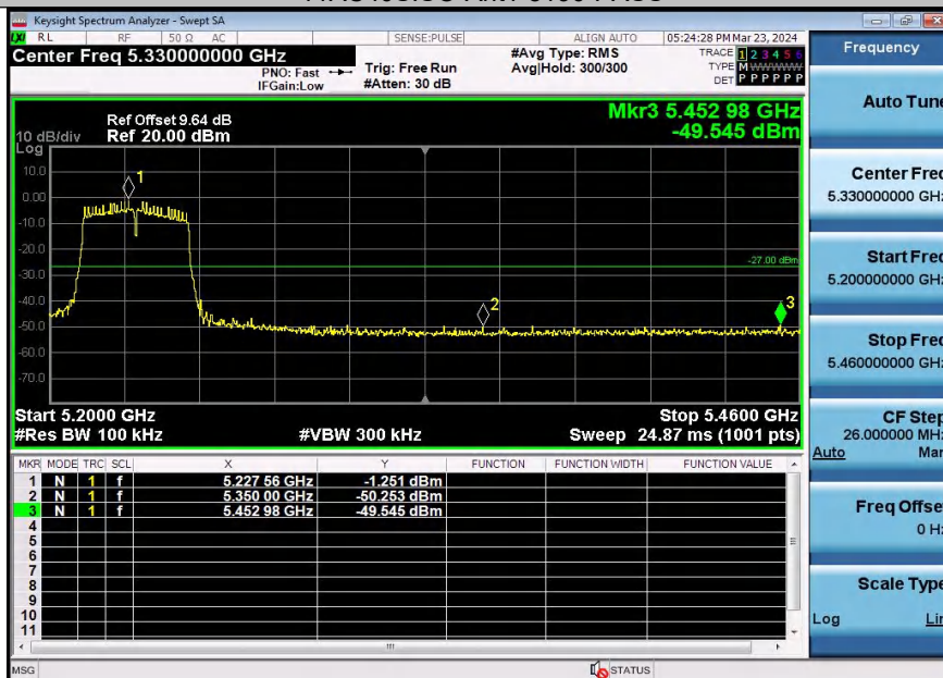
11AC40SISO-Ant1-5230-PASS
