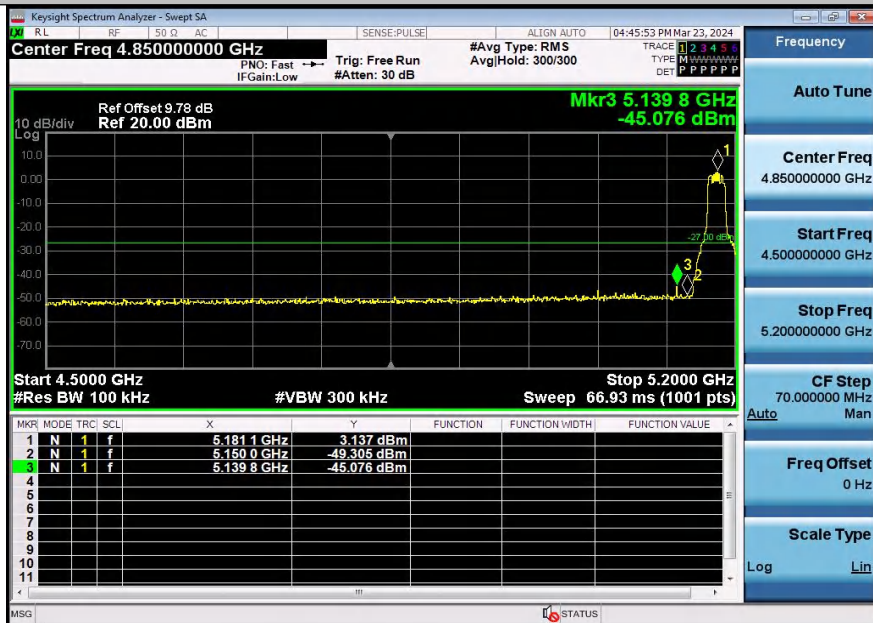
11A20SISO-Ant1-5180-PASS
