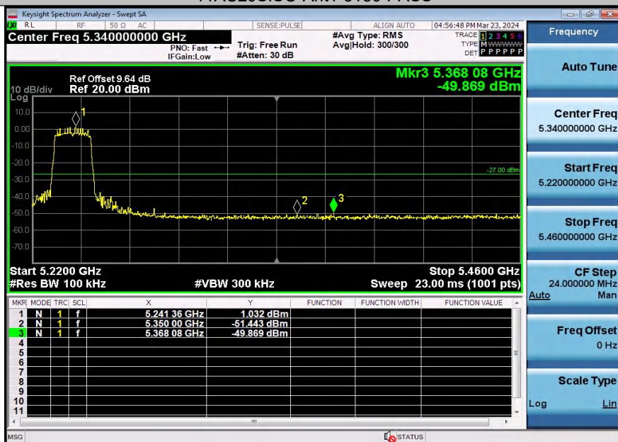
11A20SISO-Ant1-5240-PASS
