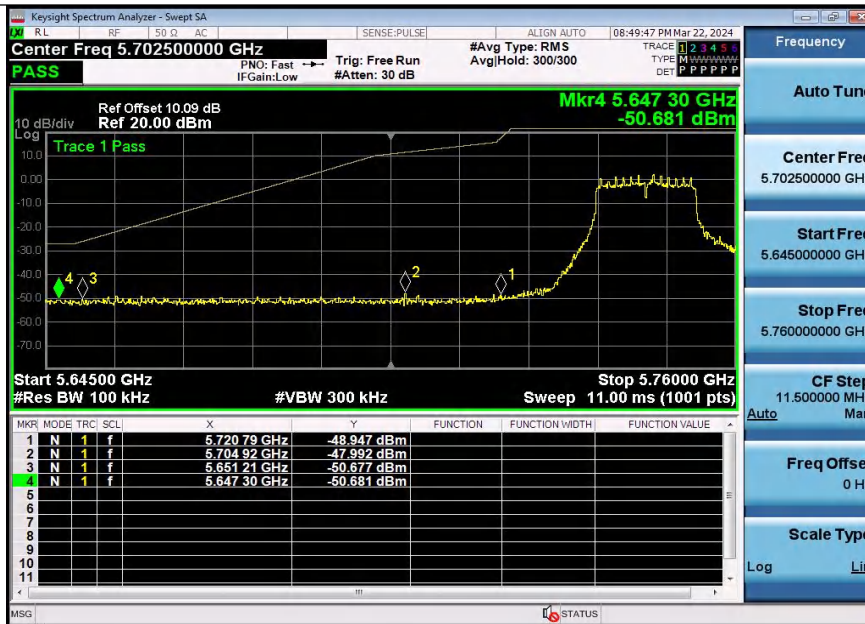
11A-Ant1-5745-PASS
