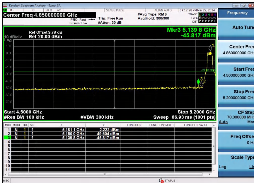
11N20SISO-Ant1-5180-PASS
