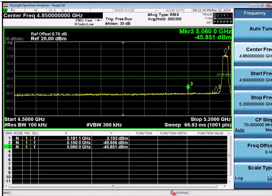
11A-Ant1-5180-PASS
