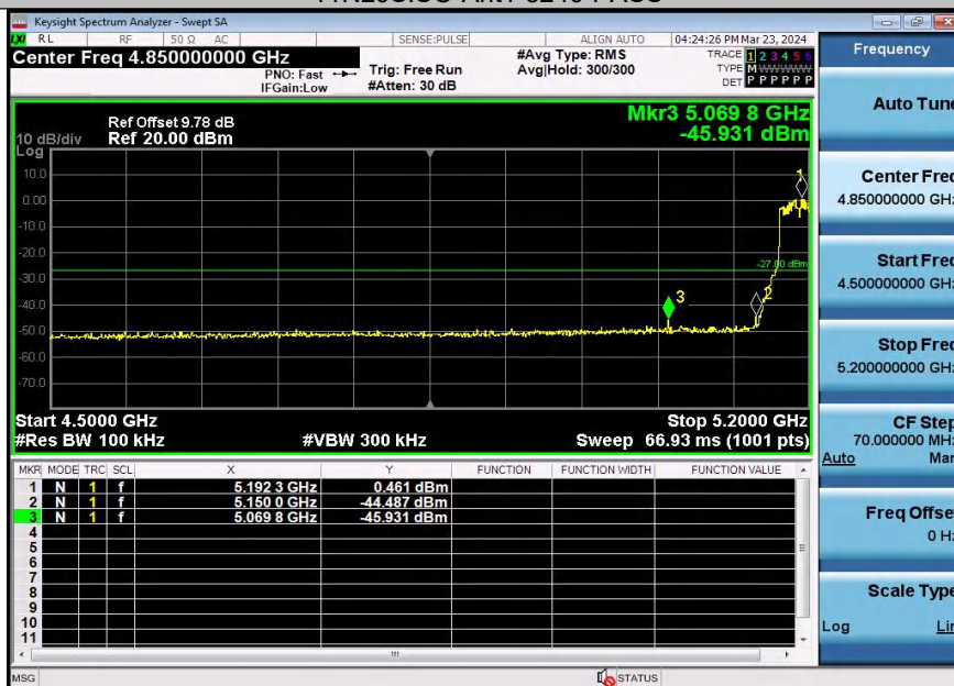
11N40SISO-Ant1-5190-PASS
