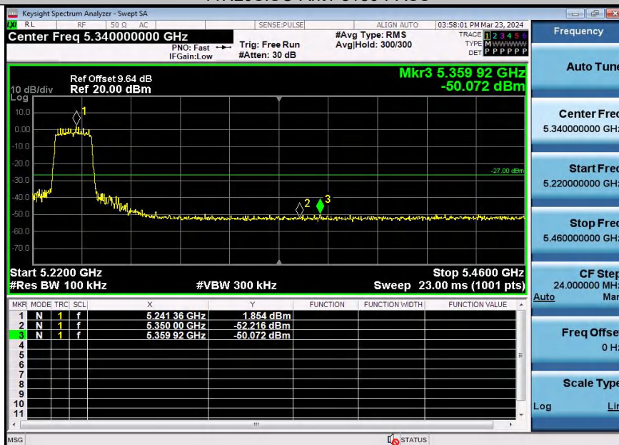
11N20SISO-Ant1-5240-PASS
