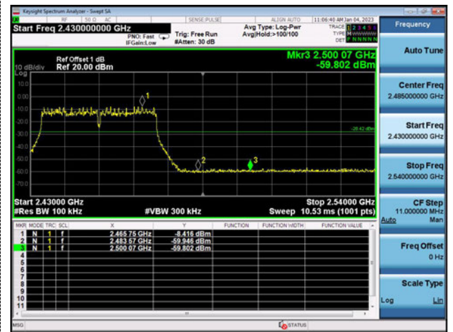
Right bandedge
