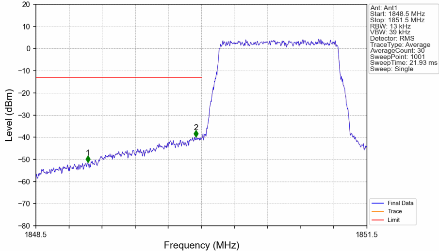
Band2_1.4MHz_16QAM_LCH_1850.7MHz_RB_6_0_NTNV
