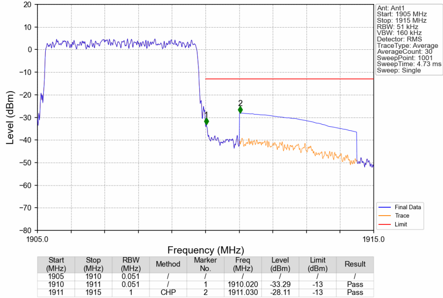
Band2_5MHz_16QAM_HCH_1907.5MHz_RB_25_0_NTNV
