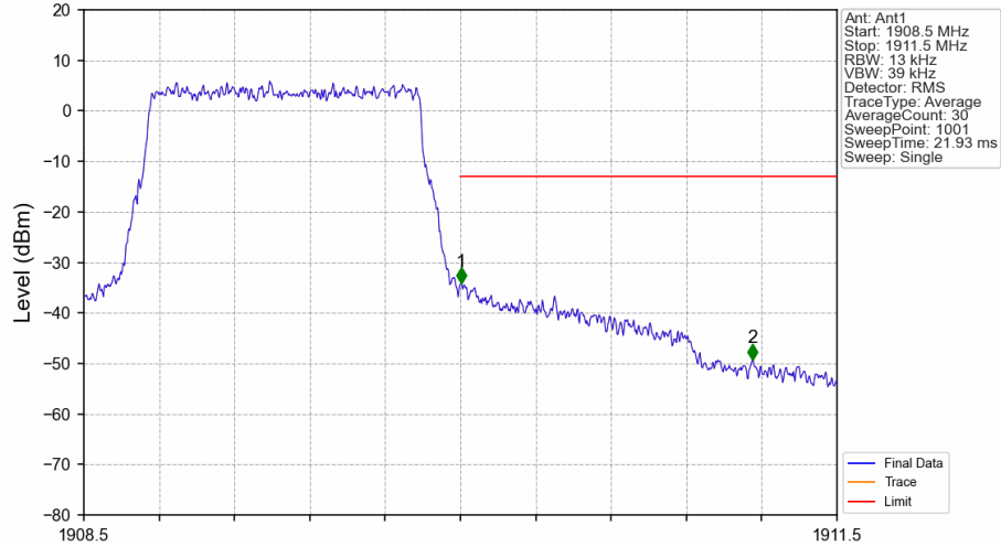
Band2_1.4MHz_QPSK_HCH_1909.3MHz_RB_6_0_NTNV
