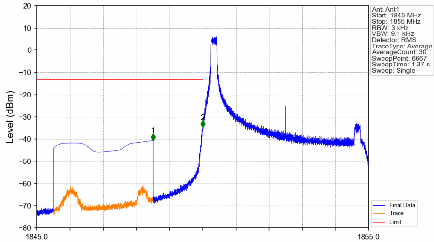
Band2_5MHz_16QAM_LCH_1852.5MHz_RB_1_0_NTNV
