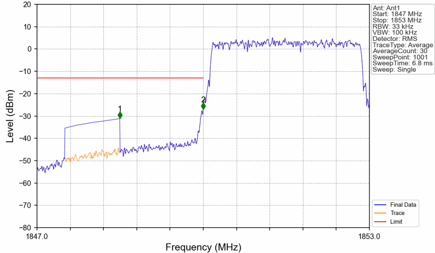
Band2_3MHz_16QAM_LCH_1851.5MHz_RB_15_0_NTNV
