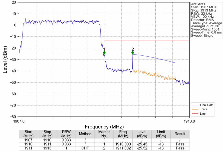
Band2_3MHz_16QAM_HCH_1908.5MHz_RB_15_0_NTNV
