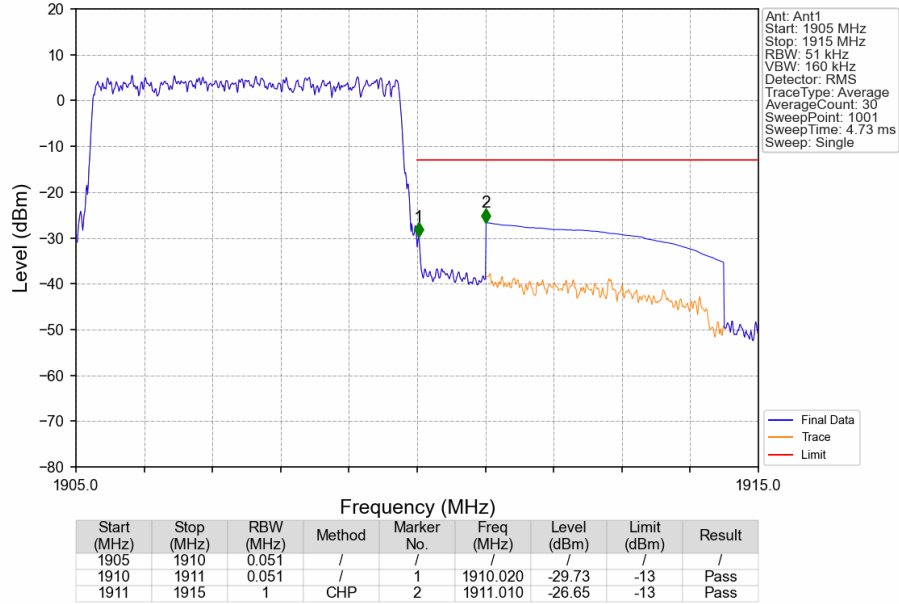
Band2_5MHz_QPSK_HCH_1907.5MHz_RB_25_0_NTNV
