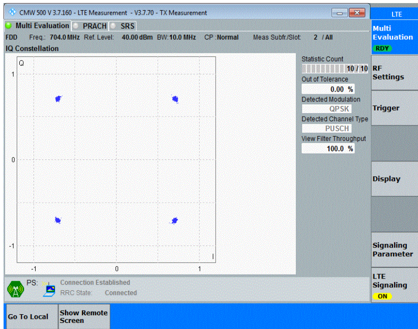
Band12-10MHz-QPSK-23095-50RB#0
