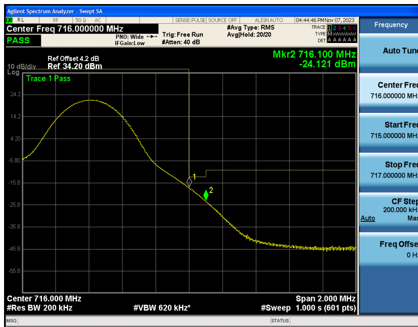
Band12-10MHz-16QAM-23130-50RB#0
