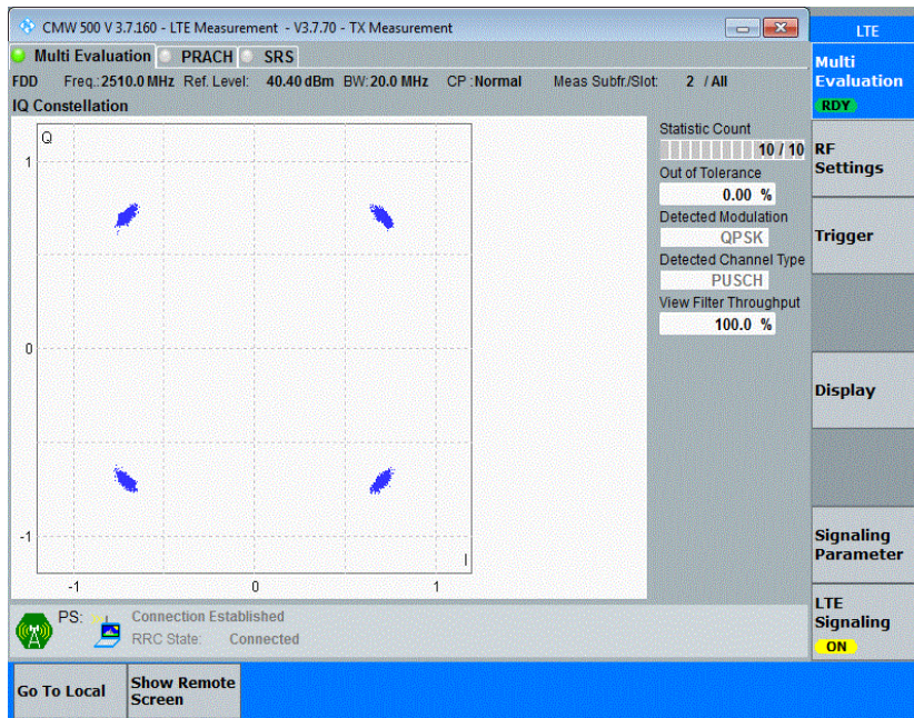
Band7-20MHz-QPSK-21100-100RB#0
