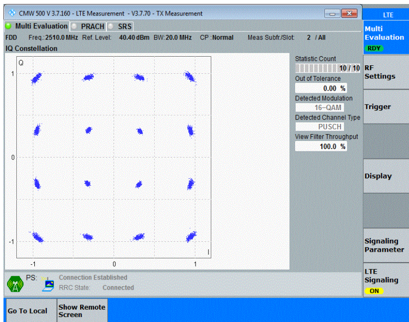
Band7-20MHz-16QAM-21100-100RB#0
