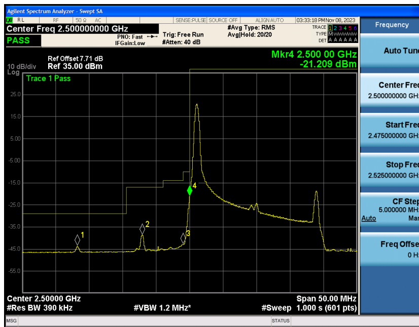
Band7-20MHz-16QAM-20850-1RB#99
