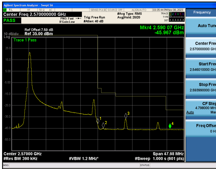
Band7-20MHz-QPSK-21350-1RB#99
