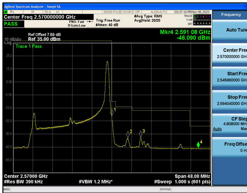
Band7-20MHz-16QAM-21350-100RB#0
