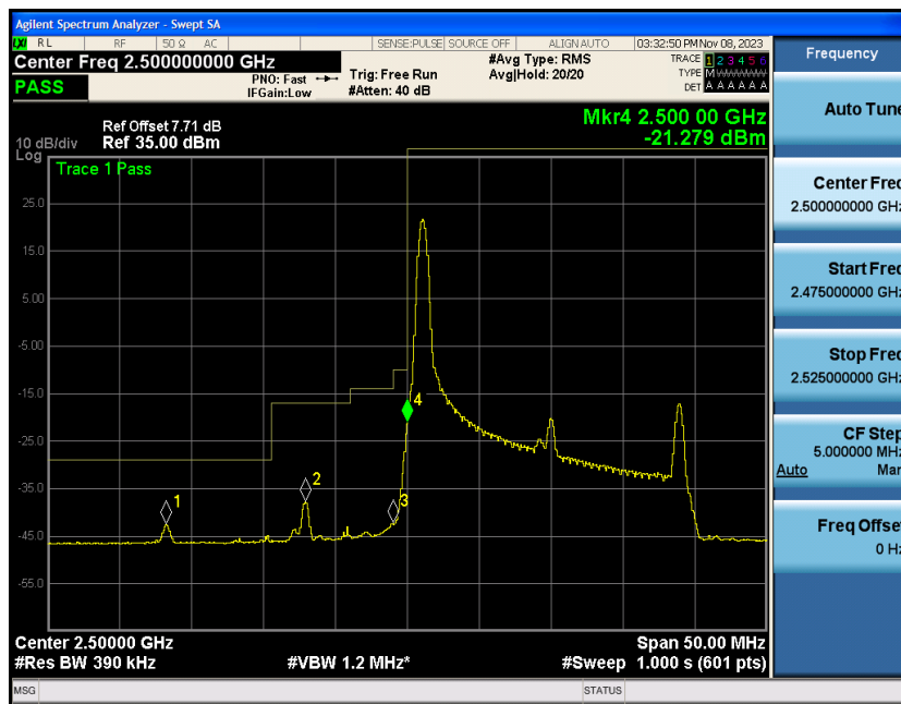
Band7-20MHz-QPSK-20850-1RB#99
