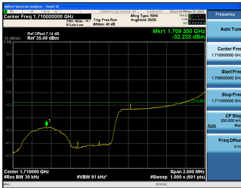
Band4-1.4MHz-16QAM-19957-6RB#0
