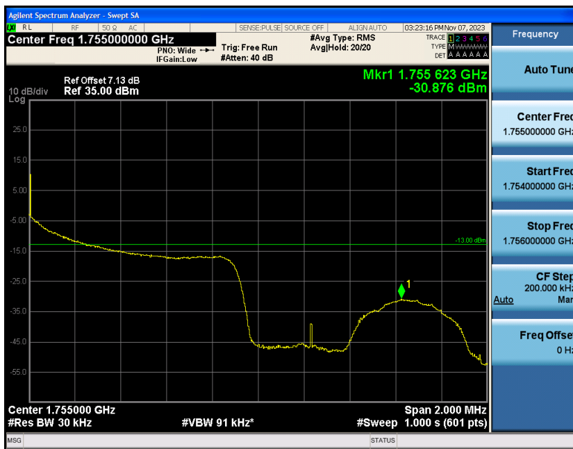
Band4-1.4MHz-QPSK-20393-1RB#5
