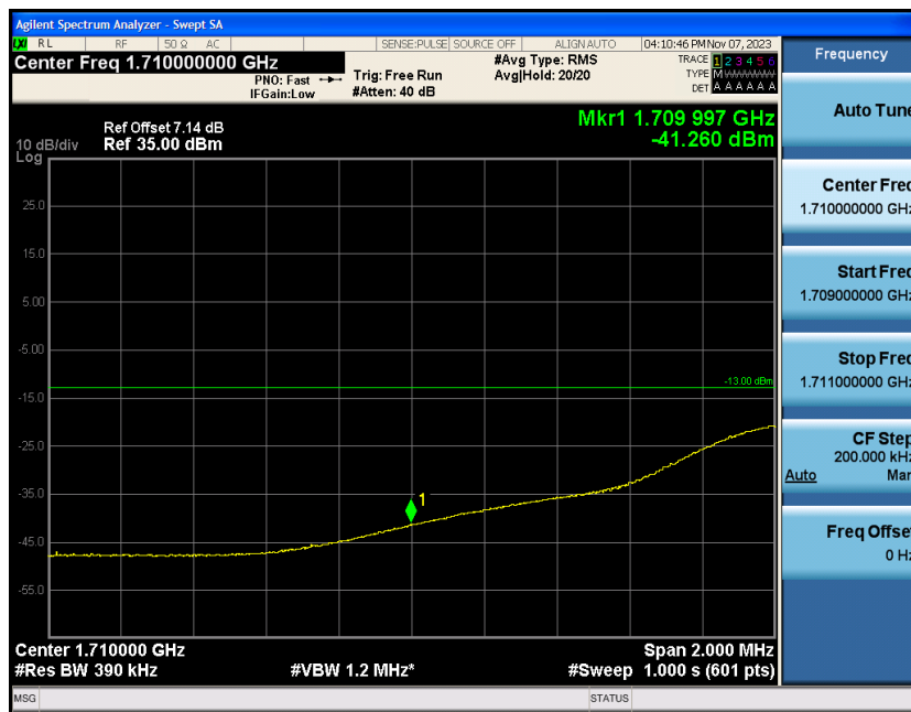
Band4-20MHz-16QAM-20050-100RB#0
