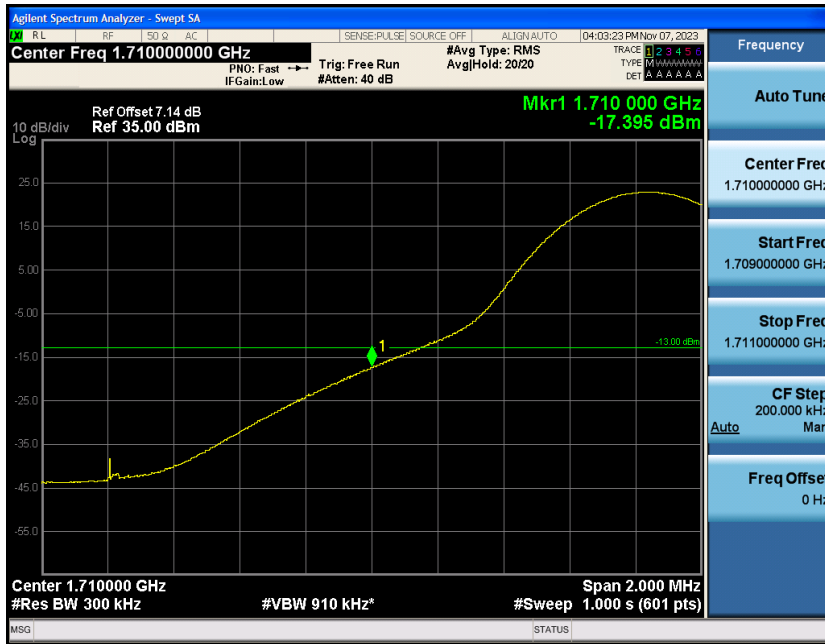
Band4-15MHz-QPSK-20025-1RB#74
