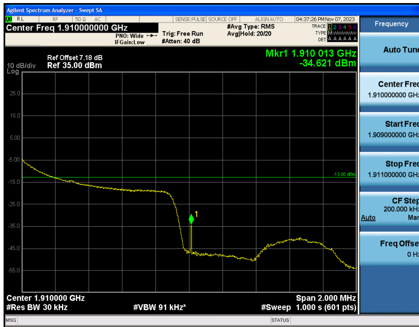
Band2-1.4MHz-16QAM-19193-1RB#5
