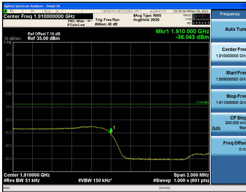
Band2-3MHz-16QAM-19185-1RB#14
