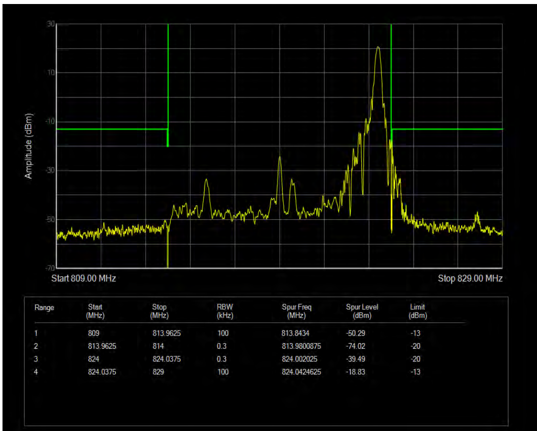
Band26a 16QAM BW=10MHz Channel=26740 RB Size=1 Position=#Max
