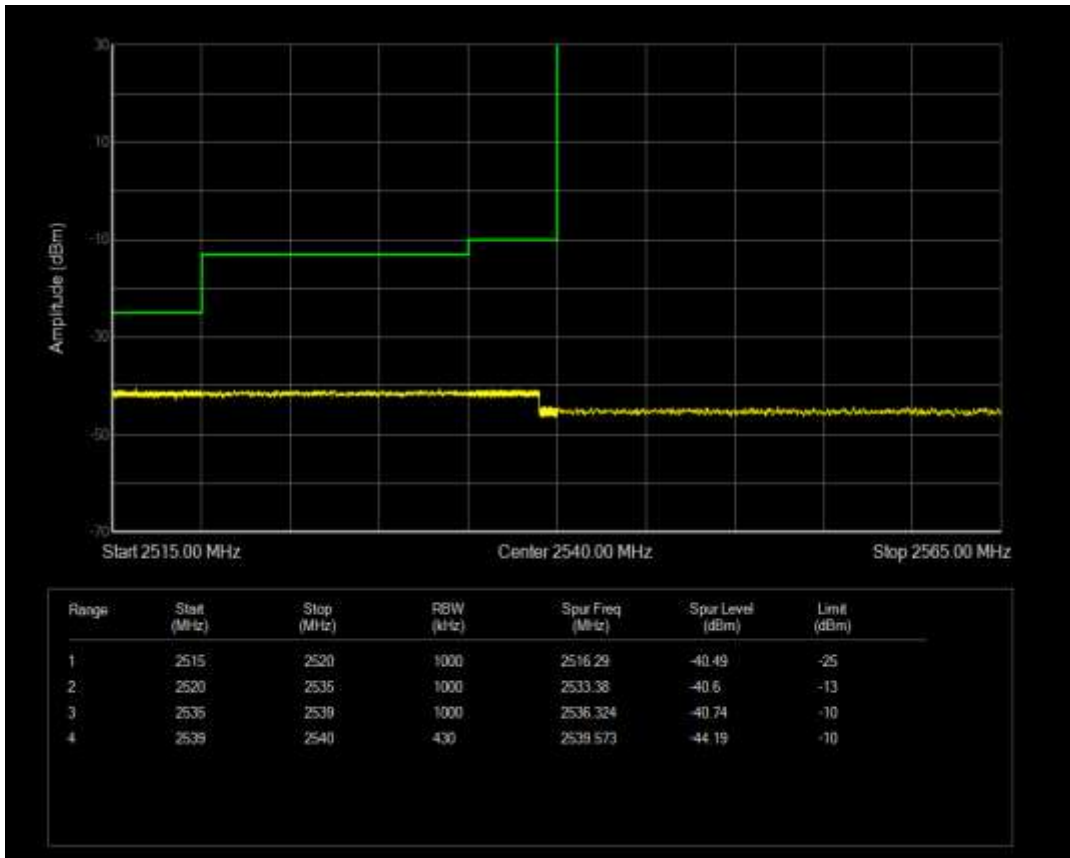
Band41 16QAM BW=20MHz Channel=40190 RB Size=1 Position=#0
