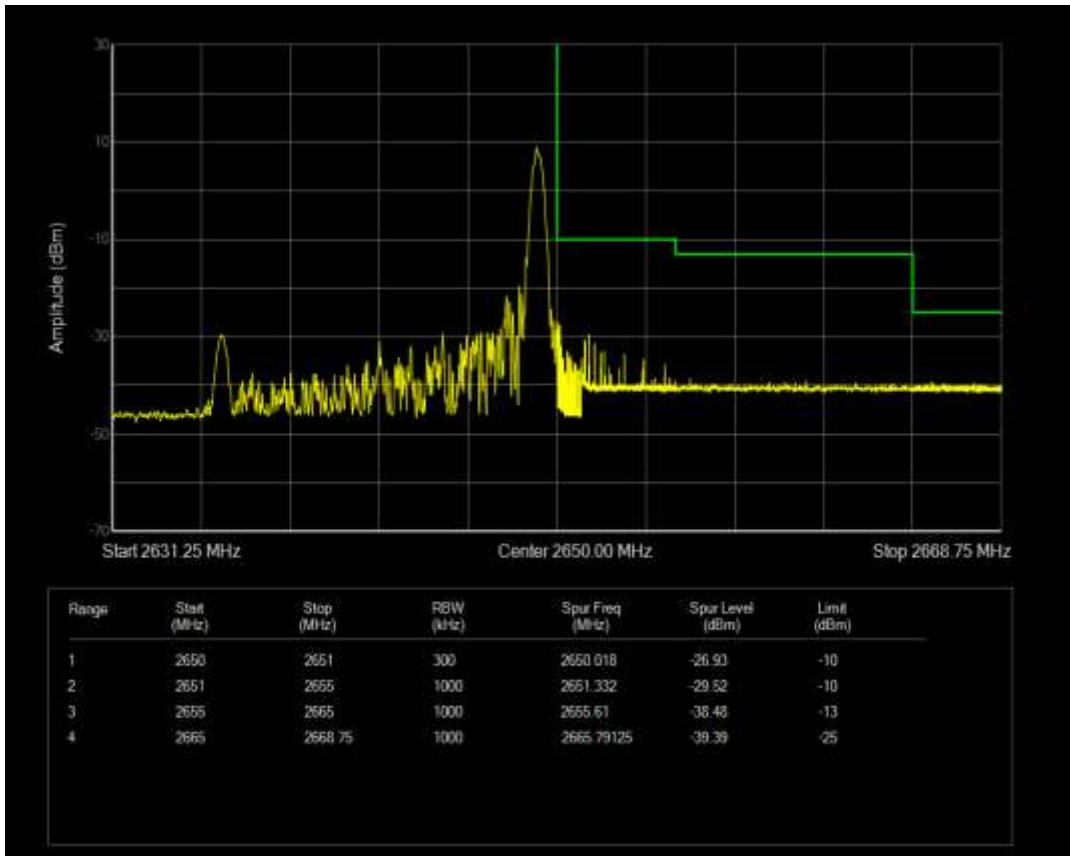
Band41 16QAM BW=15MHz Channel=41115 RB Size=75 Position=#0
